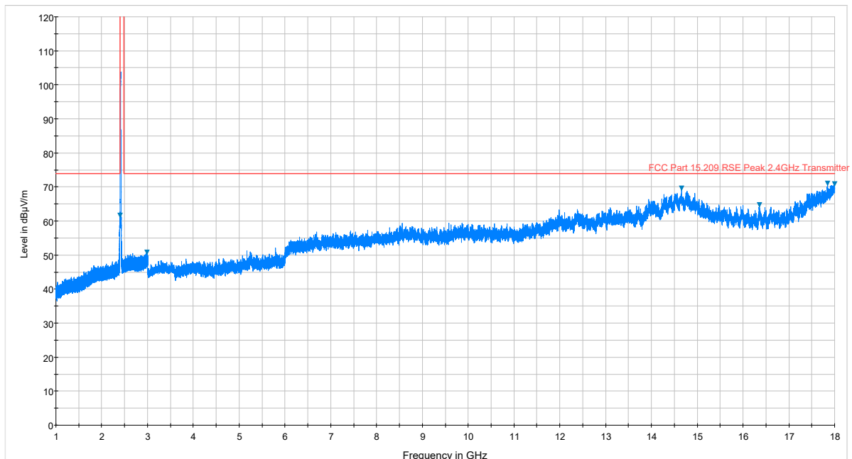
Plot 7-32. Radiated Spurious Plot above 1GHz (802.11b – Ch. 1, Ant. Pol. V)
