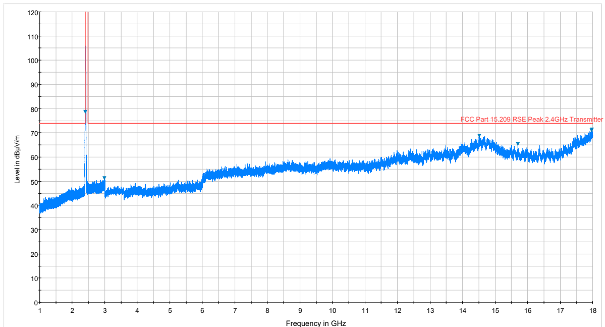
Plot 7-31. Radiated Spurious Plot above 1GHz (802.11b – Ch. 1, Ant. Pol. H)
