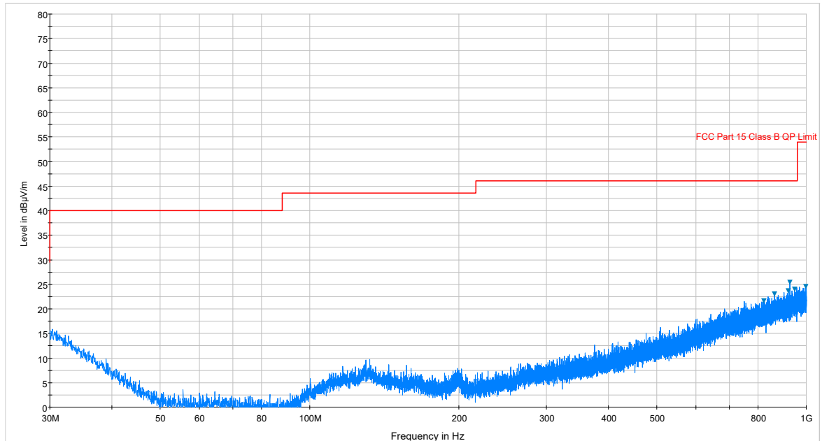
Plot 7-46. Radiated Spurious Plot below 1GHz (Pol. H)
