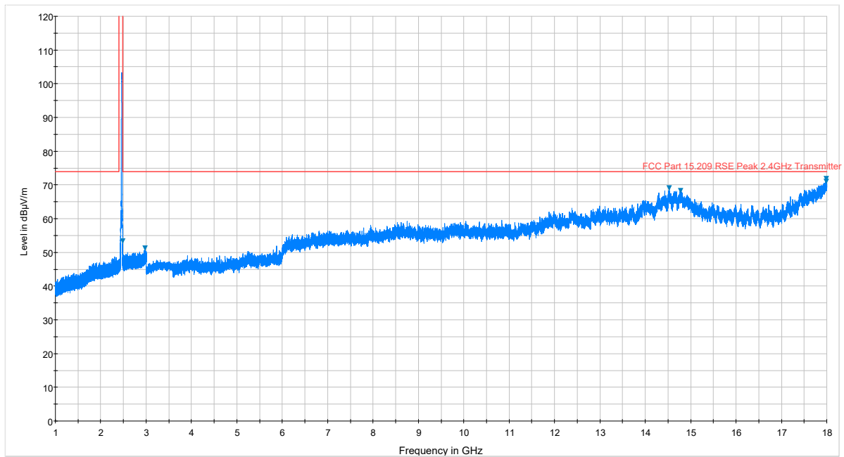
Plot 7-36. Radiated Spurious Plot above 1GHz (802.11b – Ch. 11, Ant. Pol. V)
