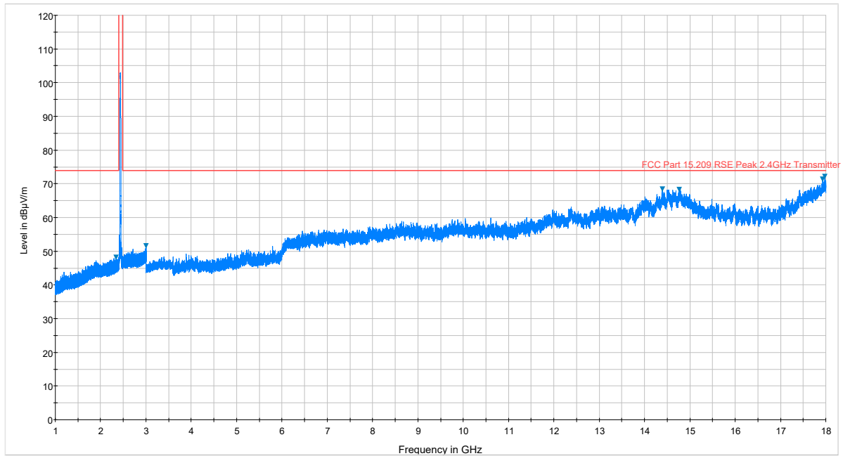
Plot 7-33. Radiated Spurious Plot above 1GHz (802.11b – Ch. 6, Ant. Pol. H)
