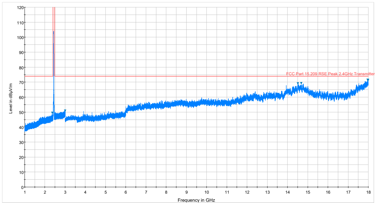
Plot 7-34. Radiated Spurious Plot above 1GHz (802.11b – Ch. 6, Ant. Pol. V)
