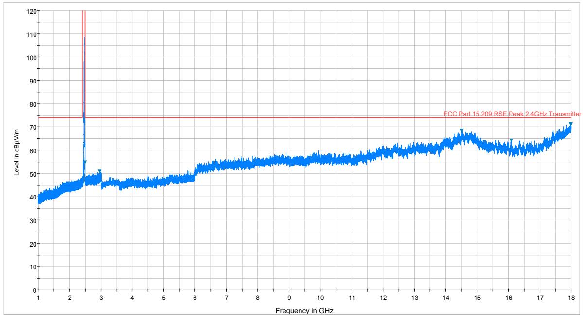
Plot 7-35. Radiated Spurious Plot above 1GHz (802.11b – Ch. 11, Ant. Pol. H)
