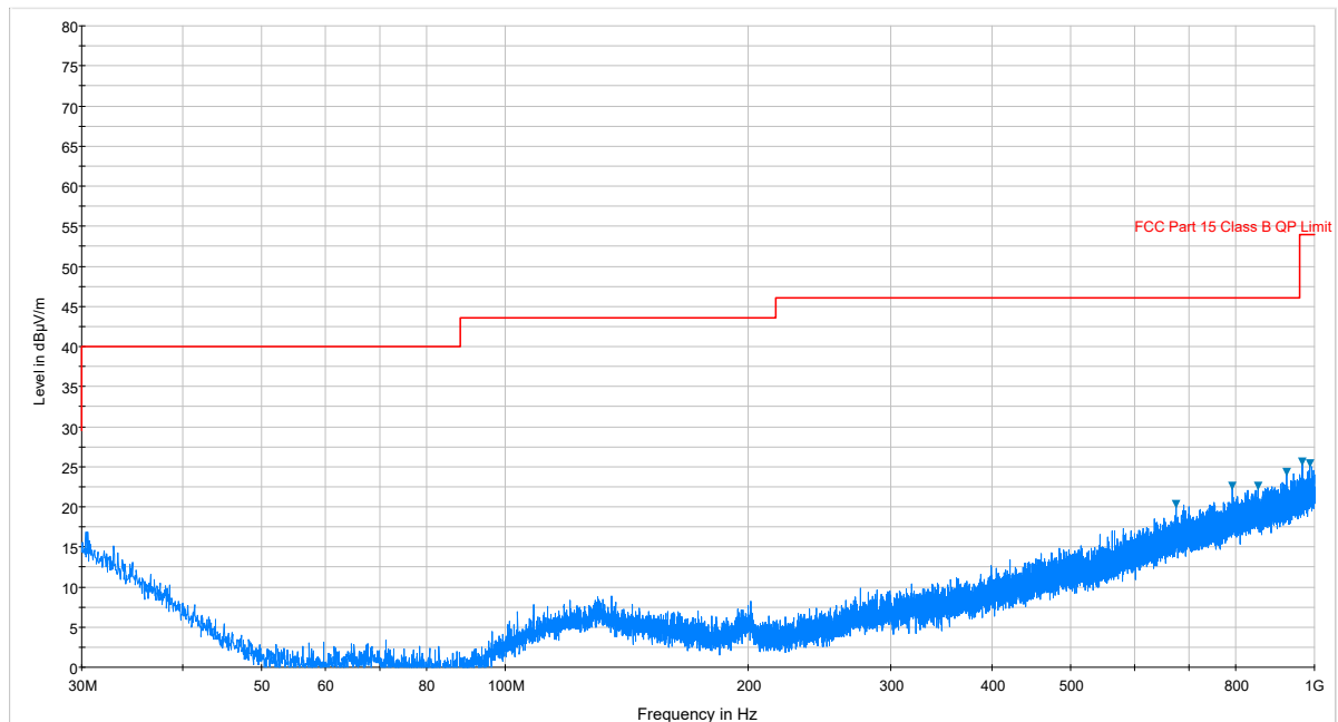
Plot 7-47. Radiated Spurious Plot below 1GHz (Pol. V)
