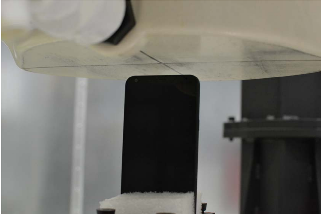
SAR Test Setup Photo 7: Top at 1.0 cm
