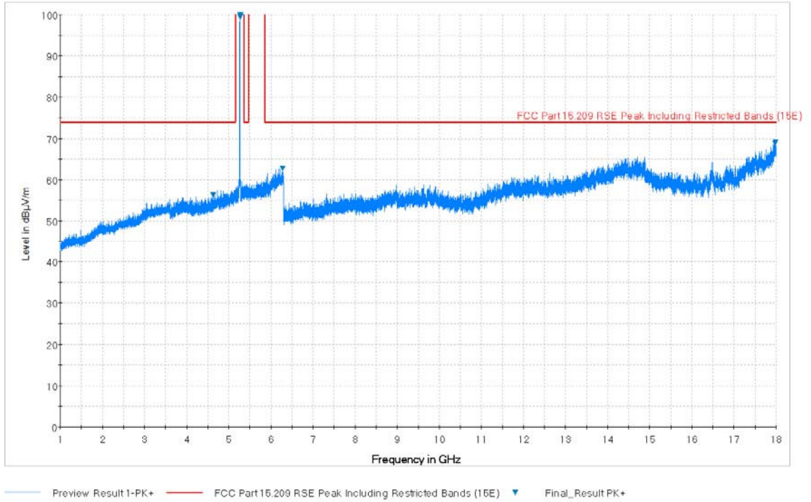
Plot 7-77. Radiated Spurious Plot above 1GHz (802.11a – U2A Ch. 56, Ant. Pol. H)
