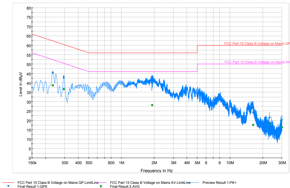
Plot 6-18. Line Conducted Plot with Bluetooth LE (L1)
