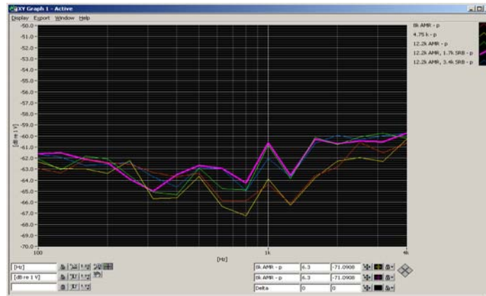
Figure 6-1 UMTS Audio Band Magnetic Noise
