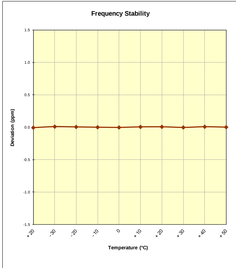
Figure 6-9. Frequency Stability Graph (AWS WCDMA Mode – Ch. 1413)
