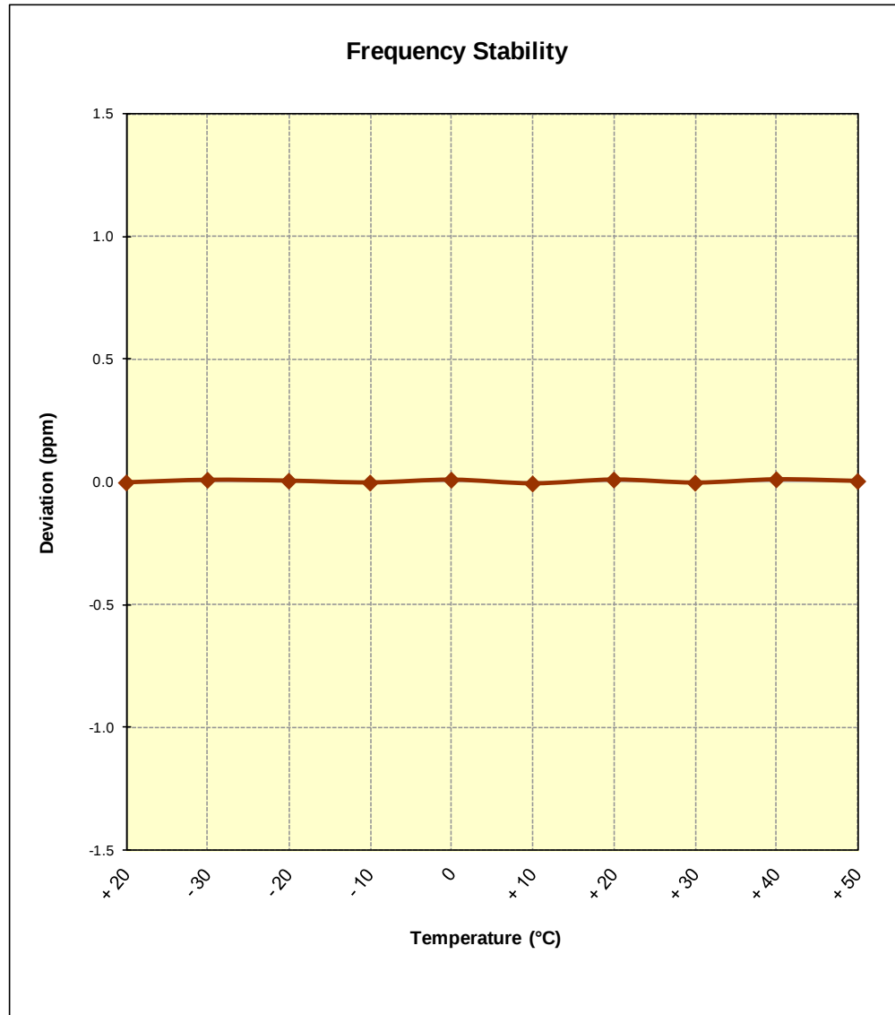
Figure 6-11. Frequency Stability Graph (PCS WCDMA Mode – Ch. 9400)
