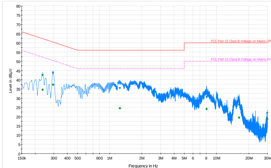
Plot 6-44. Line-Conducted Test Plot (L1)
