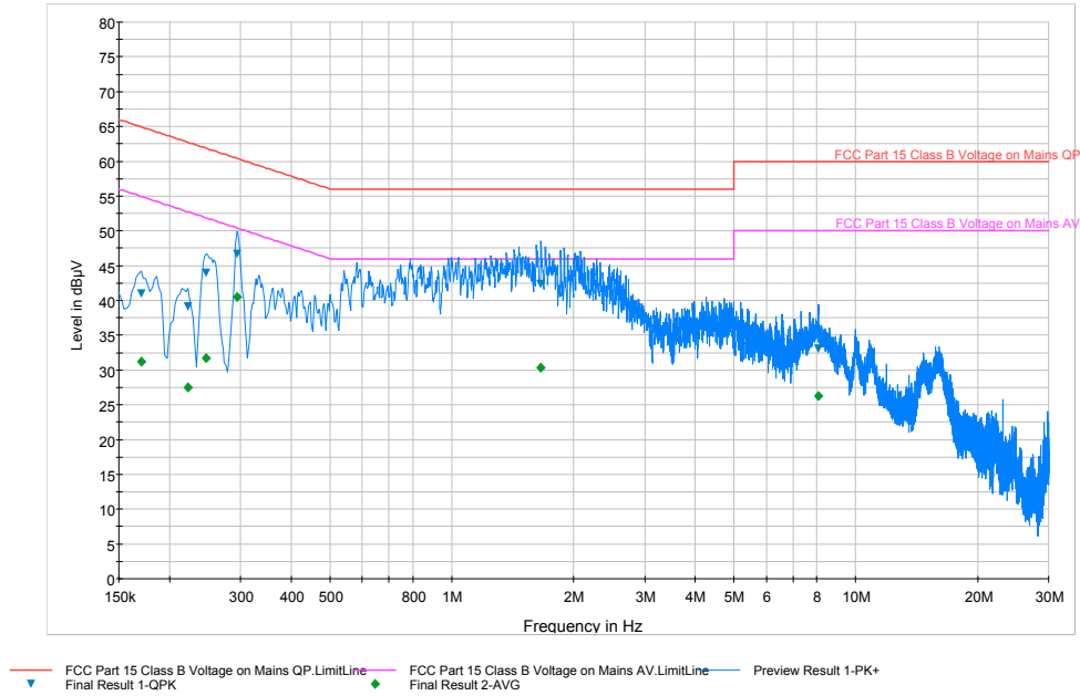
Plot 6-35. Line Conducted Plot with 802.11b (L1)
