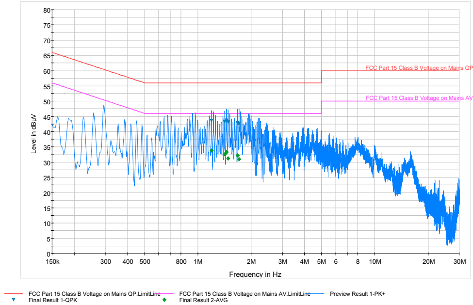
Plot 6-36. Line Conducted Plot with 802.11b (N)
