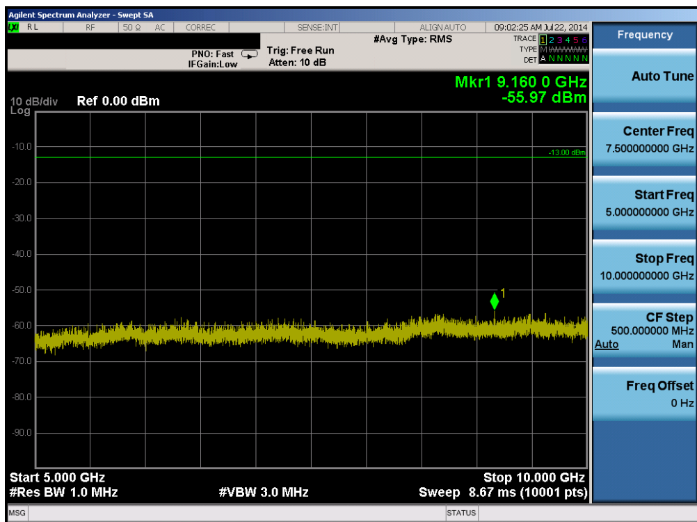
Plot 6-30. Conducted Spurious Plot (Band 17 – 5.0MHz QPSK – RB Size 1, RB Offset 0 – Low Channel)
