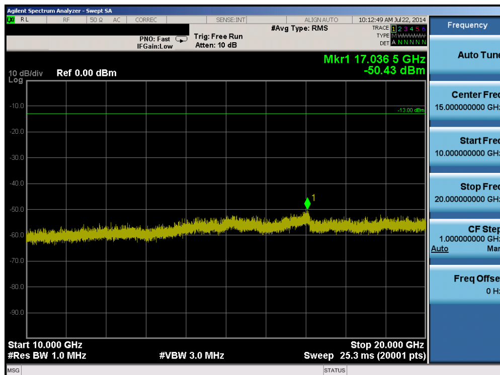
Plot 6-44. Conducted Spurious Plot (Band 2 – 15.0MHz QPSK – RB Size 1, RB Offset 0 – Mid Channel)
