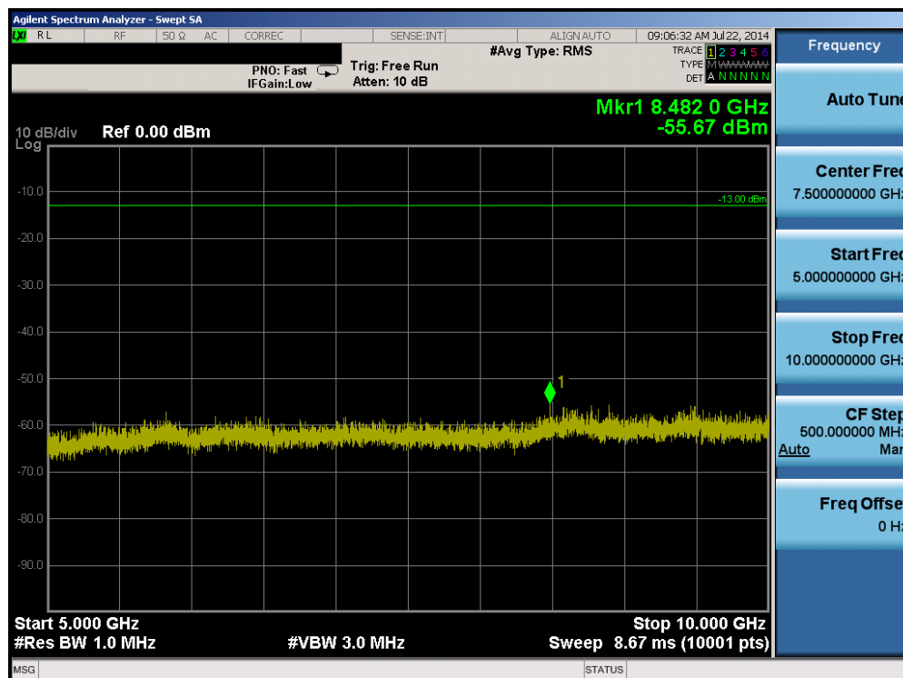
Plot 6-34. Conducted Spurious Plot (Band 17 – 5.0MHz QPSK – RB Size 1, RB Offset 0 – High Channel)
