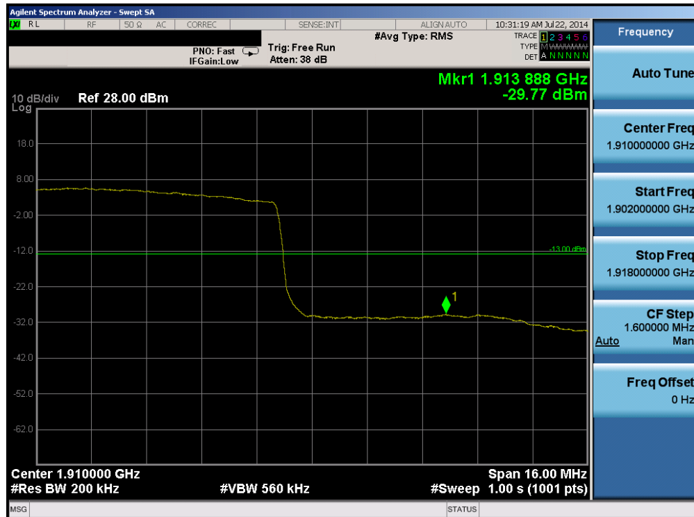
Plot 6-90. Upper Band Edge Plot (Band 2 – 20.0MHz QPSK – RB Size 100)
