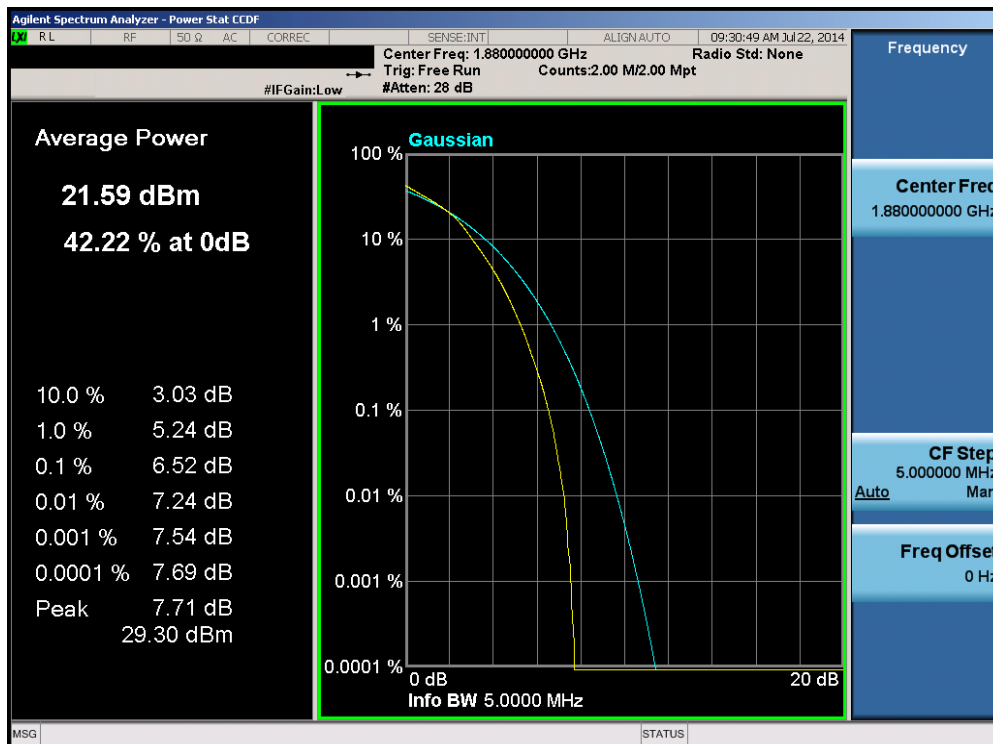
Plot 6-105. PAR Plot (Band 2 – 5.0MHz 16-QAM – RB Size 25)
