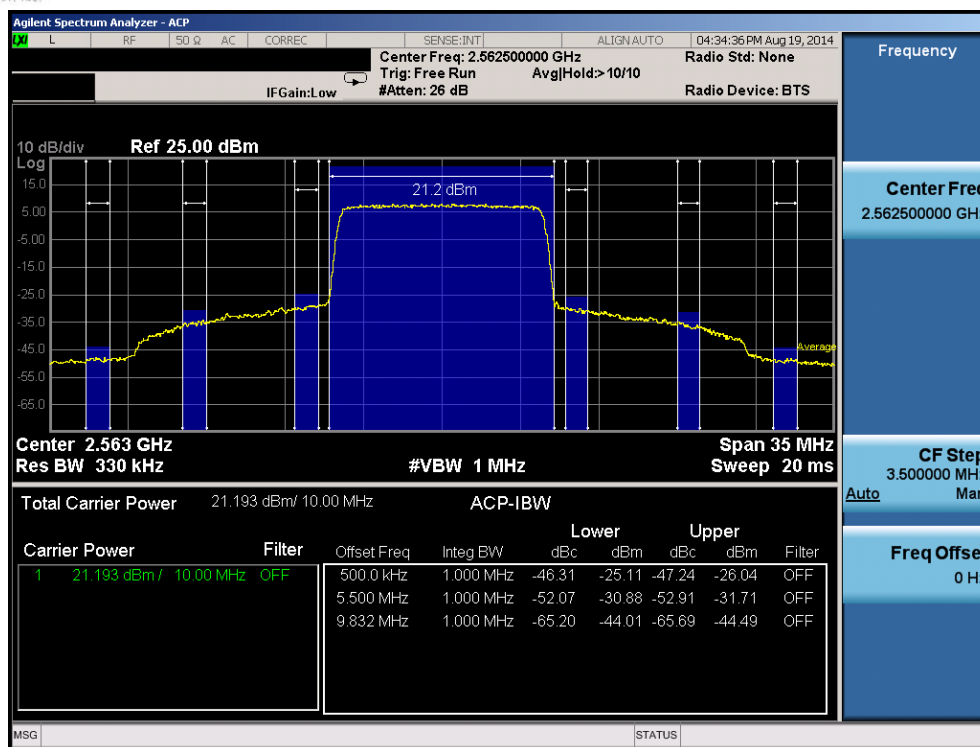
Plot 6-97. Upper ACP Plot (Band 7 – 10.0MHz QPSK – RB Size 50)
