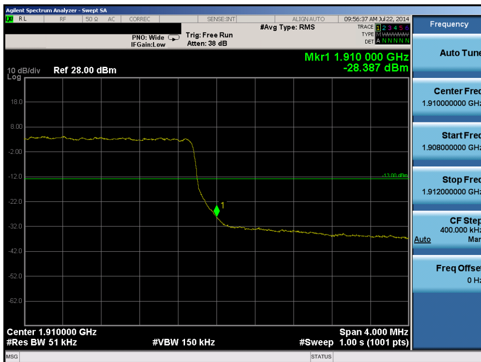
Plot 6-78. Upper Band Edge Plot (Band 2 – 5.0MHz QPSK – RB Size 25)
