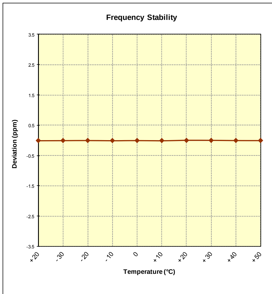
Figure 6-10. Frequency Stability Graph (Band 7)
