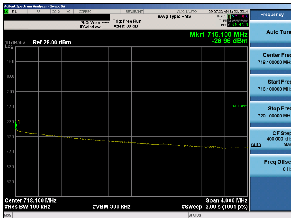
Plot 6-56. Upper Extended Band Edge Plot (Band 17 – 5.0MHz QPSK – RB Size 25)
