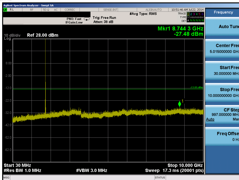
Plot 6-39. Conducted Spurious Plot (Band 4 – 10.0MHz QPSK – RB Size 1, RB Offset 0 – High Channel)
