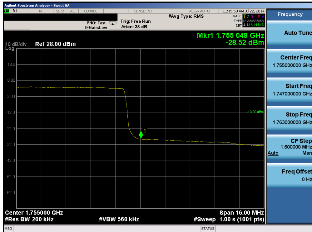
Plot 6-74. Upper Band Edge Plot (Band 4 – 20.0MHz QPSK – RB Size 100)
