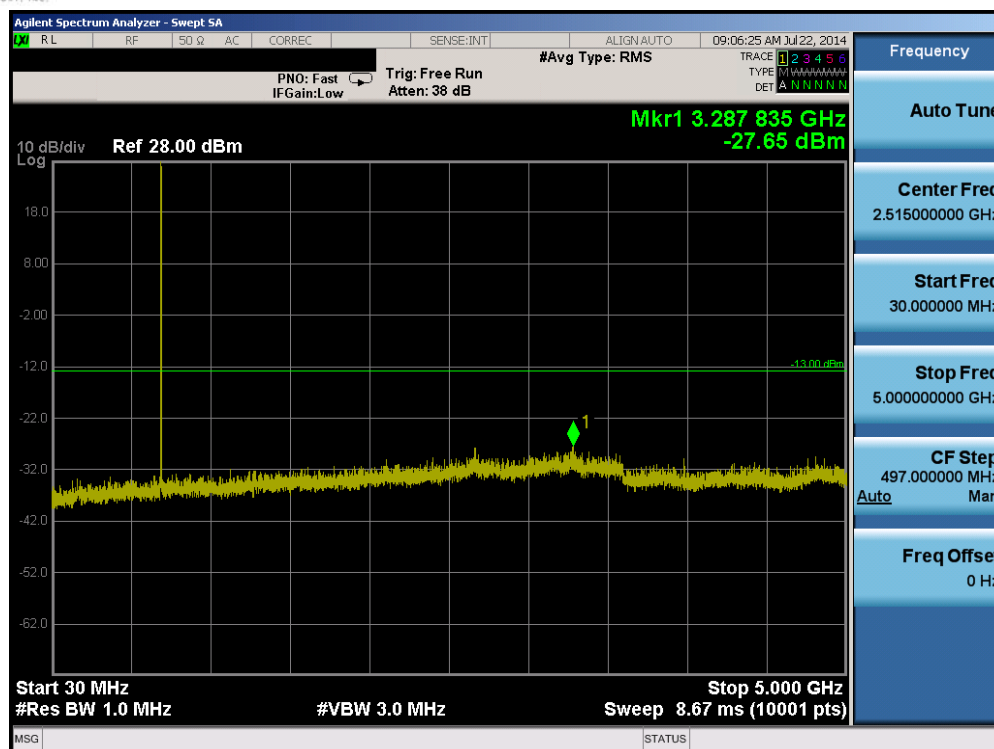
Plot 6-33. Conducted Spurious Plot (Band 17 – 5.0MHz QPSK – RB Size 1, RB Offset 0 – High Channel)
