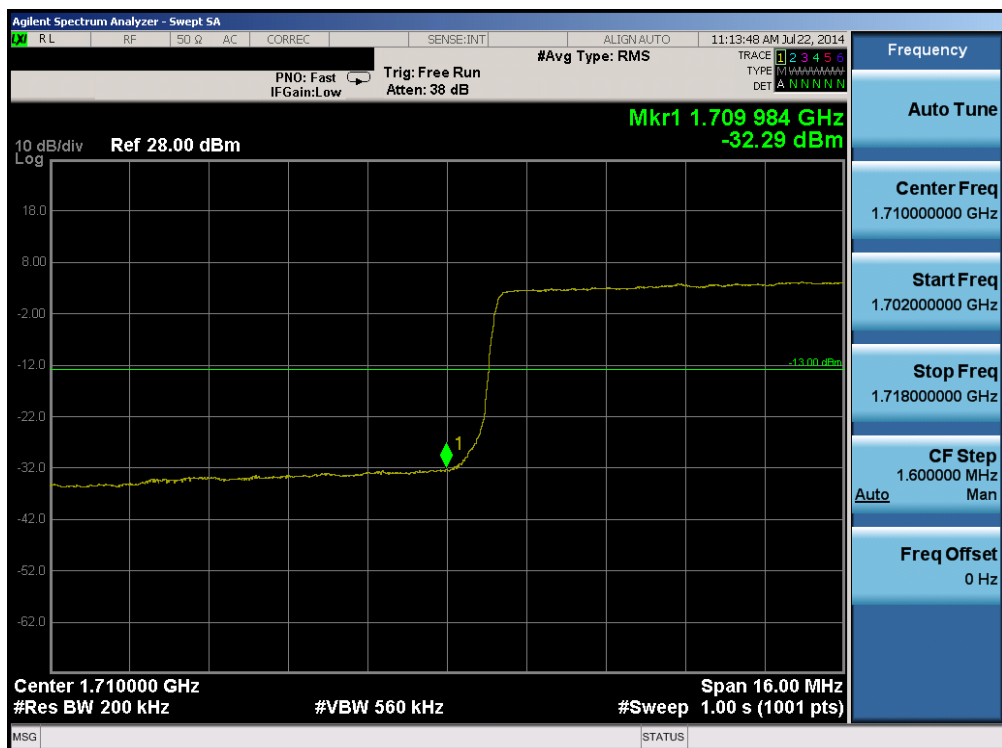
Plot 6-72. Lower Band Edge Plot (Band 4 – 20.0MHz QPSK – RB Size 100)
