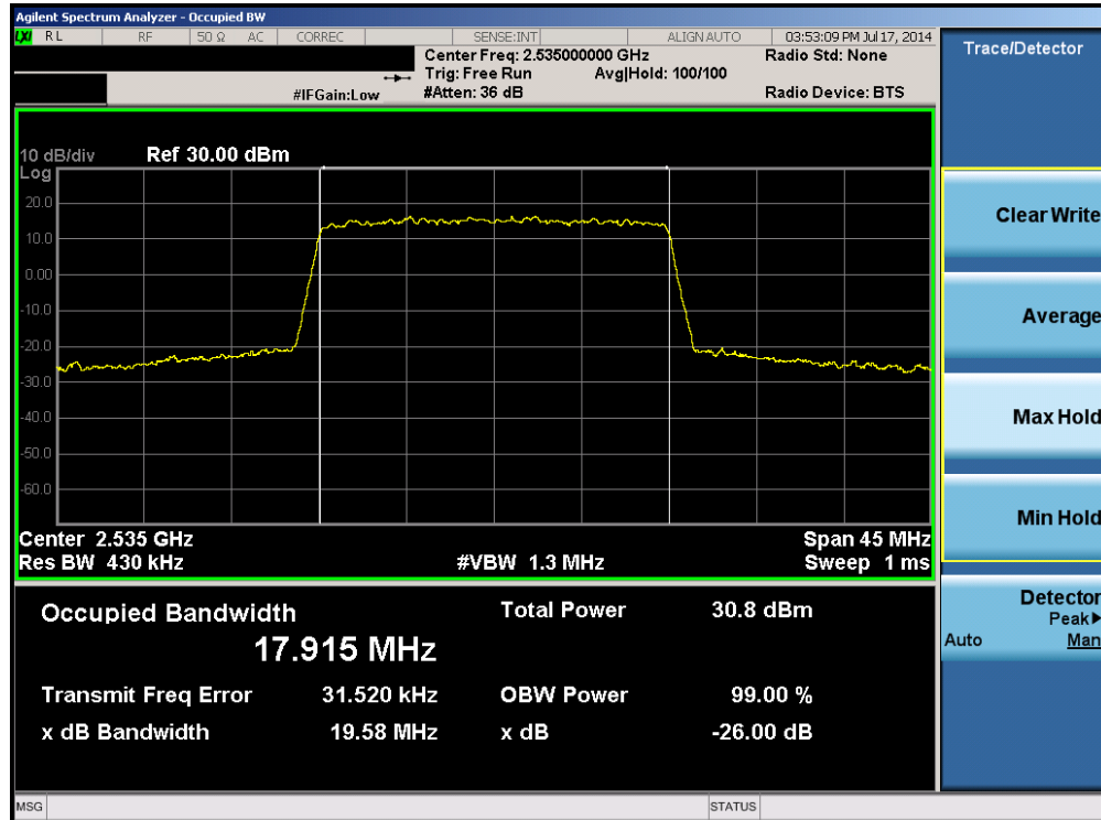
Plot 6-27. Occupied Bandwidth Plot (Band 7 – 20.0MHz QPSK – RB Size 100)
