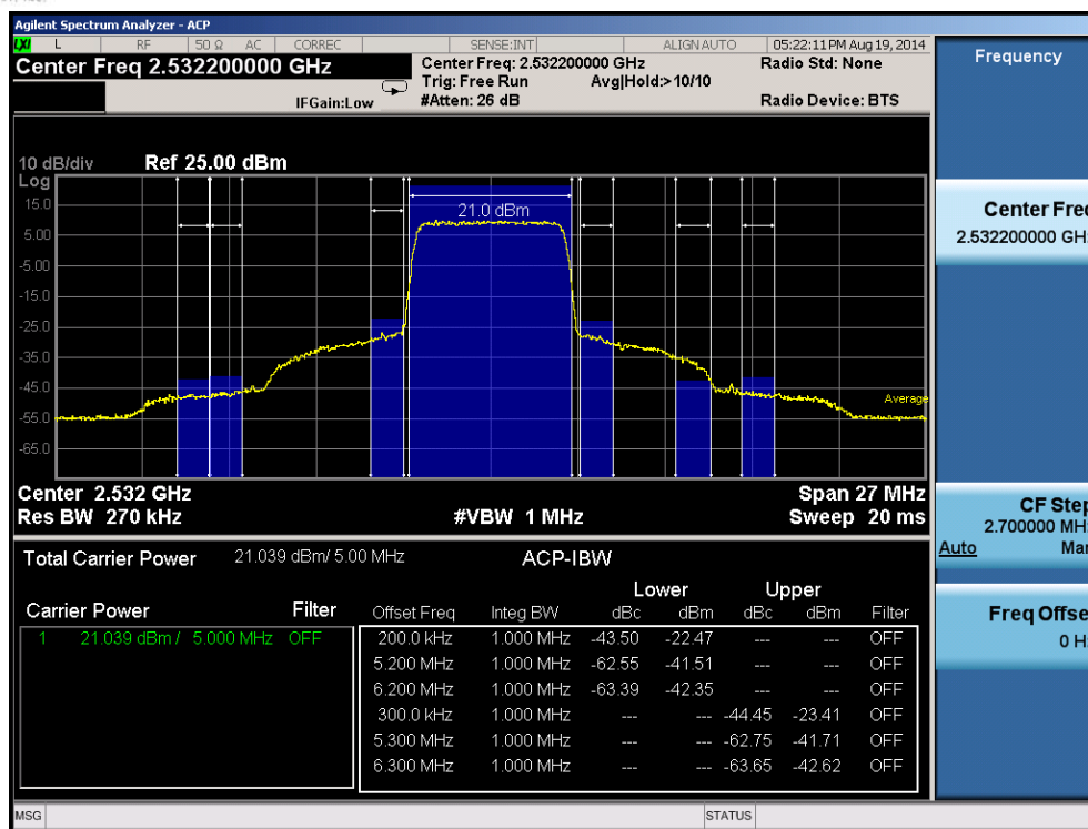
Plot 6-93. Mid ACP Plot (Band 7 – 5.0MHz QPSK – RB Size 25)
