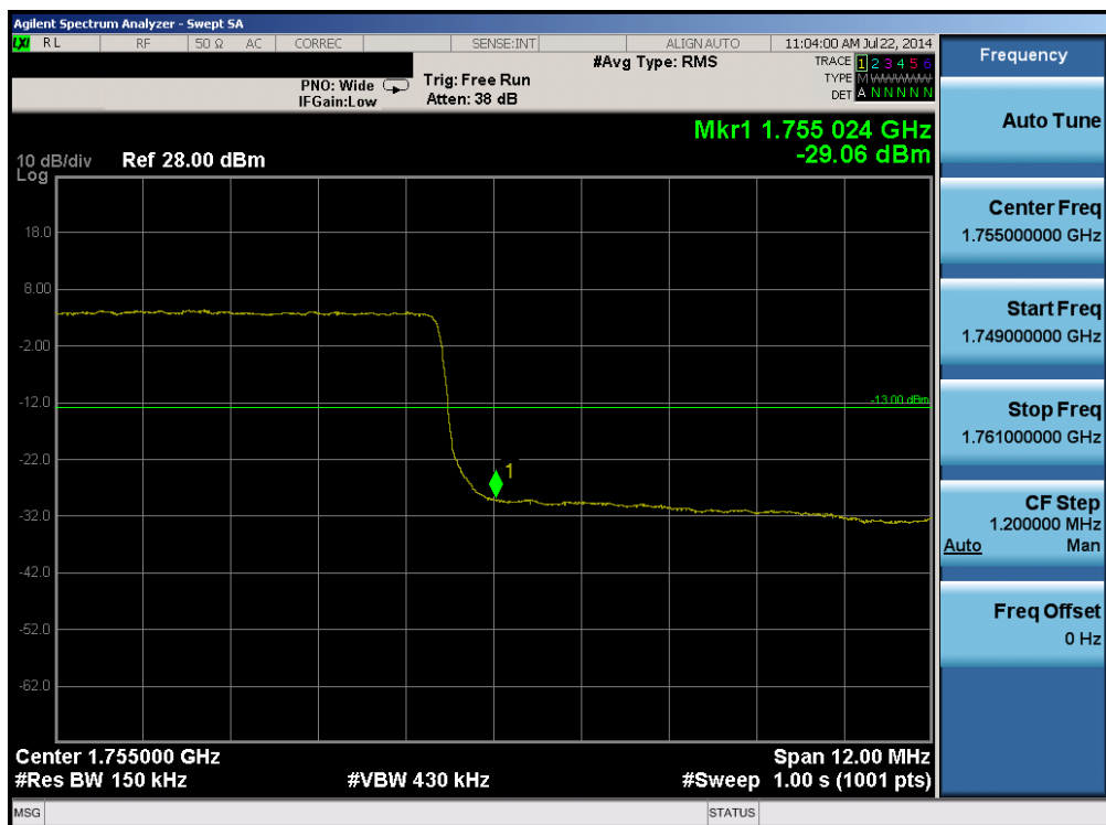
Plot 6-70. Upper Band Edge Plot (Band 4 – 15.0MHz QPSK – RB Size 75)
