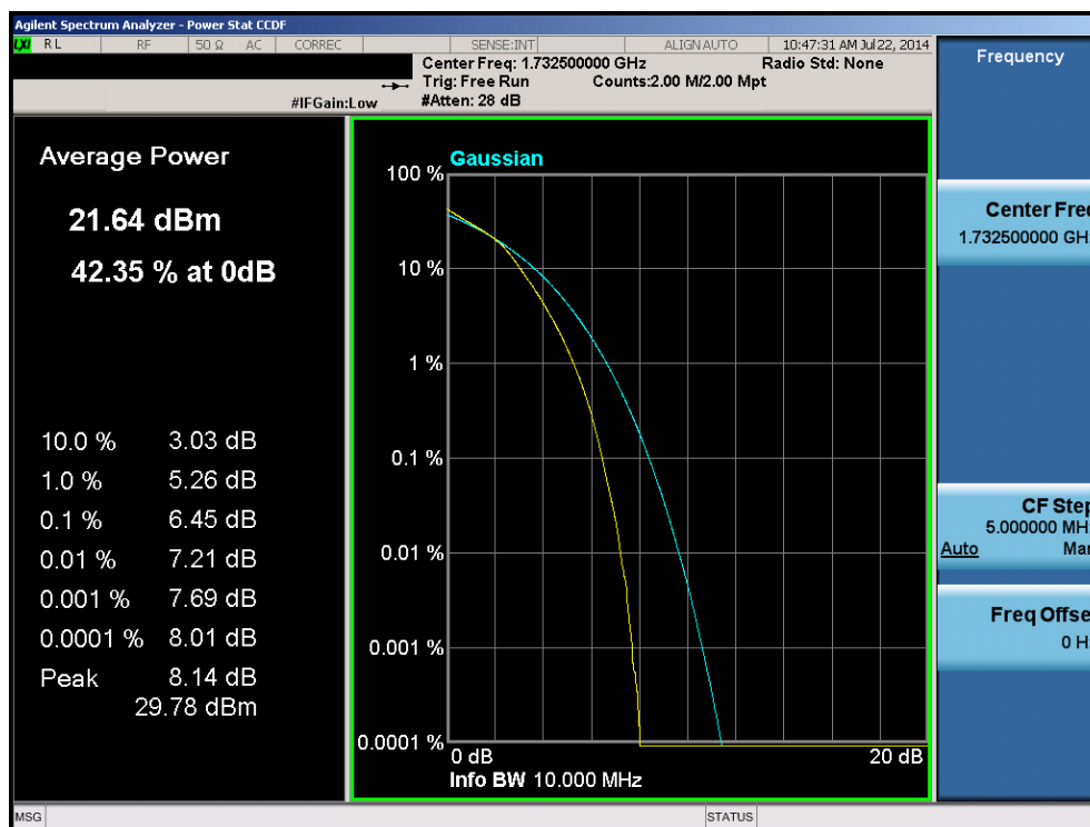
Plot 6-123. PAR Plot (Band 4 – 10.0MHz – 16-QAM – RB Size 50)
