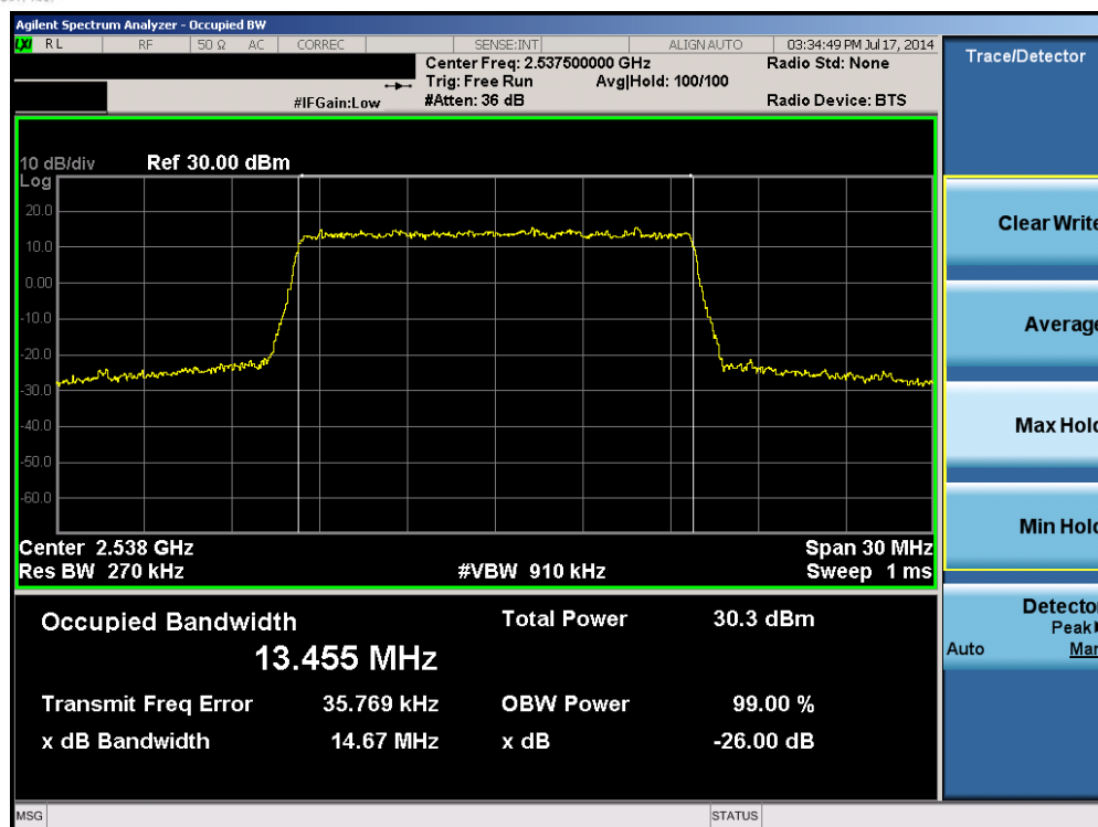
Plot 6-25. Occupied Bandwidth Plot (Band 7 – 15.0MHz QPSK – RB Size 75)
