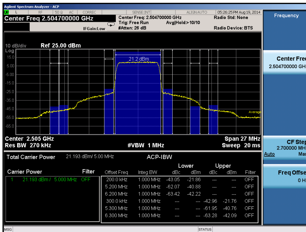
Plot 6-92. Lower ACP Plot (Band 7 – 5.0MHz QPSK – RB Size 25)
