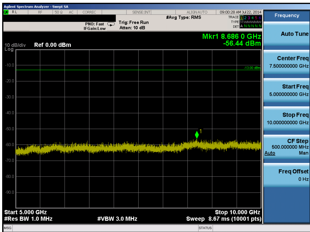
Plot 6-32. Conducted Spurious Plot (Band 17 – 5.0MHz QPSK – RB Size 1, RB Offset 0 – Mid Channel)
