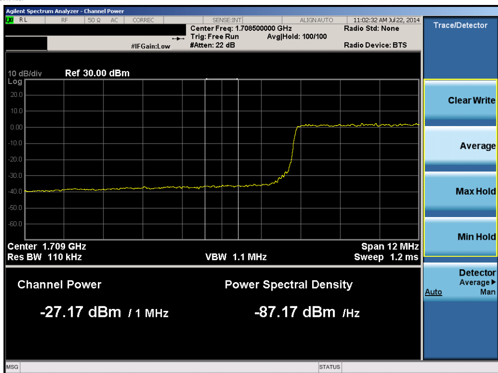
Plot 6-69. Lower Extended Band Edge Plot (Band 4 – 15.0MHz QPSK – RB Size 75)
