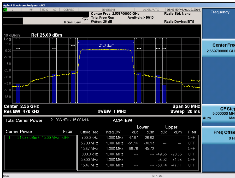
Plot 6-100. Upper ACP Plot (Band 7 – 15.0MHz QPSK – RB Size 75)
