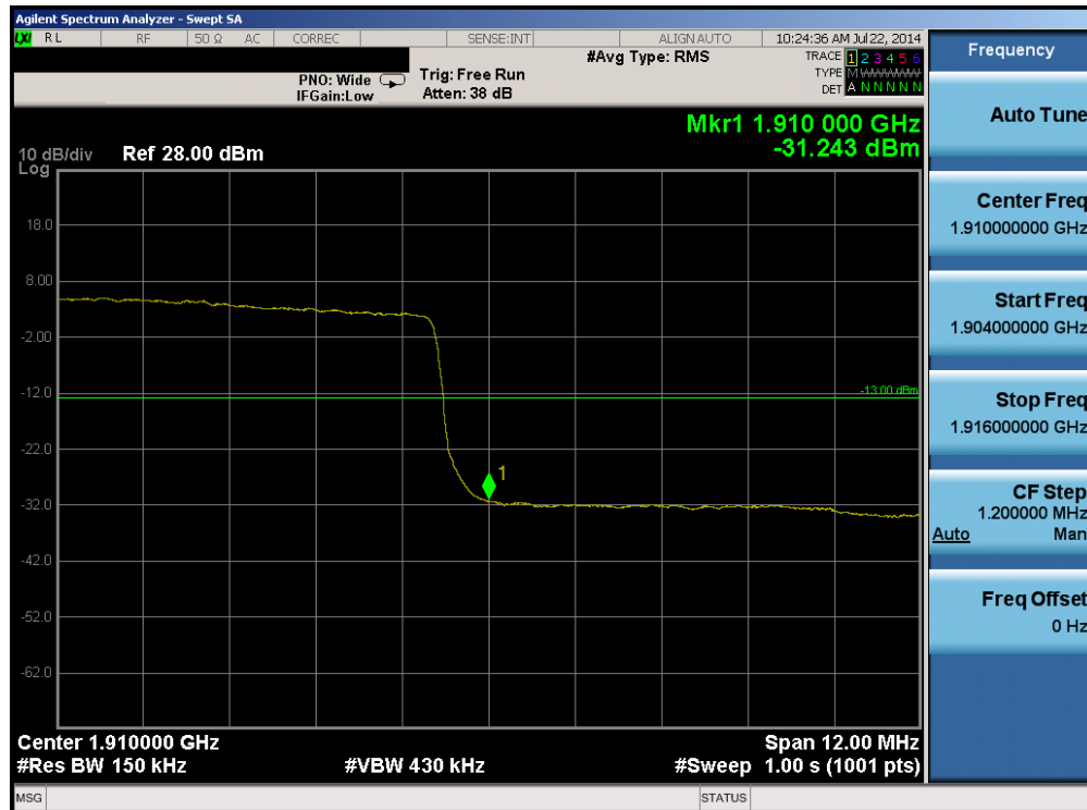
Plot 6-86. Upper Band Edge Plot (Band 2 – 15.0MHz QPSK – RB Size 75)
