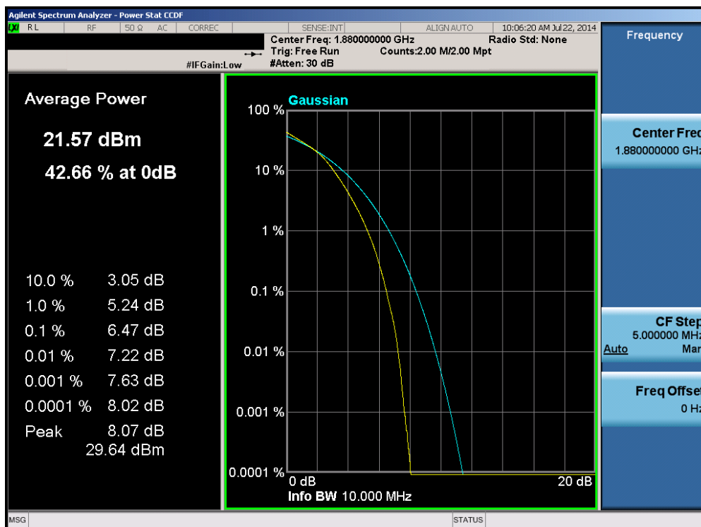
Plot 6-107. PAR Plot (Band 2 – 10.0MHz 16-QAM – RB Size 50)
