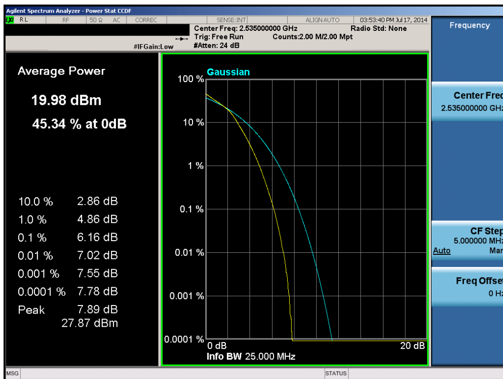
Plot 6-119. PAR Plot (Band 7 – 20.0MHz 16-QAM – RB Size 100)
