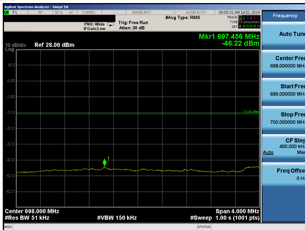
Plot 6-53. Lower Band Edge Plot (Band 17 – 5.0MHz QPSK – RB Size 25)
