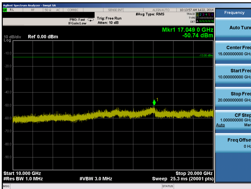
Plot 6-42. Conducted Spurious Plot (Band 2 – 15.0MHz QPSK – RB Size 1, RB Offset 0 – Low Channel)
