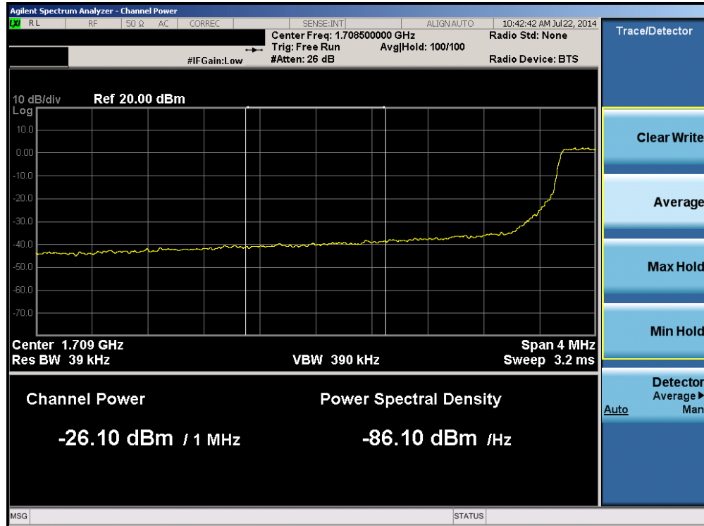
Plot 6-61. Lower Extended Band Edge Plot (Band 4 – 5.0MHz QPSK – RB Size 25)
