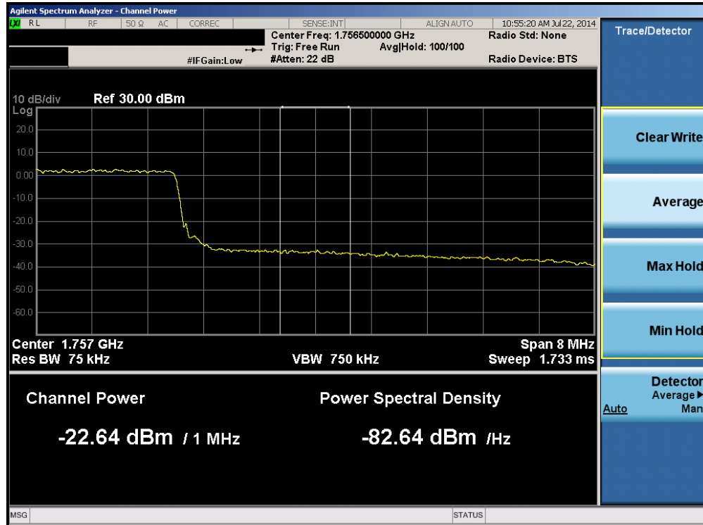
Plot 6-67. Upper Extended Band Edge Plot (Band 4 – 10.0MHz QPSK – RB Size 50)
