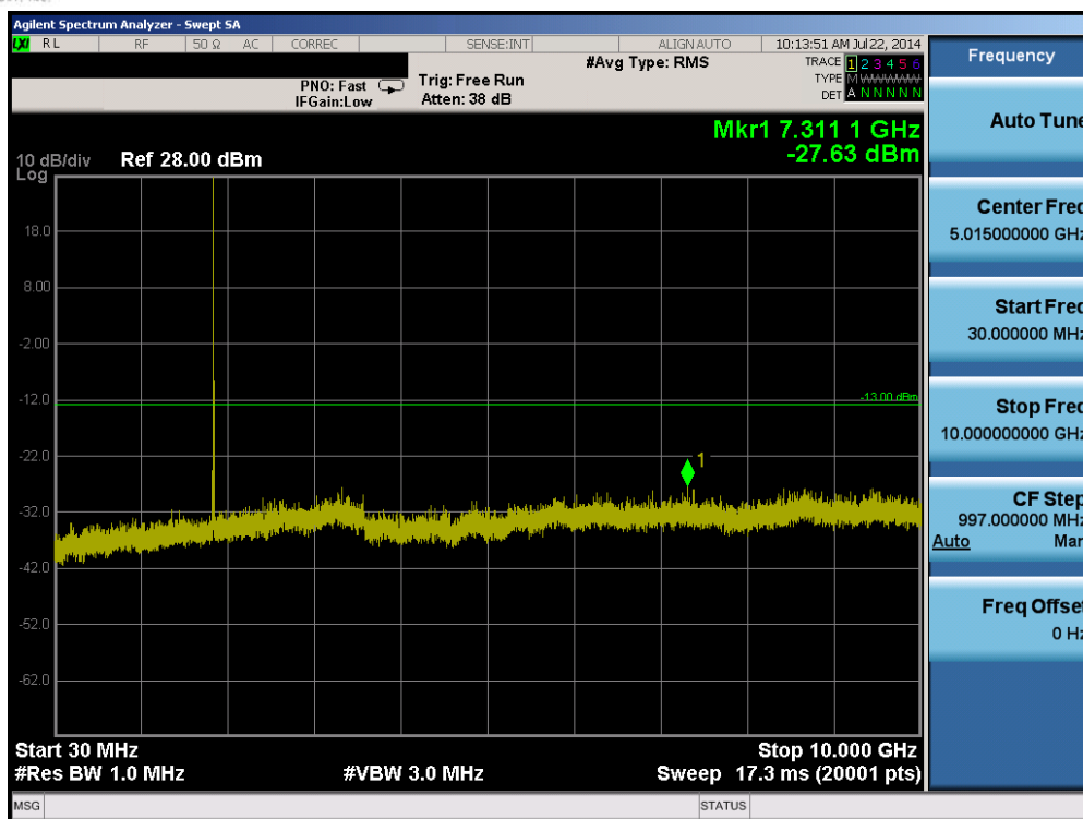
Plot 6-41. Conducted Spurious Plot (Band 2 – 15.0MHz QPSK – RB Size 1, RB Offset 0 – Low Channel)
