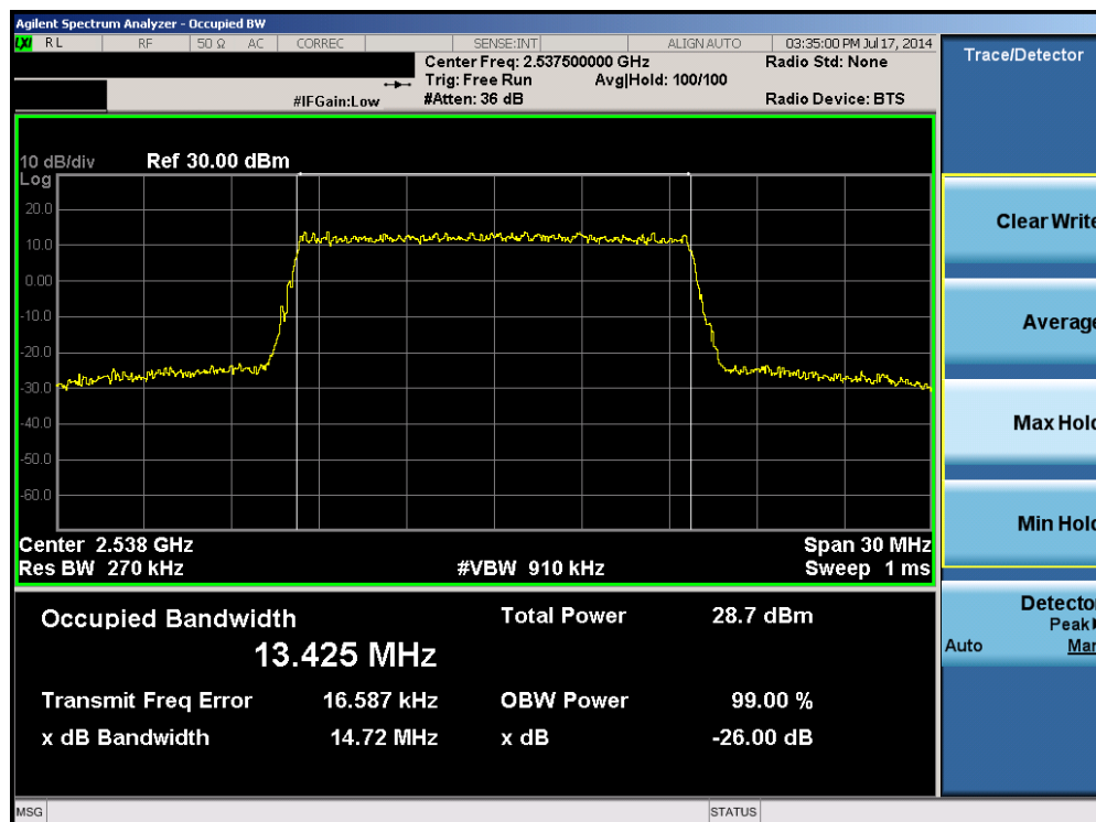
Plot 6-26. Occupied Bandwidth Plot (Band 7 – 15.0MHz 16-QAM – RB Size 75)
