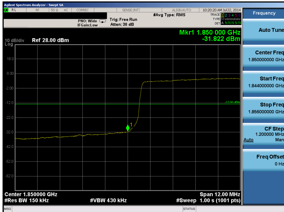
Plot 6-84. Lower Band Edge Plot (Band 2 – 15.0MHz QPSK – RB Size 75)
