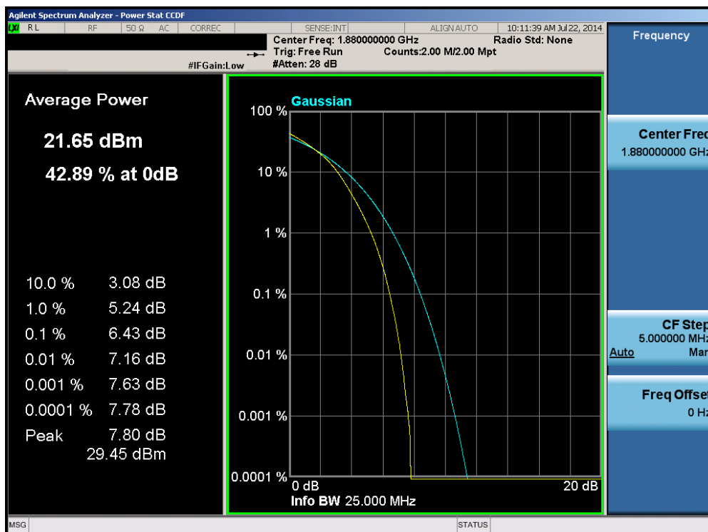
Plot 6-109. PAR Plot (Band 2 – 15.0MHz 16-QAM – RB Size 75)
