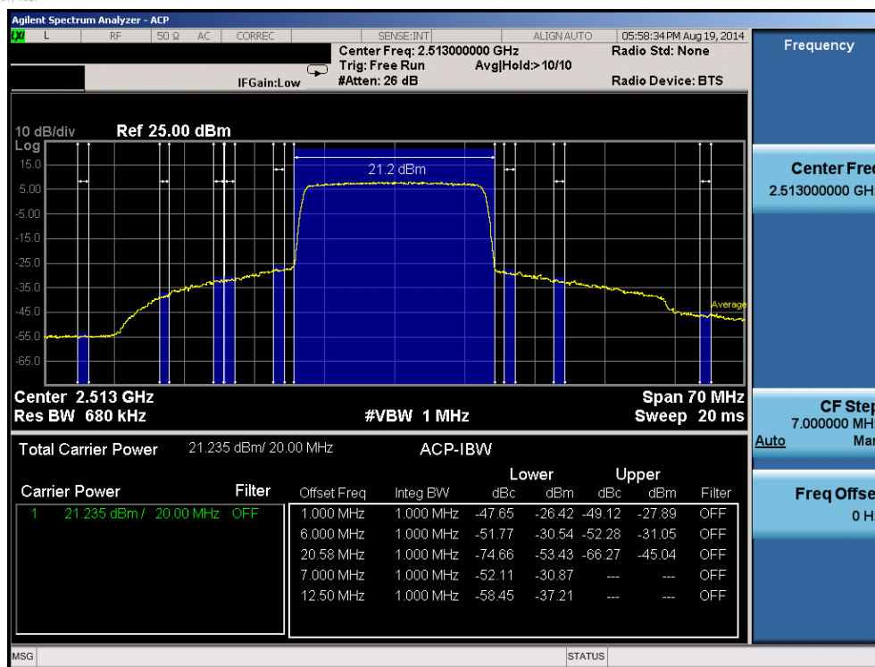
Plot 6-101. Lower ACP Plot (Band 7 – 20.0MHz QPSK – RB Size 100)
