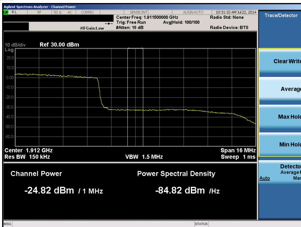
Plot 6-91. Upper Extended Band Edge Plot (Band 2 – 20.0MHz QPSK – RB Size 100)
