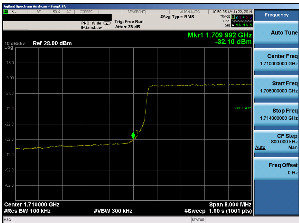
Plot 6-64. Lower Band Edge Plot (Band 4 – 10.0MHz QPSK – RB Size 50)
