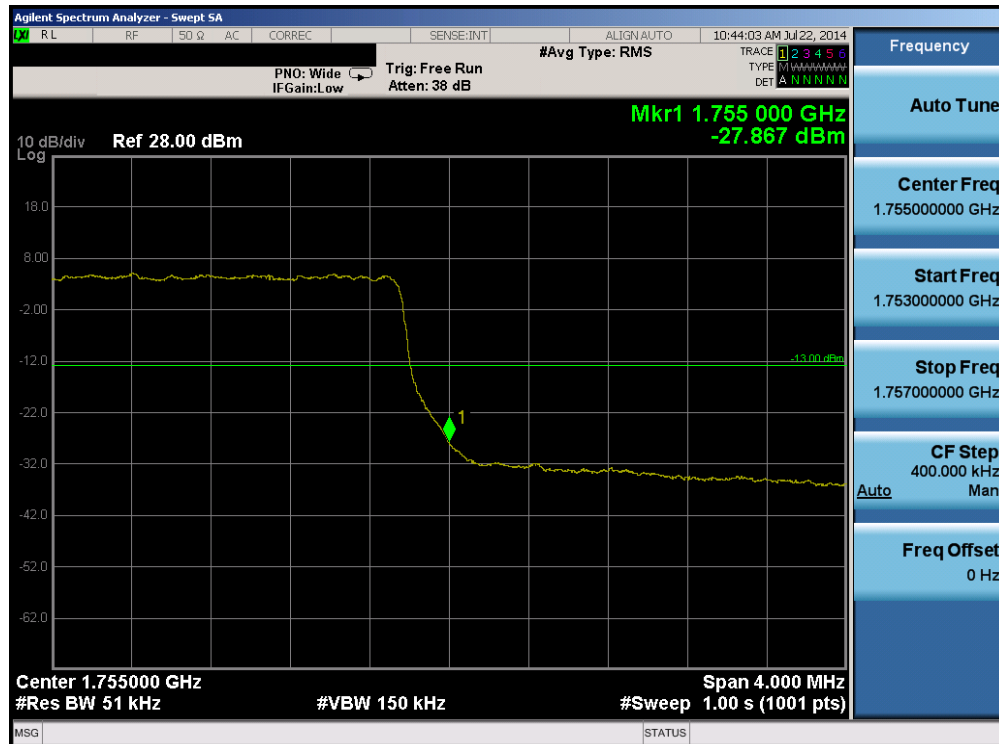
Plot 6-62. Upper Band Edge Plot (Band 4 – 5.0MHz QPSK – RB Size 25)
