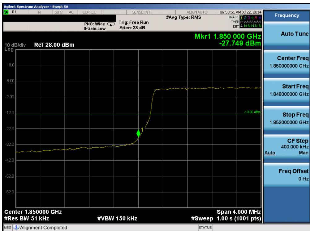
Plot 6-76. Lower Band Edge Plot (Band 2 – 5.0MHz QPSK – RB Size 25)
