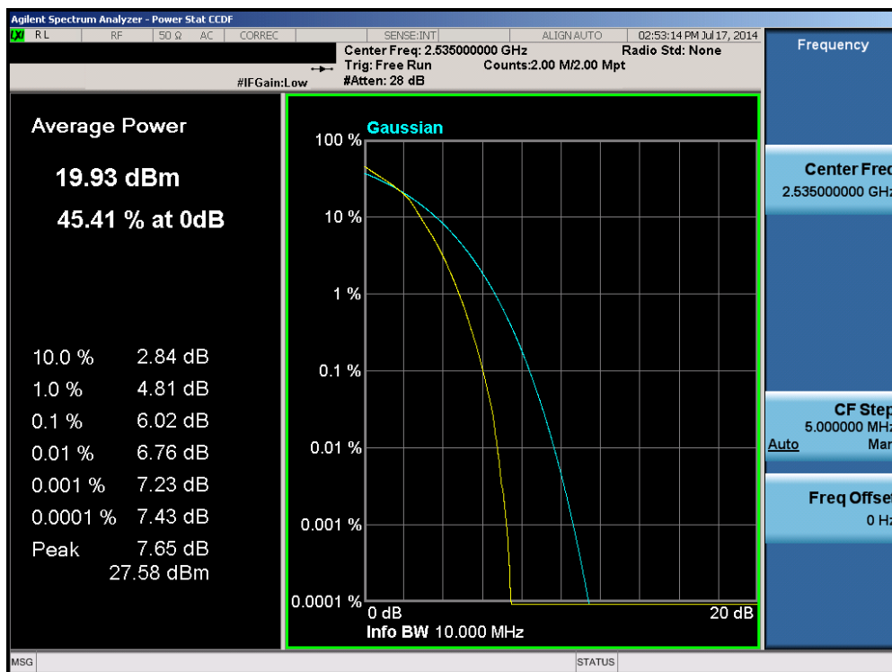
Plot 6-115. PAR Plot (Band 7 – 10.0MHz 16-QAM – RB Size 50)
