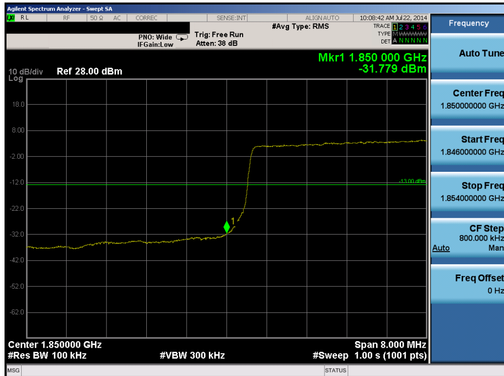
Plot 6-80. Lower Band Edge Plot (Band 2 – 10.0MHz QPSK – RB Size 50)
