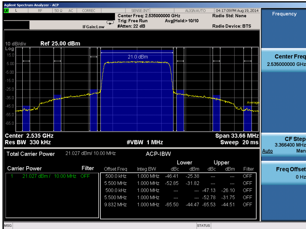
Plot 6-96. Mid ACP Plot (Band 7 – 10.0MHz QPSK – RB Size 50)
