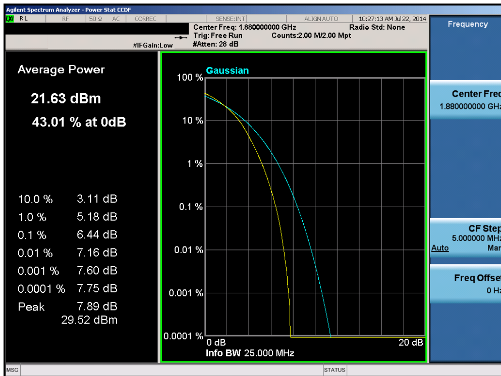
Plot 6-111. PAR Plot (Band 2 – 20.0MHz 16-QAM – RB Size 100)
