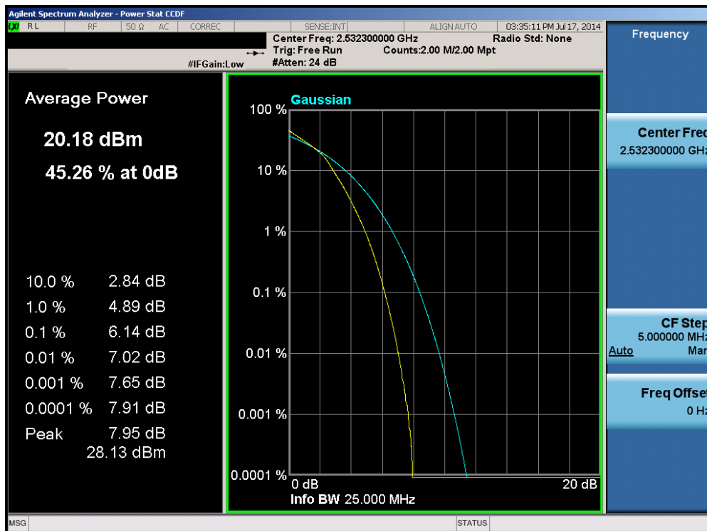
Plot 6-117. PAR Plot (Band 7 – 15.0MHz 16-QAM – RB Size 75)
