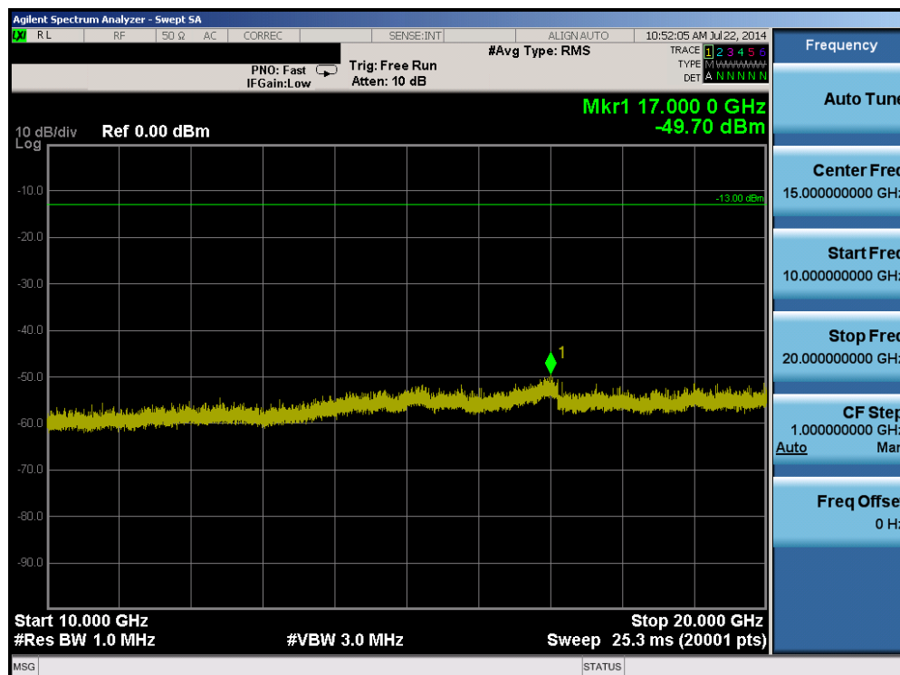
Plot 6-40. Conducted Spurious Plot (Band 4 – 10.0MHz QPSK – RB Size 1, RB Offset 0 – High Channel)
