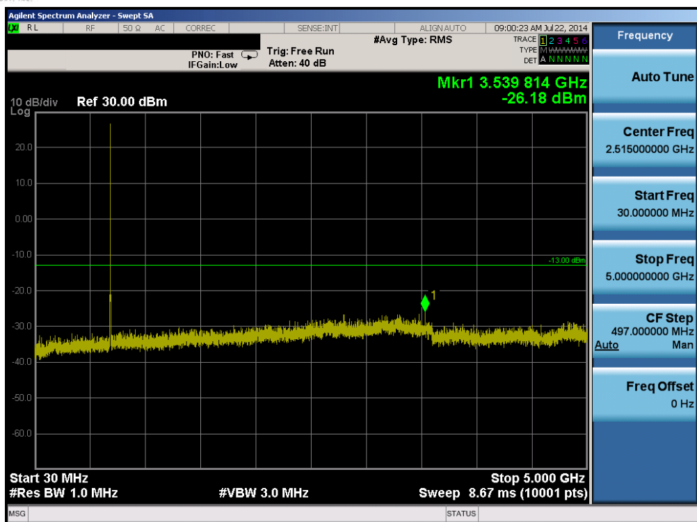
Plot 6-31. Conducted Spurious Plot (Band 17 – 5.0MHz QPSK – RB Size 1, RB Offset 0 – Mid Channel)
