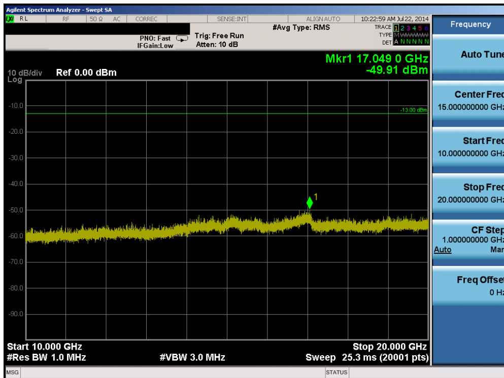
Plot 6-46. Conducted Spurious Plot (Band 2 – 15.0MHz QPSK – RB Size 1, RB Offset 0 – High Channel)
