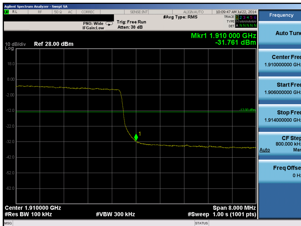
Plot 6-82. Upper Band Edge Plot (Band 2 – 10.0MHz QPSK – RB Size 50)
