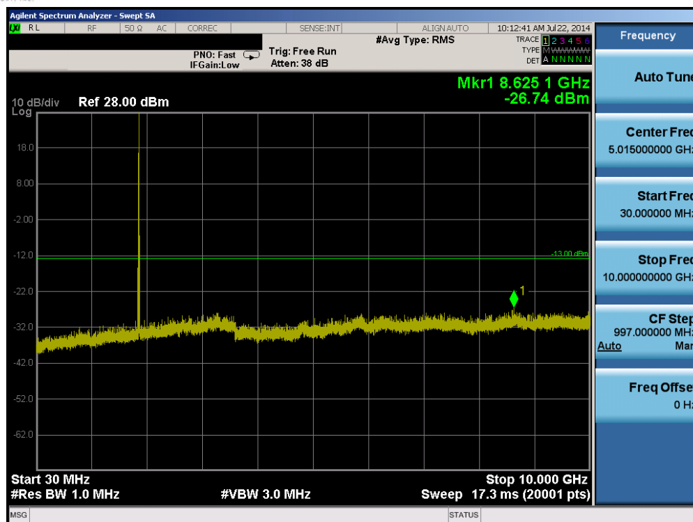
Plot 6-43. Conducted Spurious Plot (Band 2 – 15.0MHz QPSK – RB Size 1, RB Offset 0 – Mid Channel)
