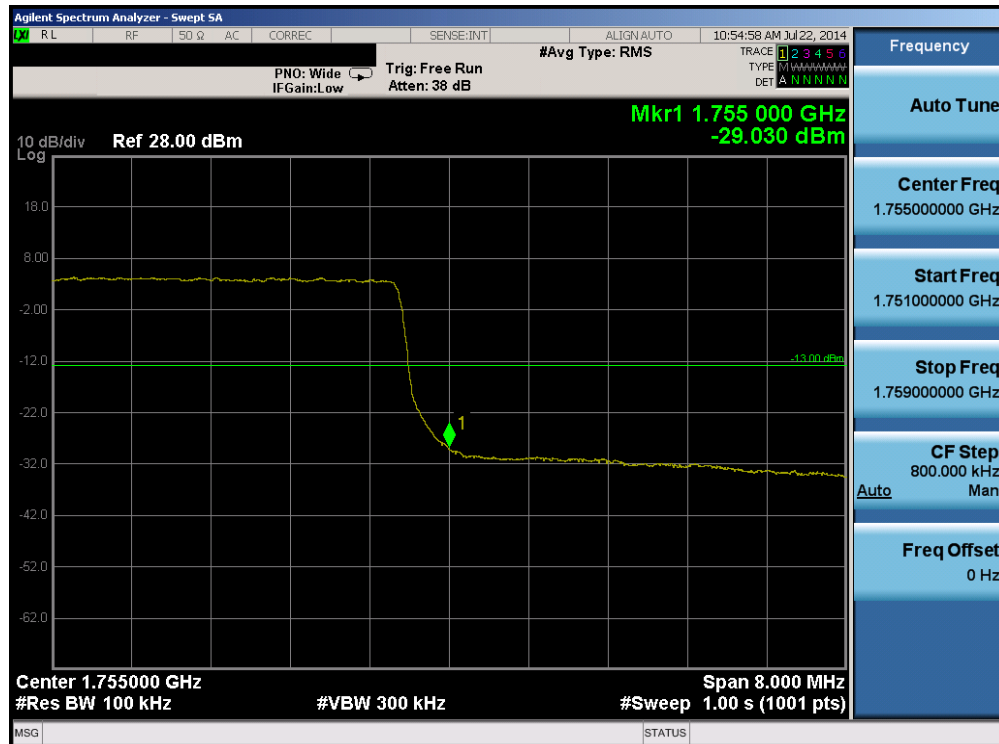
Plot 6-66. Upper Band Edge Plot (Band 4 – 10.0MHz QPSK – RB Size 50)
