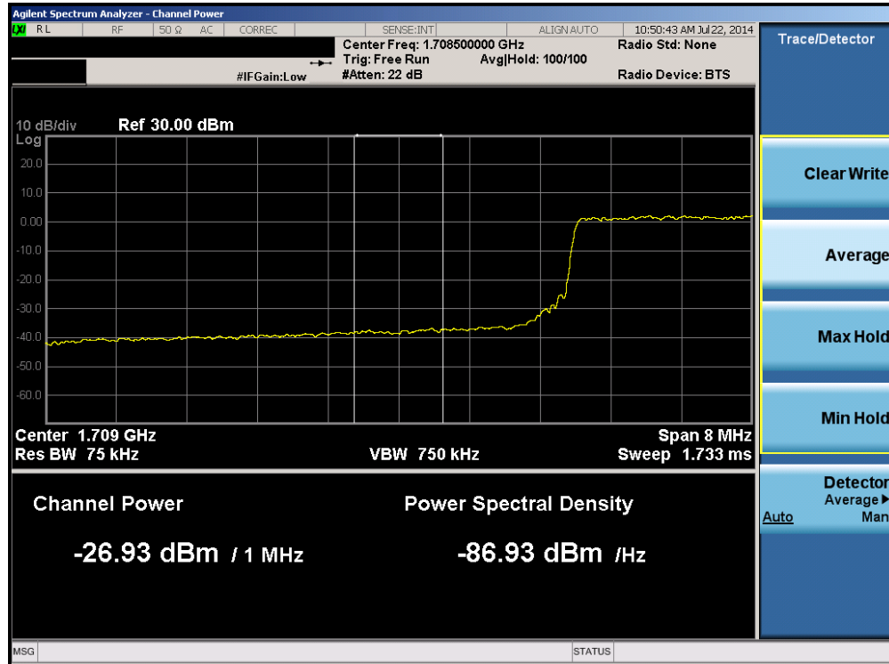
Plot 6-65. Lower Extended Band Edge Plot (Band 4 – 10.0MHz QPSK – RB Size 50)
