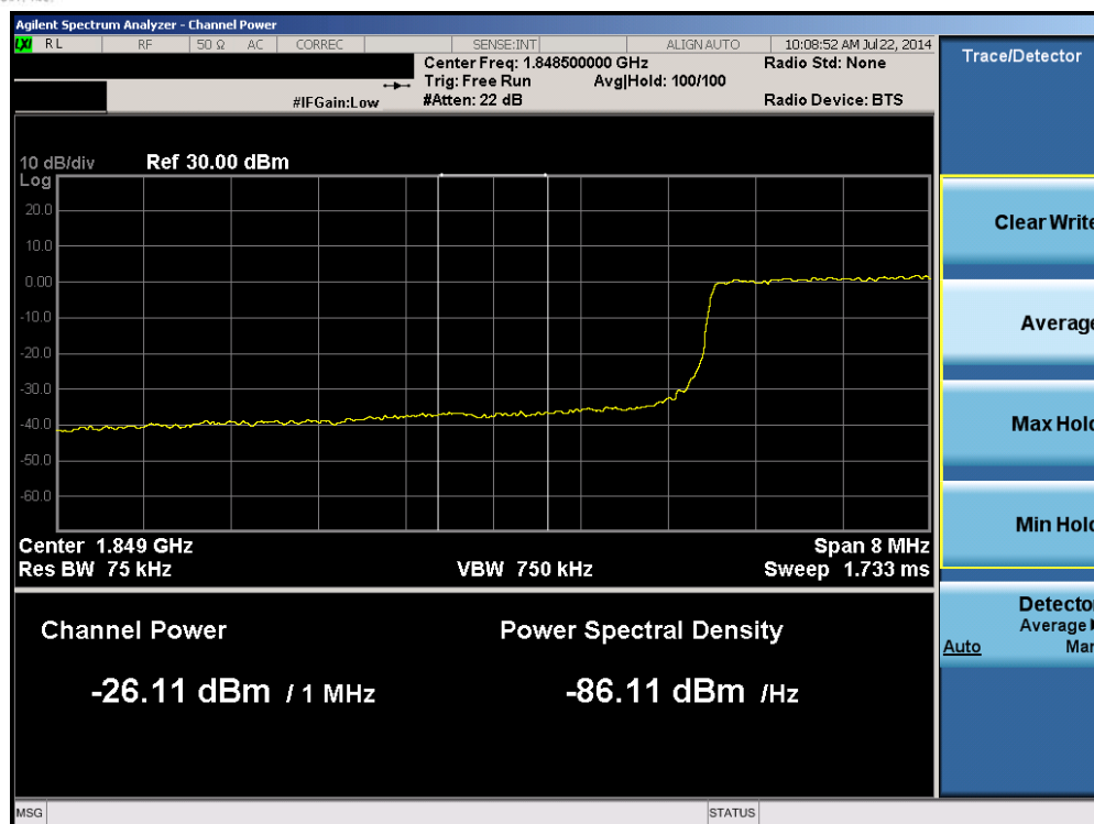
Plot 6-81. Lower Extended Band Edge Plot (Band 2 – 10.0MHz QPSK – RB Size 50)
