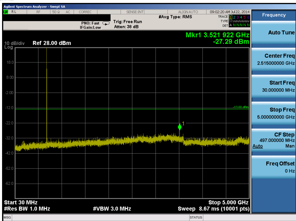
Plot 6-29. Conducted Spurious Plot (Band 17 – 5.0MHz QPSK – RB Size 1, RB Offset 0 – Low Channel)
