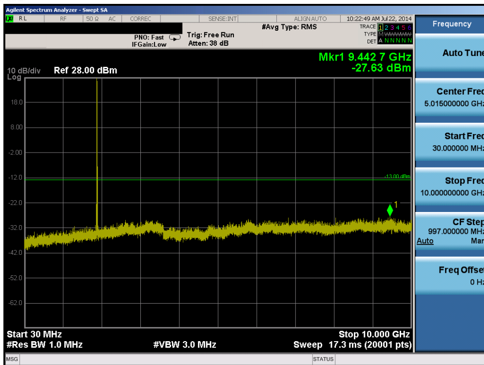
Plot 6-45. Conducted Spurious Plot (Band 2 – 15.0MHz QPSK – RB Size 1, RB Offset 0 – High Channel)
