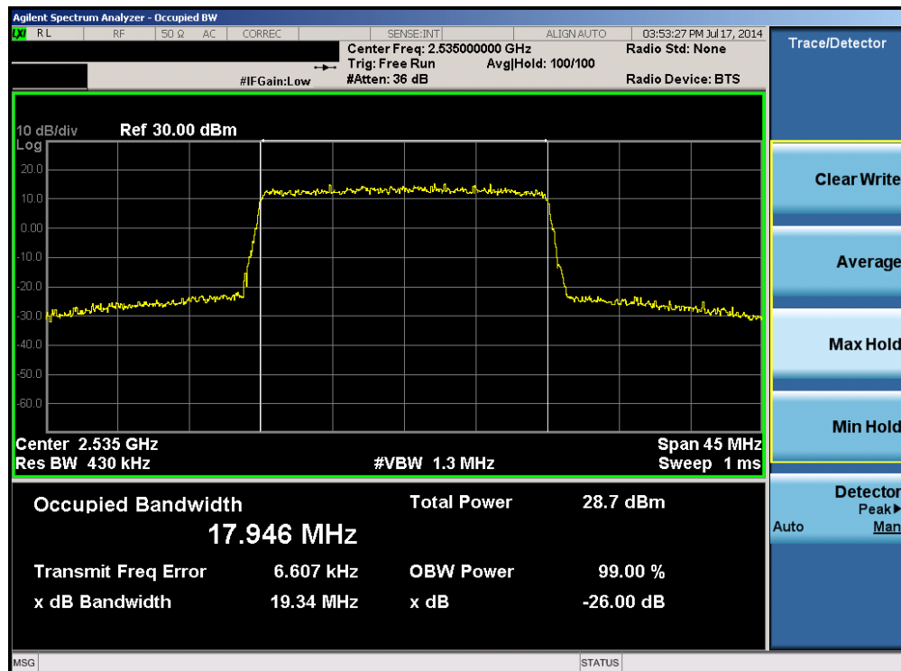
Plot 6-28. Occupied Bandwidth Plot (Band 7 – 20.0MHz 16-QAM – RB Size 100)
