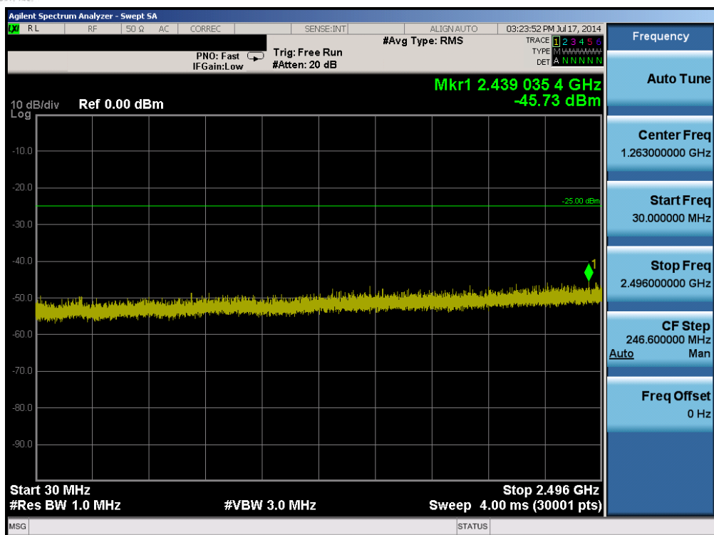
Plot 6-51. Conducted Spurious Plot (Band 7 – 10.0MHz QPSK – RB Size 1, RB Offset 0 – High Channel)
