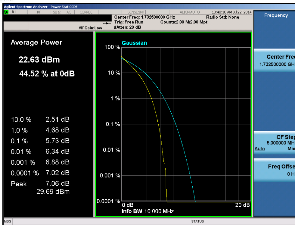
Plot 6-122. PAR Plot (Band 4 – 10.0MHz – QPSK – RB Size 50)
