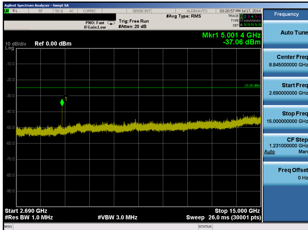
Plot 6-48. Conducted Spurious Plot (Band 7 – 10.0MHz QPSK – RB Size 1, RB Offset 0 – Low Channel)
