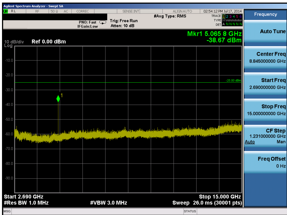
Plot 6-50. Conducted Spurious Plot (Band 7 – 10.0MHz QPSK – RB Size 1, RB Offset 0 – Mid Channel)
