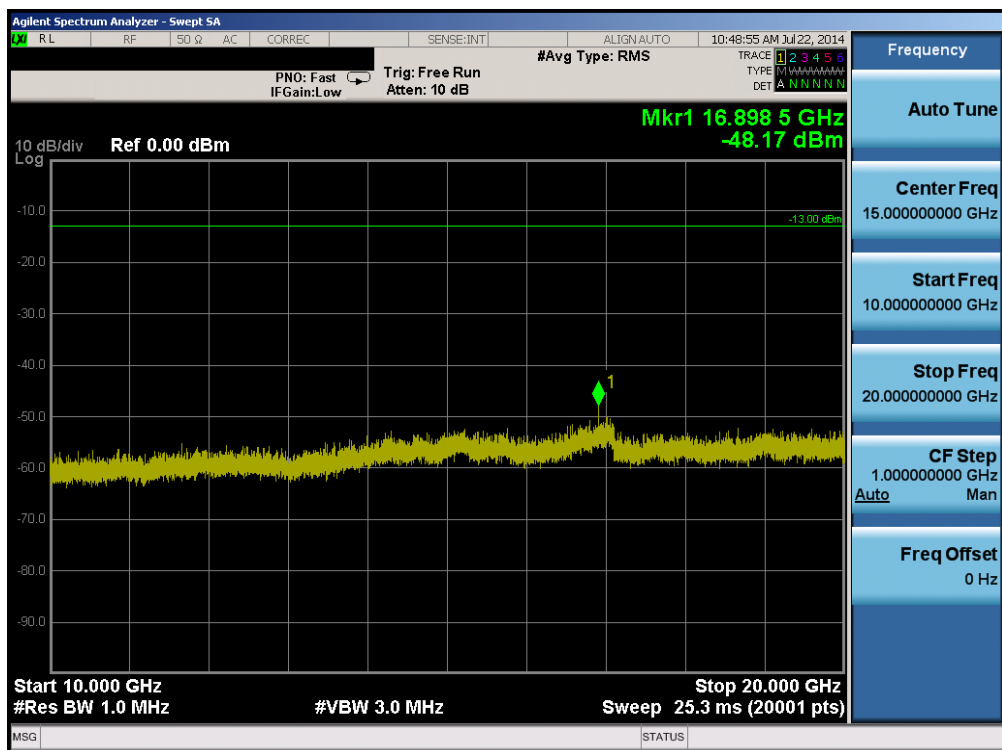
Plot 6-38. Conducted Spurious Plot (Band 4 – 10.0MHz QPSK – RB Size 1, RB Offset 0 – Mid Channel)
