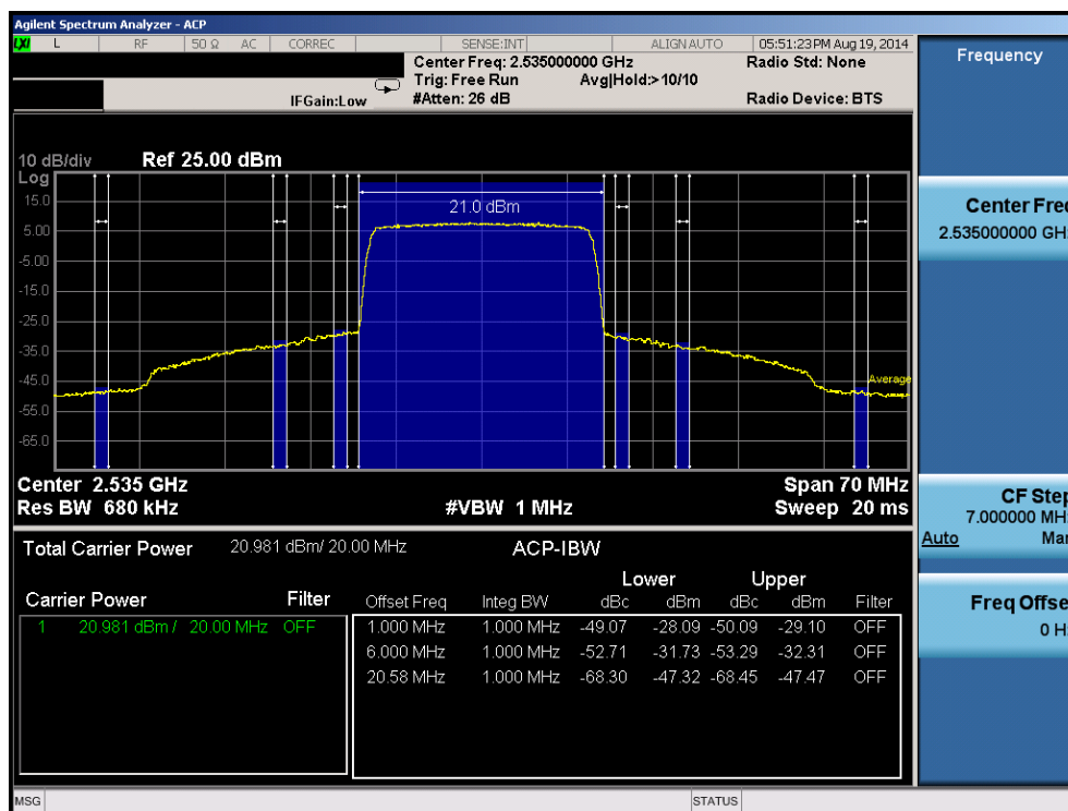
Plot 6-102. Mid ACP Plot (Band 7 – 20.0MHz QPSK – RB Size 100)
