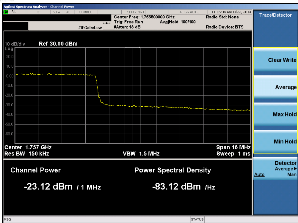
Plot 6-75. Upper Extended Band Edge Plot (Band 4 – 20.0MHz QPSK – RB Size 100)
