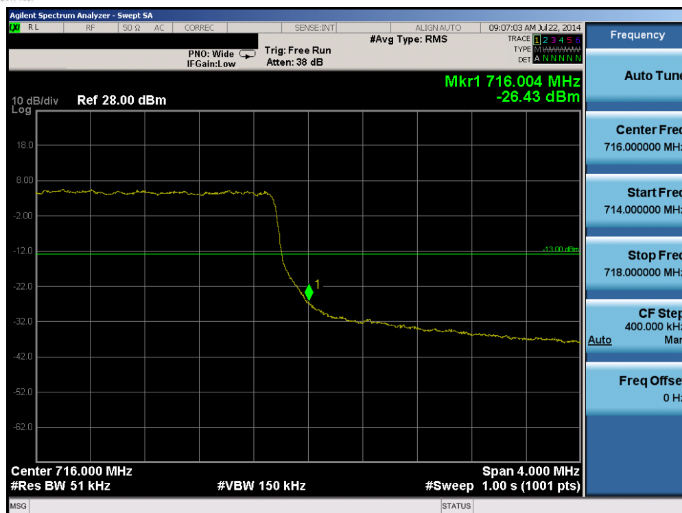
Plot 6-55. Upper Band Edge Plot (Band 17 – 5.0MHz QPSK – RB Size 25)
