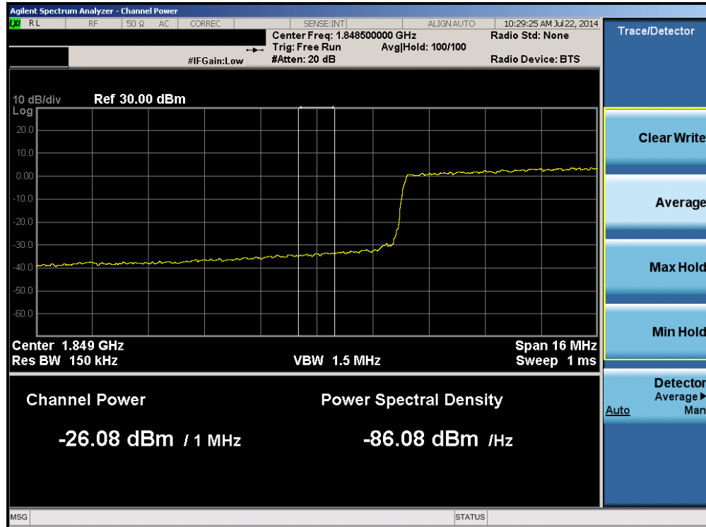
Plot 6-89. Lower Extended Band Edge Plot (Band 2 – 20.0MHz QPSK – RB Size 100)
