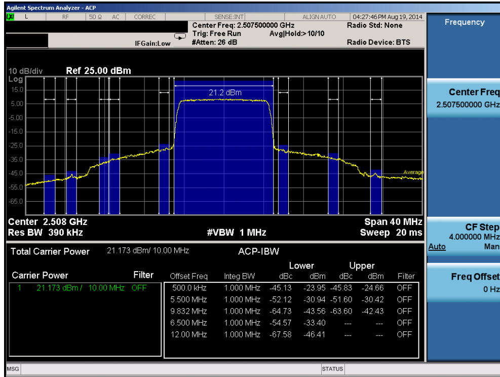
Plot 6-95. Lower ACP Plot (Band 7 – 10.0MHz QPSK – RB Size 50)
