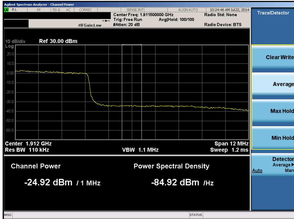
Plot 6-87. Upper Extended Band Edge Plot (Band 2 – 15.0MHz QPSK – RB Size 75)
