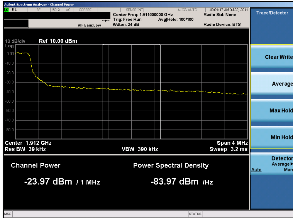
Plot 6-79. Upper Extended Band Edge Plot (Band 2 – 5.0MHz QPSK – RB Size 25)
