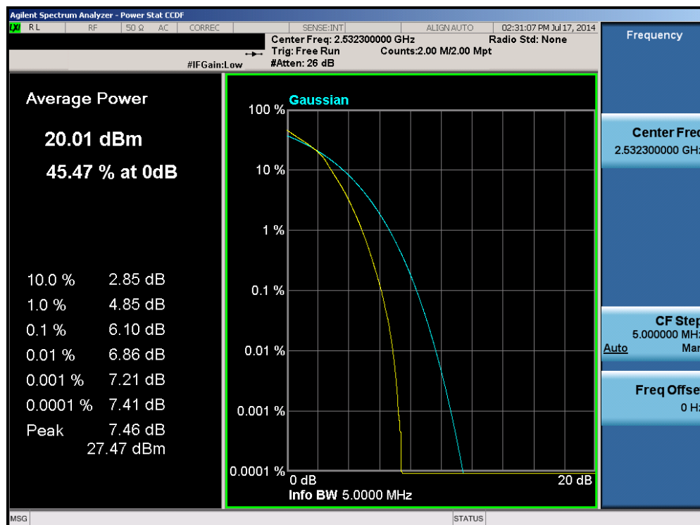
Plot 6-113. PAR Plot (Band 7 – 5.0MHz 16-QAM – RB Size 25)
