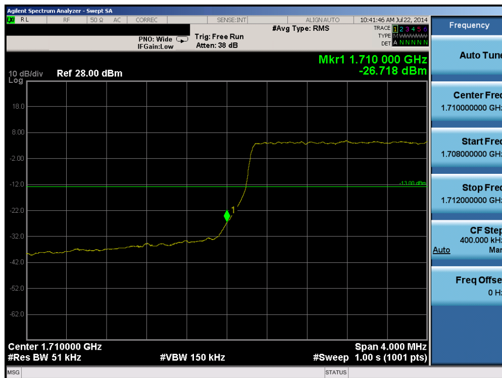
Plot 6-60. Lower Band Edge Plot (Band 4 – 5.0MHz QPSK – RB Size 25)
