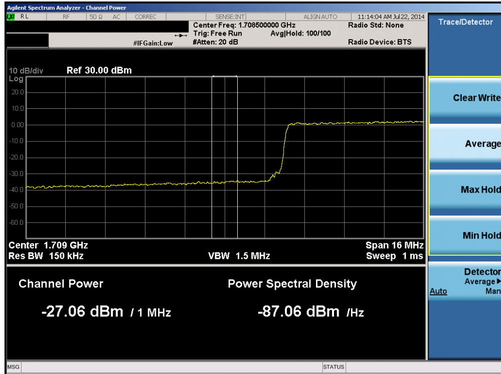
Plot 6-73. Lower Extended Band Edge Plot (Band 4 – 20.0MHz QPSK – RB Size 100)
