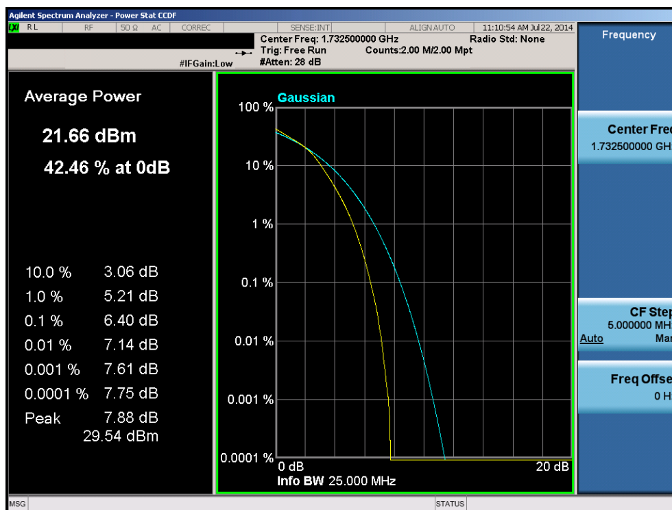
Plot 6-127. PAR Plot (Band 4 – 20.0MHz – 16-QAM – RB Size 100)
