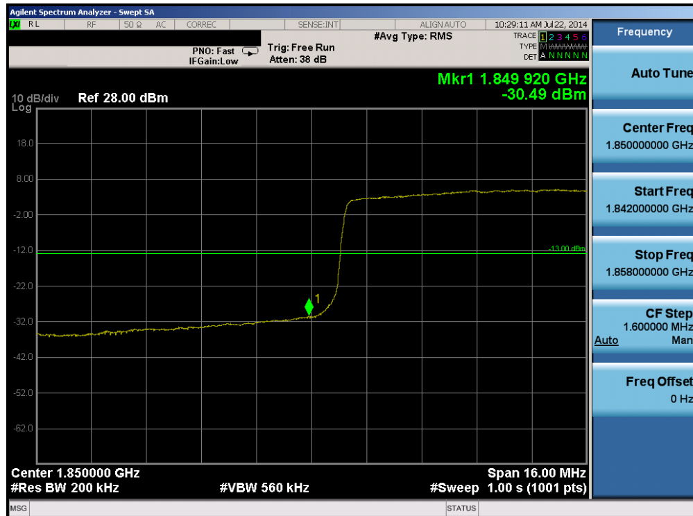
Plot 6-88. Lower Band Edge Plot (Band 2 – 20.0MHz QPSK – RB Size 100)
