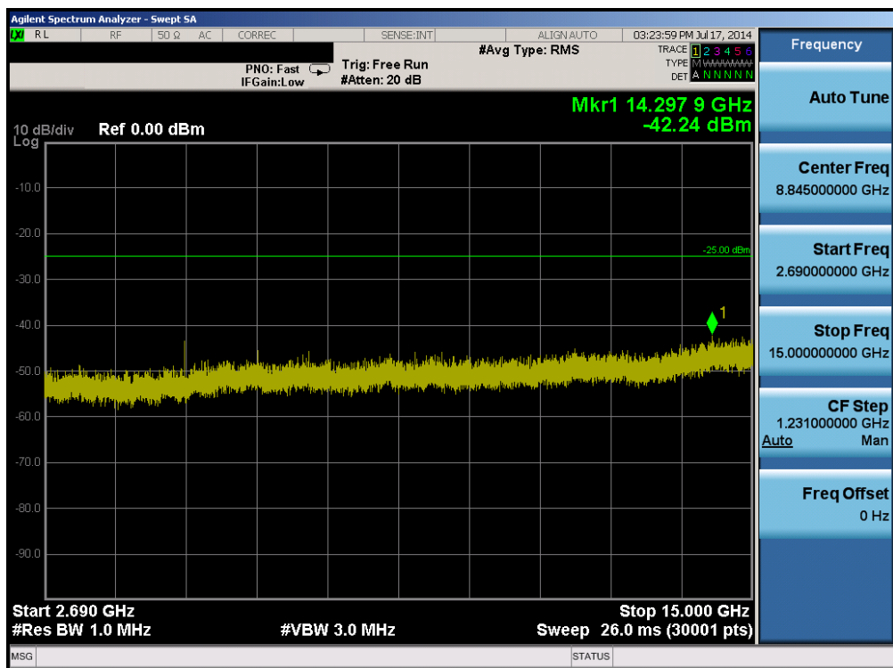
Plot 6-52. Conducted Spurious Plot (Band 7 – 10.0MHz QPSK – RB Size 1, RB Offset 0 – High Channel)
