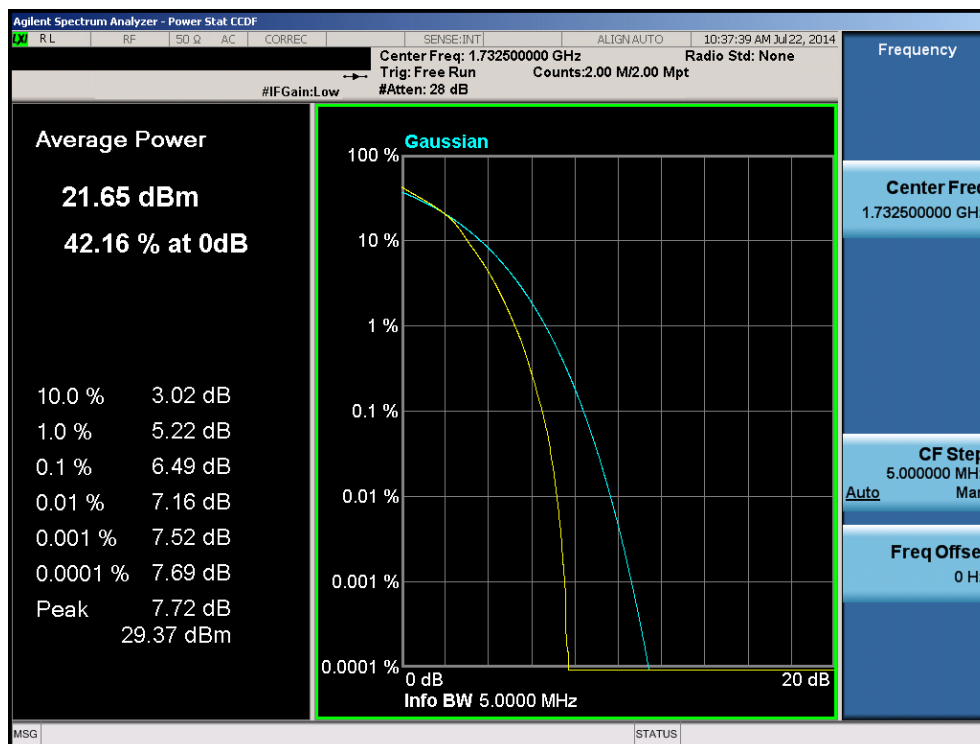
Plot 6-121. PAR Plot (Band 4 – 5.0MHz 16-QAM – RB Size 25)
