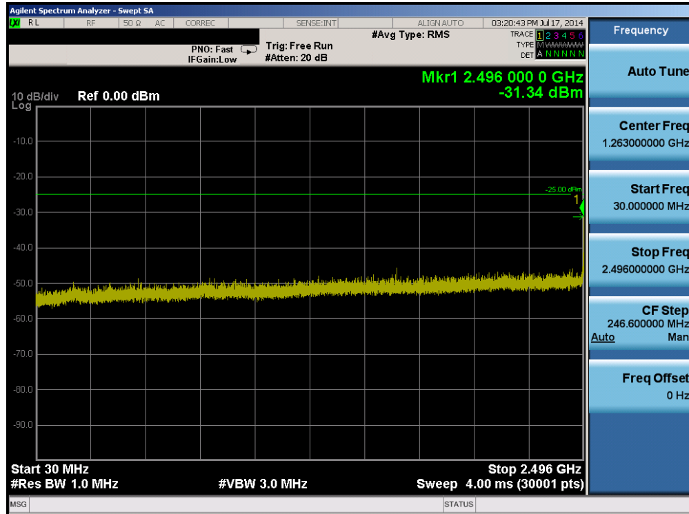
Plot 6-47. Conducted Spurious Plot (Band 7 – 10.0MHz QPSK – RB Size 1, RB Offset 0– Low Channel)
