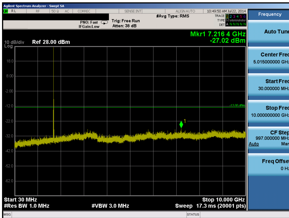
Plot 6-35. Conducted Spurious Plot (Band 4 – 10.0MHz QPSK – RB Size 1, RB Offset 0– Low Channel)
