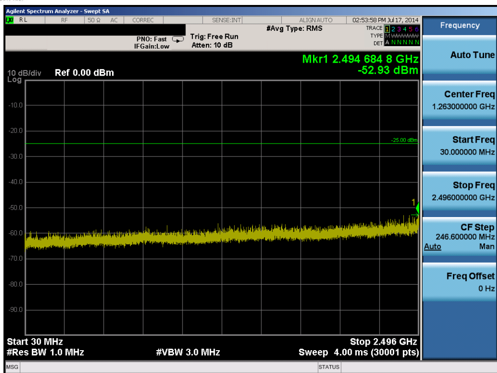
Plot 6-49. Conducted Spurious Plot (Band 7 – 10.0MHz QPSK – RB Size 1, RB Offset 0 – Mid Channel)
