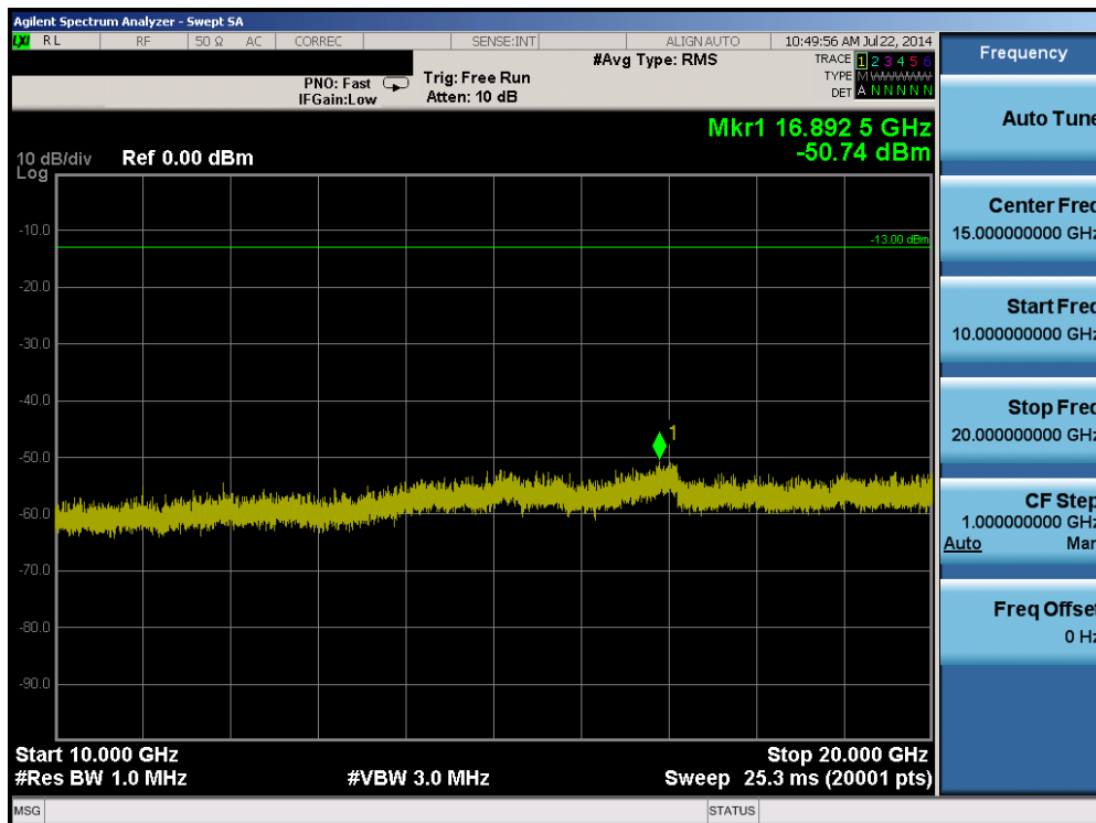
Plot 6-36. Conducted Spurious Plot (Band 4 – 10.0MHz QPSK – RB Size 1, RB Offset 0 – Low Channel)
