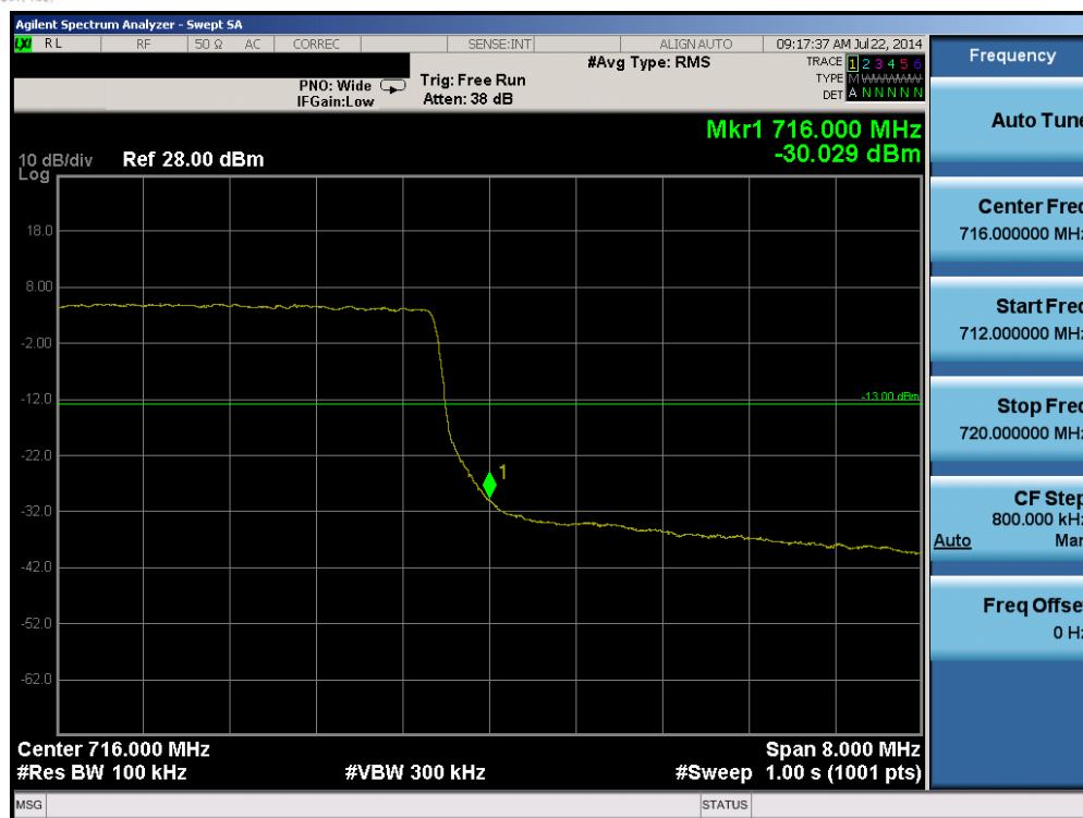
Plot 6-59. Upper Band Edge Plot (Band 17 – 10.0MHz QPSK – RB Size 50)
