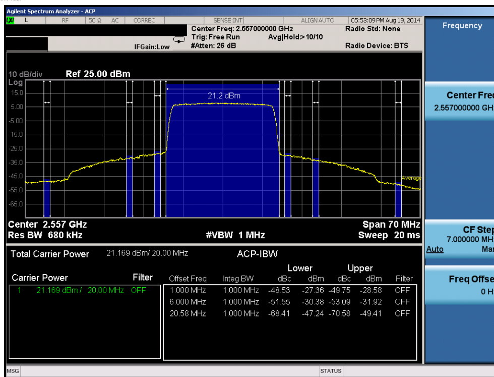
Plot 6-103. Upper ACP Plot (Band 7 – 20.0MHz QPSK – RB Size 100)
