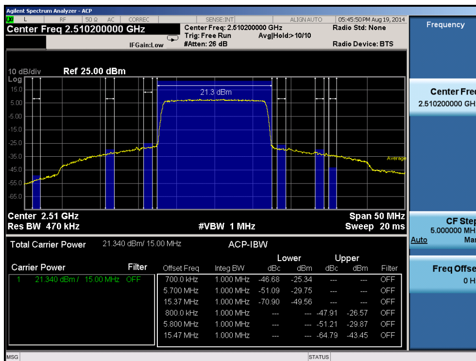
Plot 6-98. Lower ACP Plot (Band 7 – 15.0MHz QPSK – RB Size 75)
