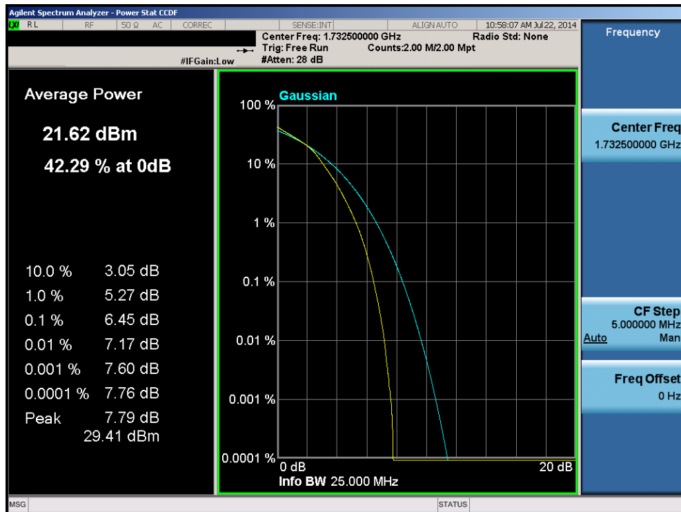
Plot 6-125. PAR Plot (Band 4 – 15.0MHz – 16-QAM – RB Size 75)
