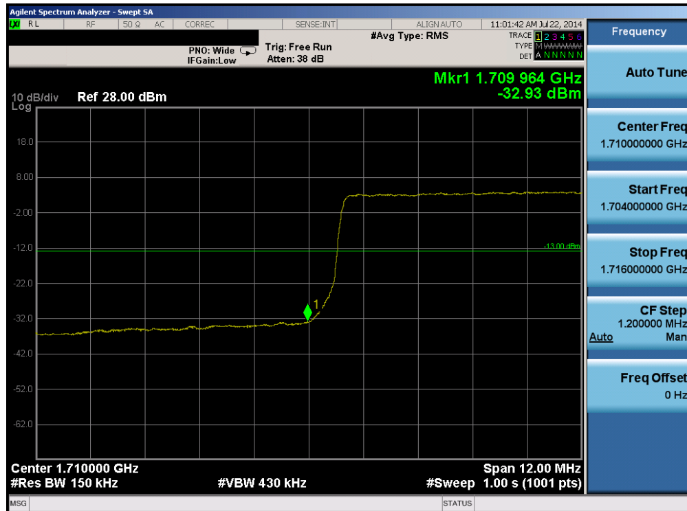
Plot 6-68. Lower Band Edge Plot (Band 4 – 15.0MHz QPSK – RB Size 75)
