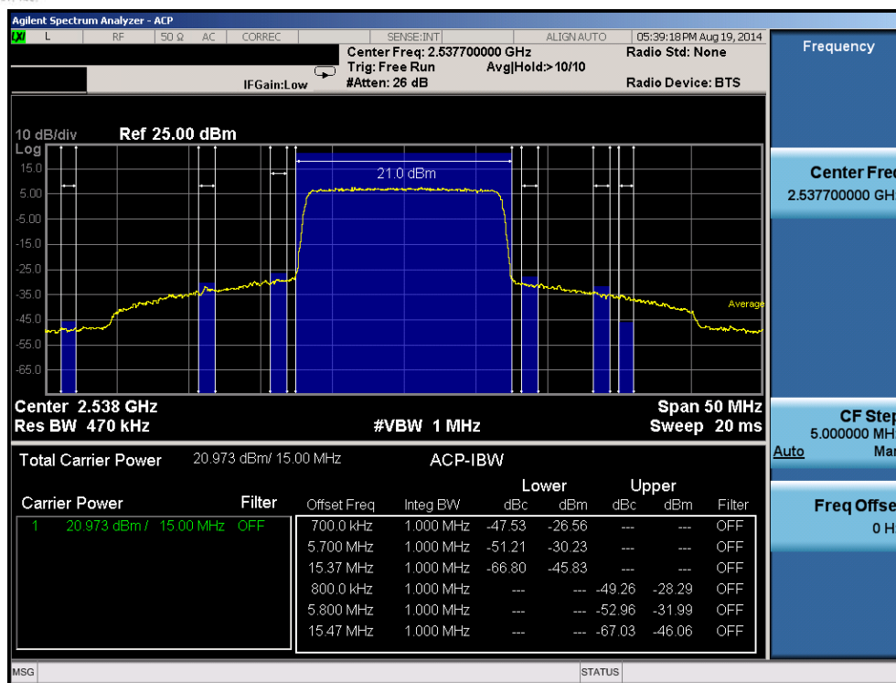
Plot 6-99. Mid ACP Plot (Band 7 – 15.0MHz QPSK – RB Size 75)
