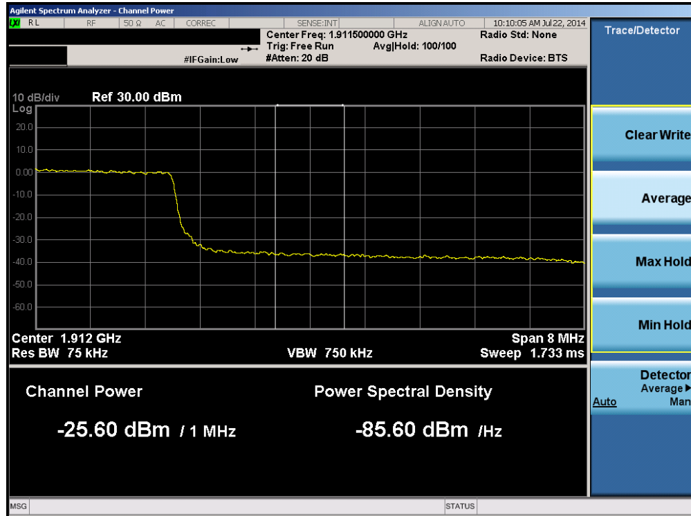
Plot 6-83. Upper Extended Band Edge Plot (Band 2 – 10.0MHz QPSK – RB Size 50)
