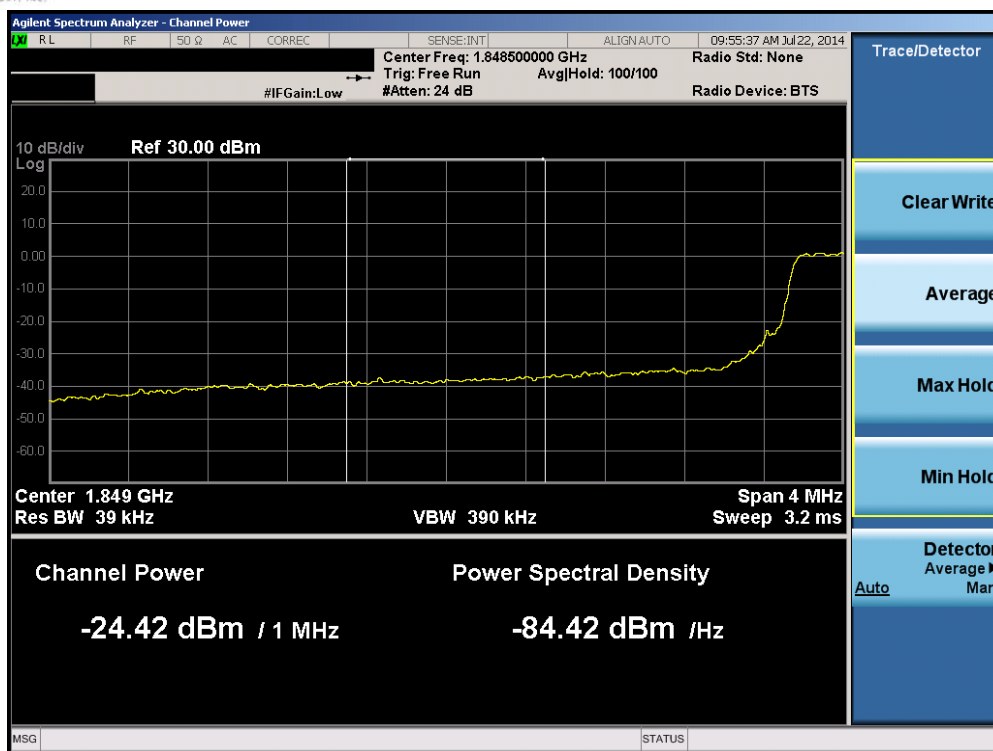
Plot 6-77. Lower Extended Band Edge Plot (Band 2 – 5.0MHz QPSK – RB Size 25)
