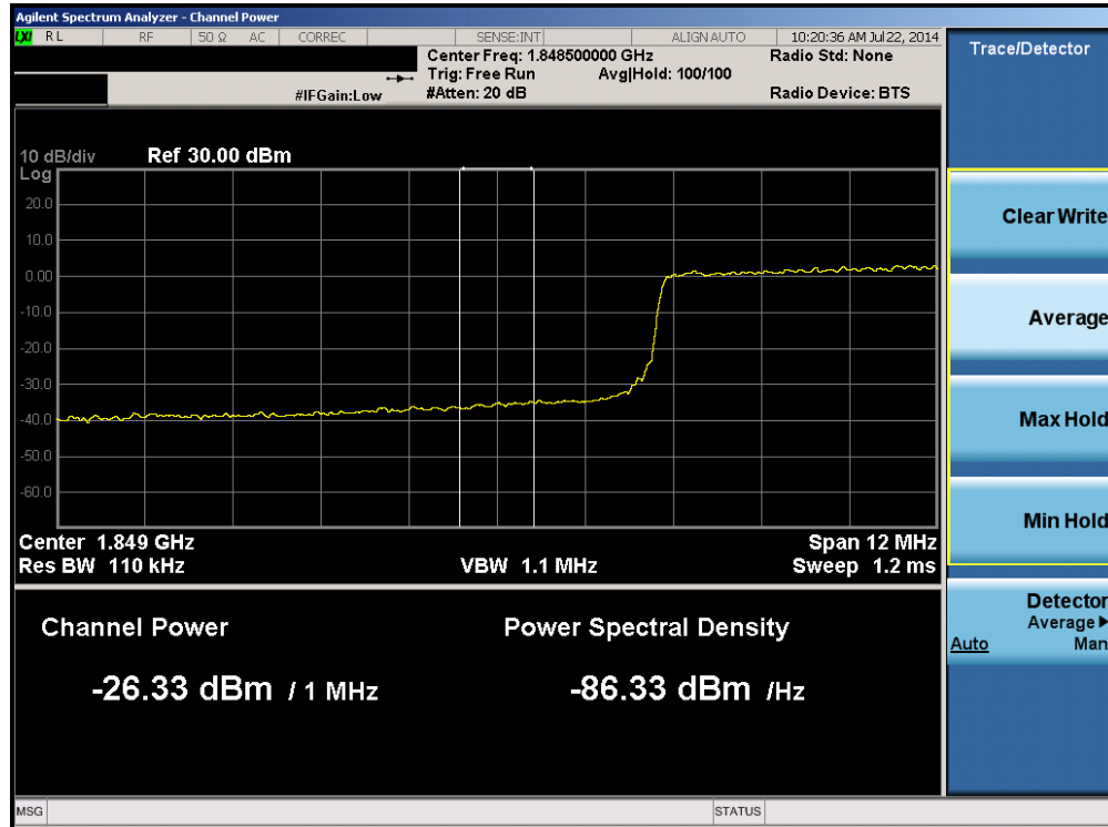
Plot 6-85. Lower Extended Band Edge Plot (Band 2 – 15.0MHz QPSK – RB Size 75)
