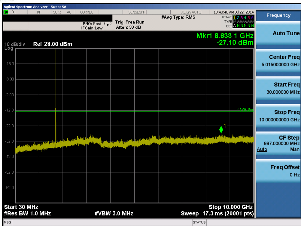
Plot 6-37. Conducted Spurious Plot (Band 4 – 10.0MHz QPSK – RB Size 1, RB Offset 0 – Mid Channel)
