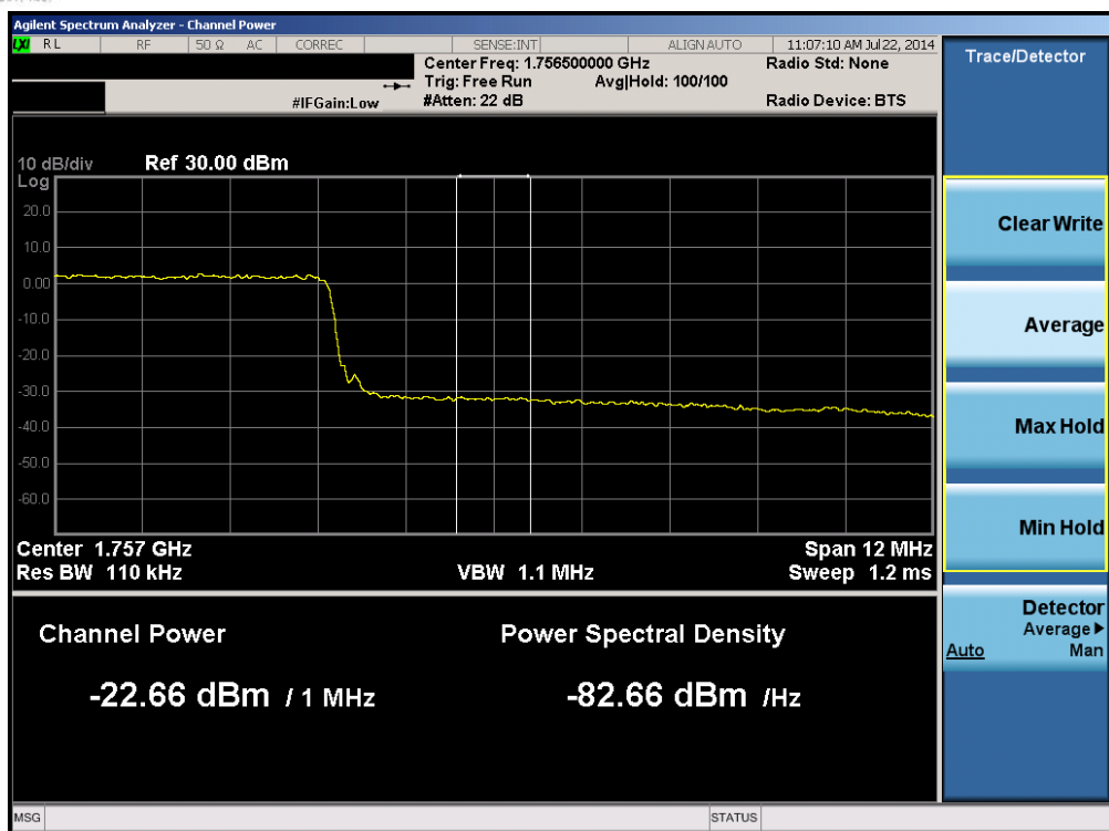
Plot 6-71. Upper Extended Band Edge Plot (Band 4 – 15.0MHz QPSK – RB Size 75)
