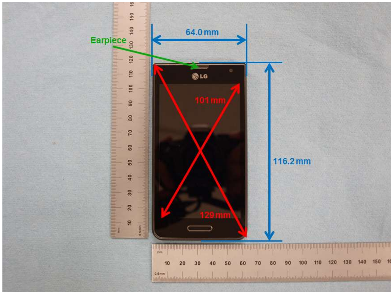
Overall Dimensions
