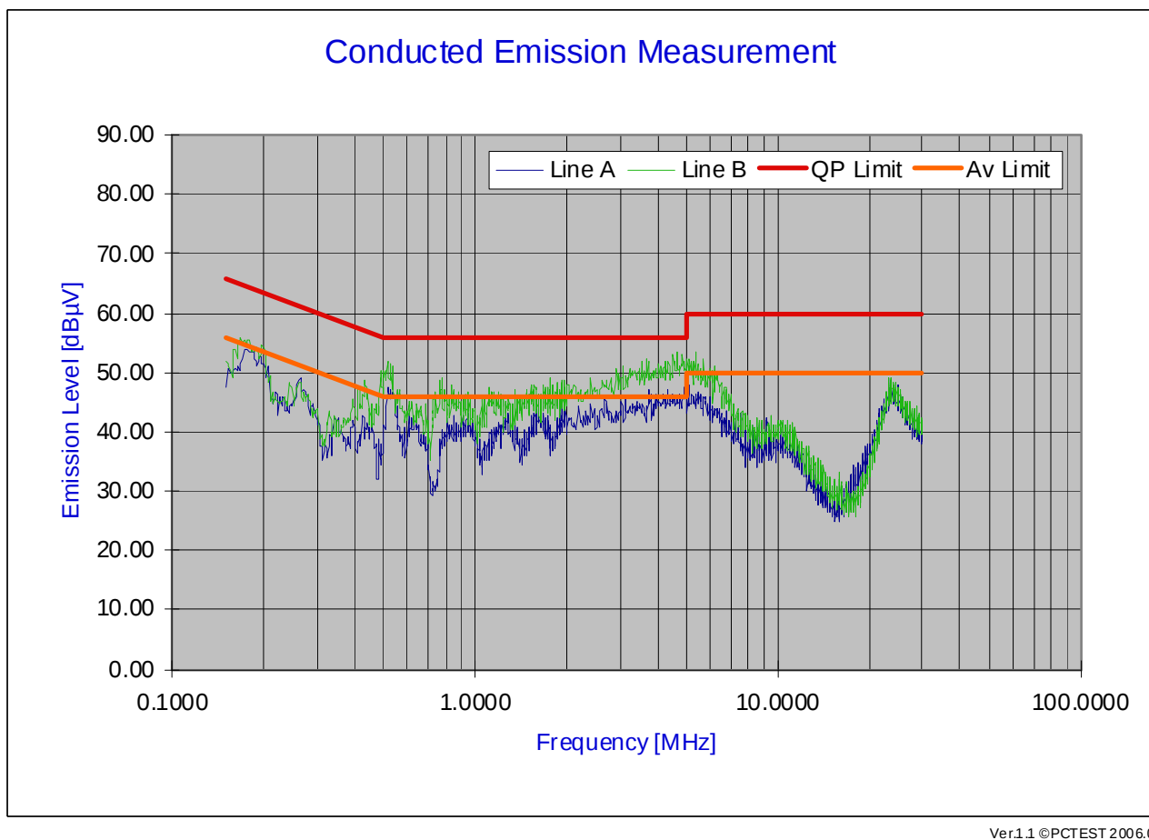
Plot 6-33. Line Conducted Plot with 802.11n
