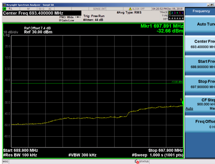
LTE Band 12, 17 / 10MHz / 64QAM - RB Size/Offset (25/0)
