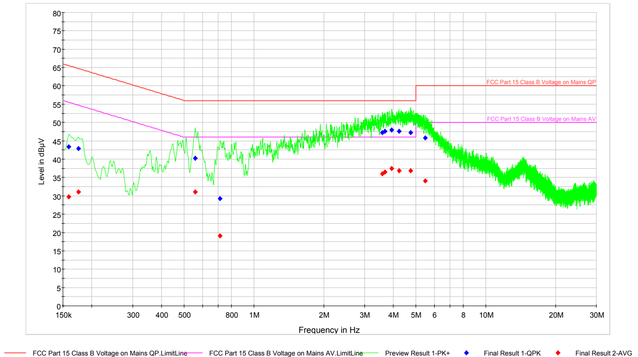
Plot 6-25. Line Conducted Plot with Bluetooth (LN)
