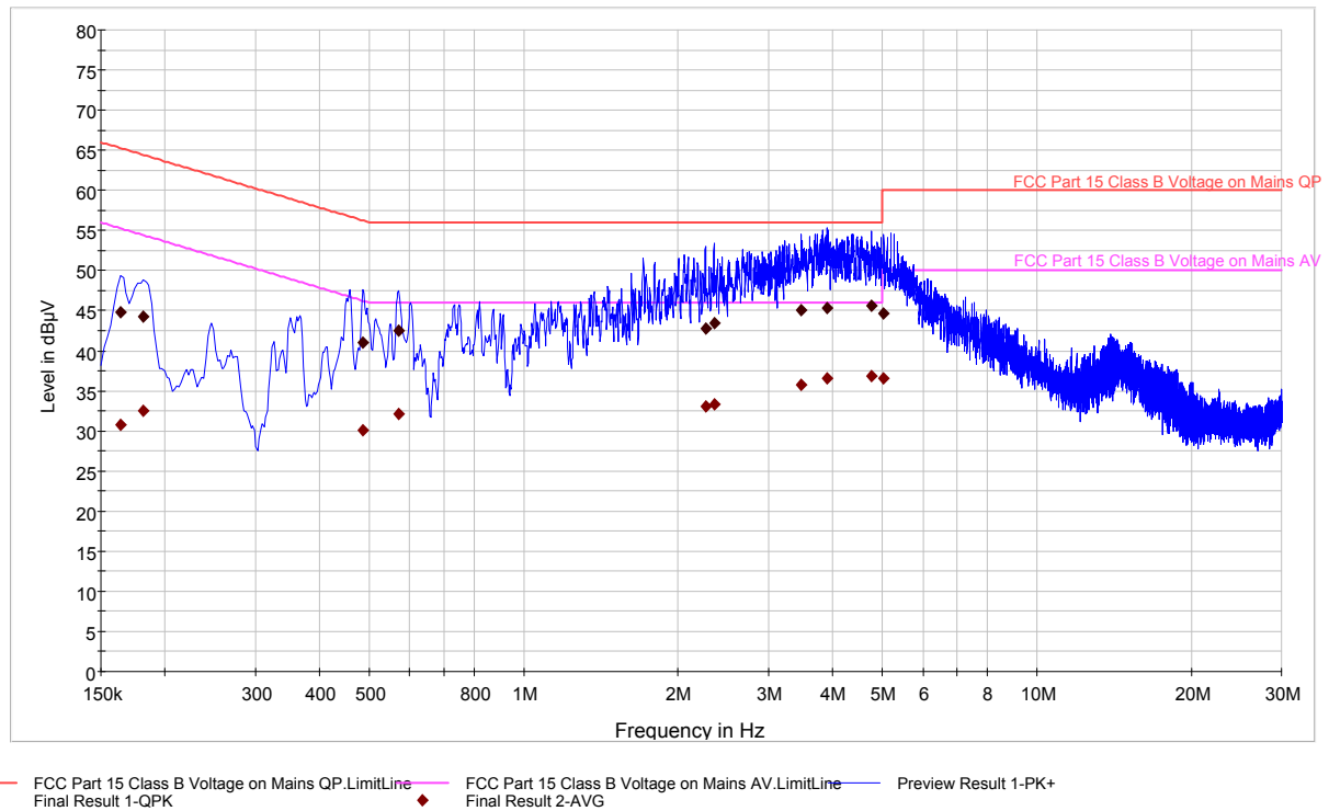
Plot 6-24. Line Conducted Plot with Bluetooth (L1)
