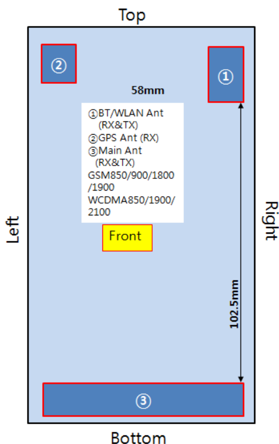
Figure 13.1 Identification of Sides for SAR Testing
