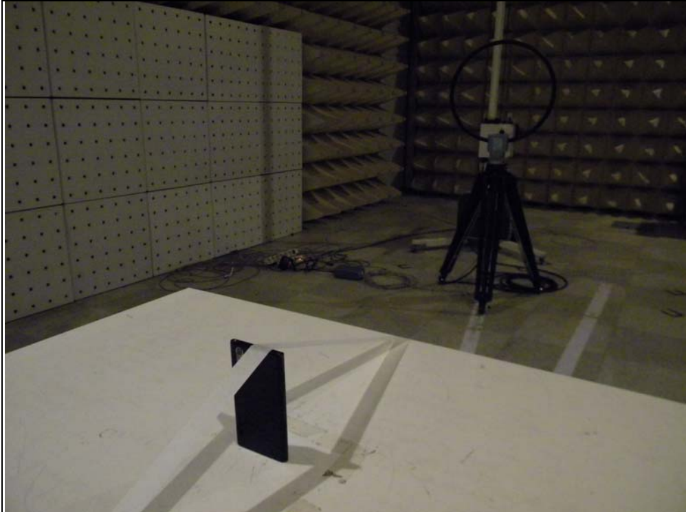
A. Photo of Field Strength & Spurious Emission Test(NFC)
