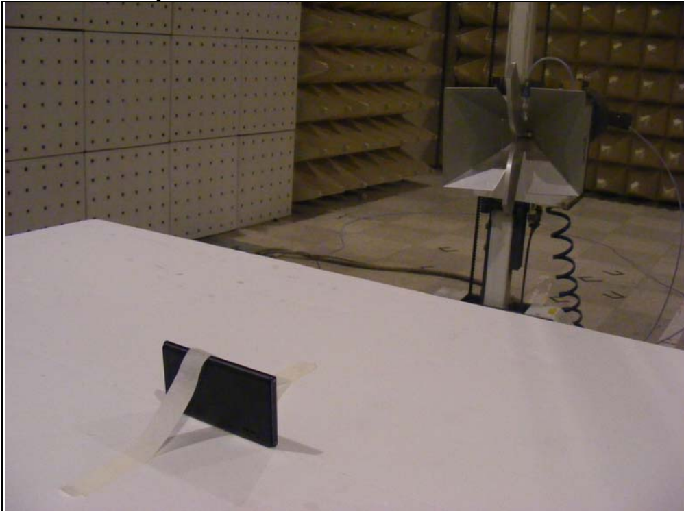
D. Photo of Field Strength & Spurious Emission Test (5GHz WLAN_1 meter)
