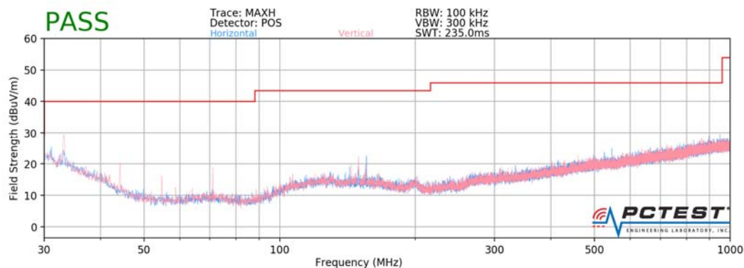
Plot 7-48. Radiated Spurious Plot below 1GHz
