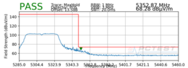
Plot 7-95. Radiated Upper Band Edge Plot (Peak – UNII Band 2A)
