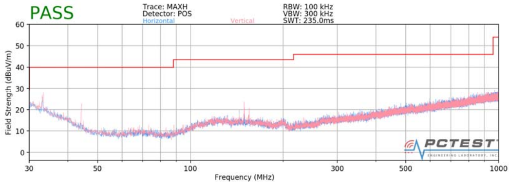
Plot 7-109. Radiated Spurious Plot below 1GHz (802.11a – U3 Ch. 157)
