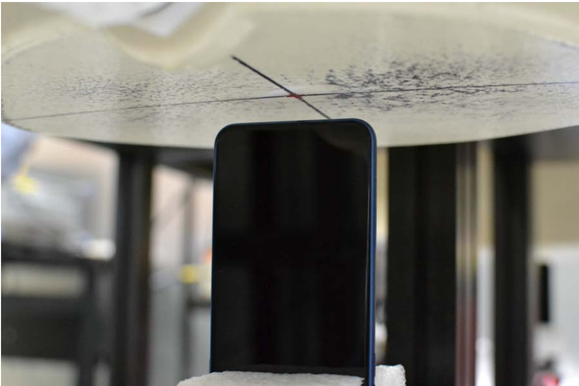
SAR Test Setup Photo 8: Bottom at 1.0 cm
