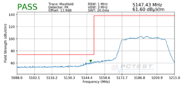
Plot 7-93. Radiated Lower Band Edge Plot (Peak – UNII Band 1)
