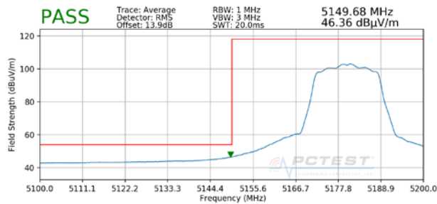
Plot 7-85. Radiated Lower Band Edge Plot (Average – UNII Band 1)
