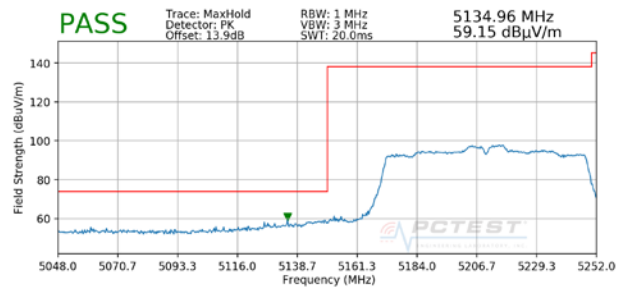
Plot 7-100. Radiated Lower Band Edge Plot (Peak – UNII Band 1)
