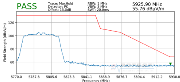
Plot 7-98. Radiated Upper Band Edge Plot (Peak - UNII Band 3)
