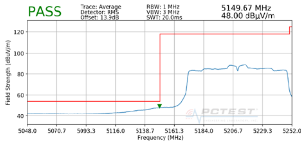
Plot 7-99. Radiated Lower Band Edge Plot (Average – UNII Band 1)
