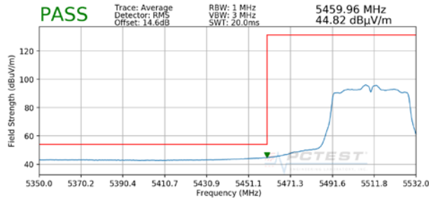
Plot 7-96. Radiated Lower Band Edge Plot (Average - UNII Band 2C)
