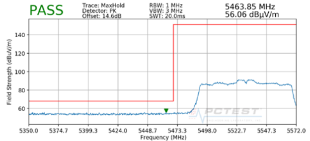
Plot 7-104. Radiated Lower Band Edge Plot (Peak – UNII Band 2C)
