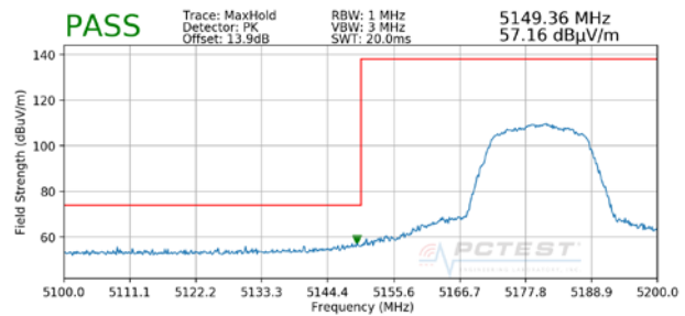
Plot 7-86. Radiated Lower Band Edge Plot (Peak – UNII Band 1)
