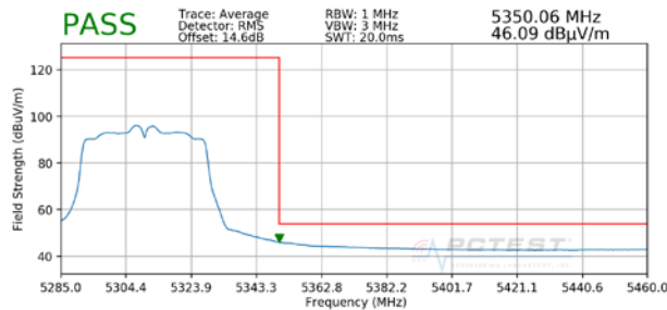
Plot 7-94. Radiated Upper Band Edge Plot (Average – UNII Band 2A)
