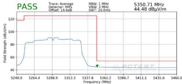
Plot 7-101. Radiated Upper Band Edge Plot (Average – UNII Band 2A)
