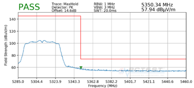
Plot 7-95. Radiated Upper Band Edge Plot (Peak – UNII Band 2A)
