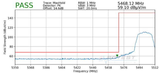
Plot 7-90. Radiated Lower Band Edge Plot (Peak - UNII Band 2C)
