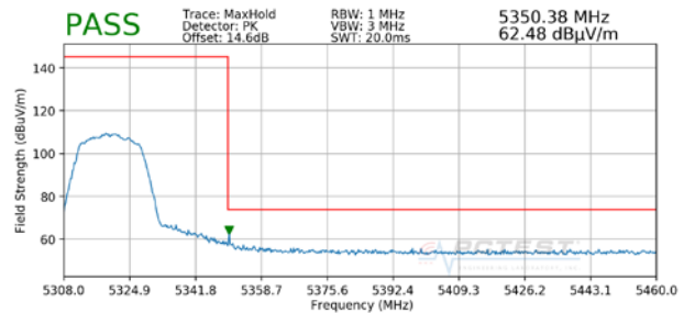
Plot 7-88. Radiated Upper Band Edge Plot (Peak – UNII Band 2A)
