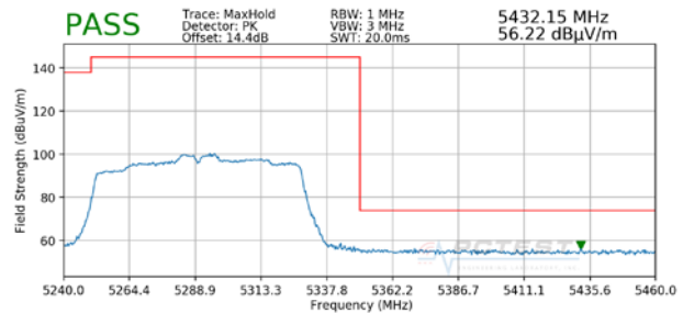
Plot 7-102. Radiated Upper Band Edge Plot (Peak – UNII Band 2A)
