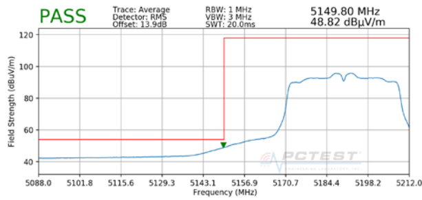
Plot 7-92. Radiated Lower Band Edge Plot (Average – UNII Band 1)
