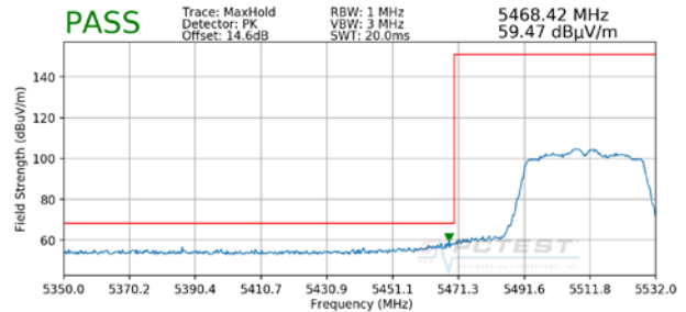
Plot 7-97. Radiated Lower Band Edge Plot (Peak - UNII Band 2C)
