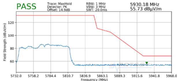
Plot 7-105. Radiated Upper Band Edge Plot (Peak – UNII Band 3)
