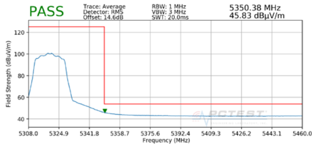
Plot 7-87. Radiated Upper Band Edge Plot (Average – UNII Band 2A)
