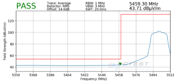
Plot 7-89. Radiated Lower Band Edge Plot (Average - UNII Band 2C)
