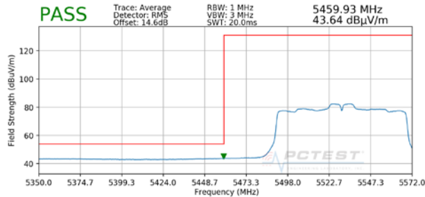
Plot 7-103. Radiated Lower Band Edge Plot (Average – UNII Band 2C)
