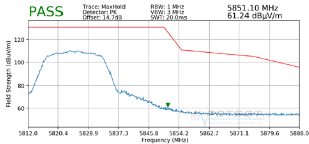
Plot 7-91. Radiated Upper Band Edge Plot (Peak - UNII Band 3)
