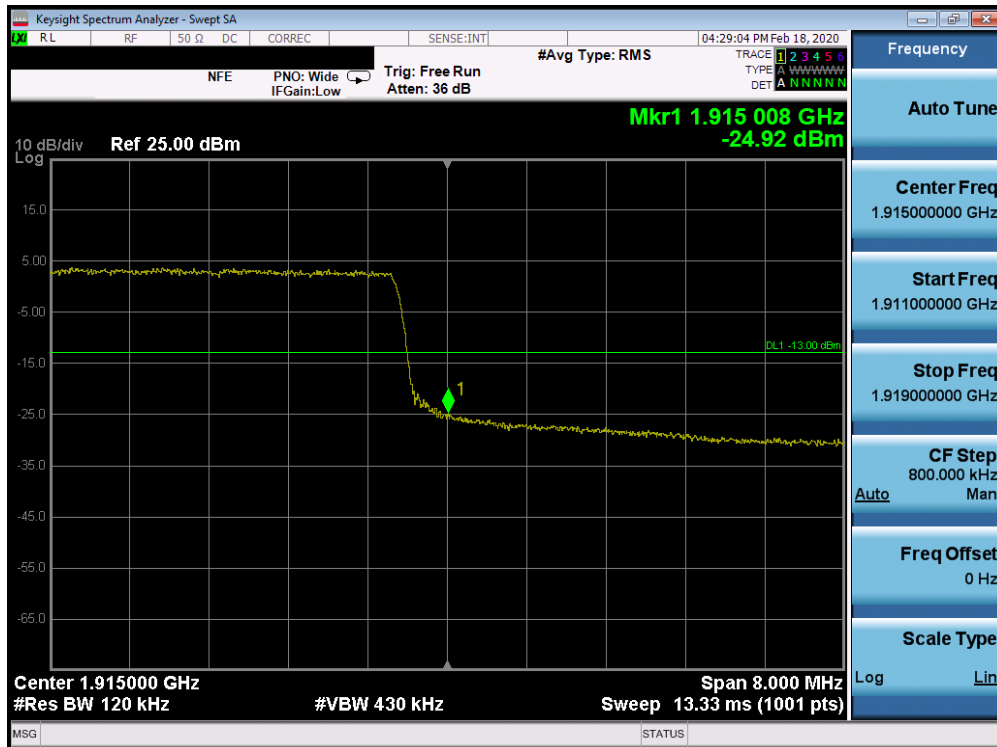
Plot 7-192. Upper Band Edge Plot (Band 25 - 10.0MHz QPSK - Full RB Configuration)
