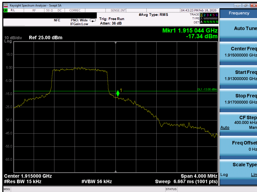
Plot 7-174. Upper Band Edge Plot (Band 25 - 1.4MHz QPSK - Full RB Configuration)
