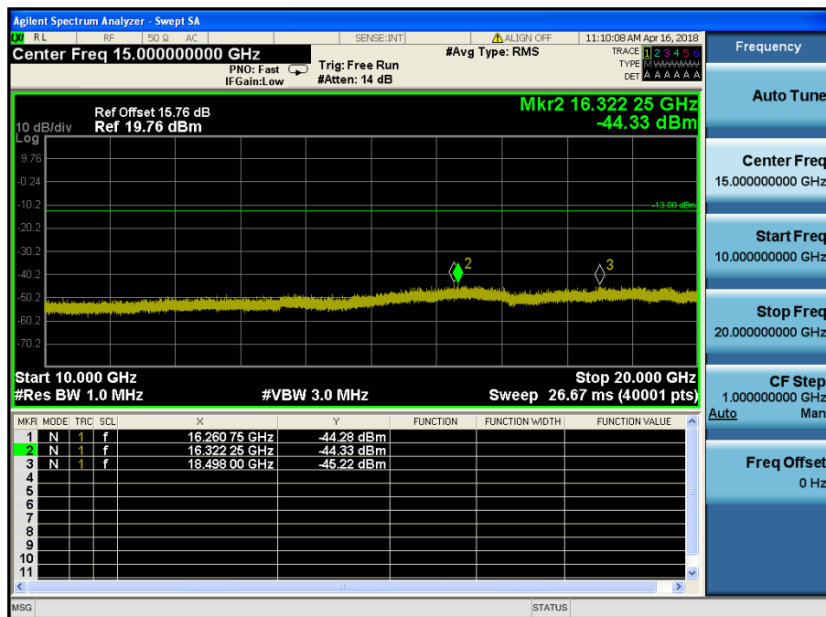
LTE Band 66 / 3MHz / 16QAM - RB Size/Offset (1/0) – Mid Channel
