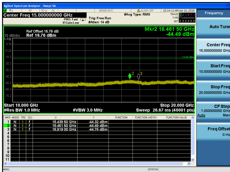
LTE Band 66 / 1.4MHz / 16QAM - RB Size/Offset (1/5) – Low Channel
