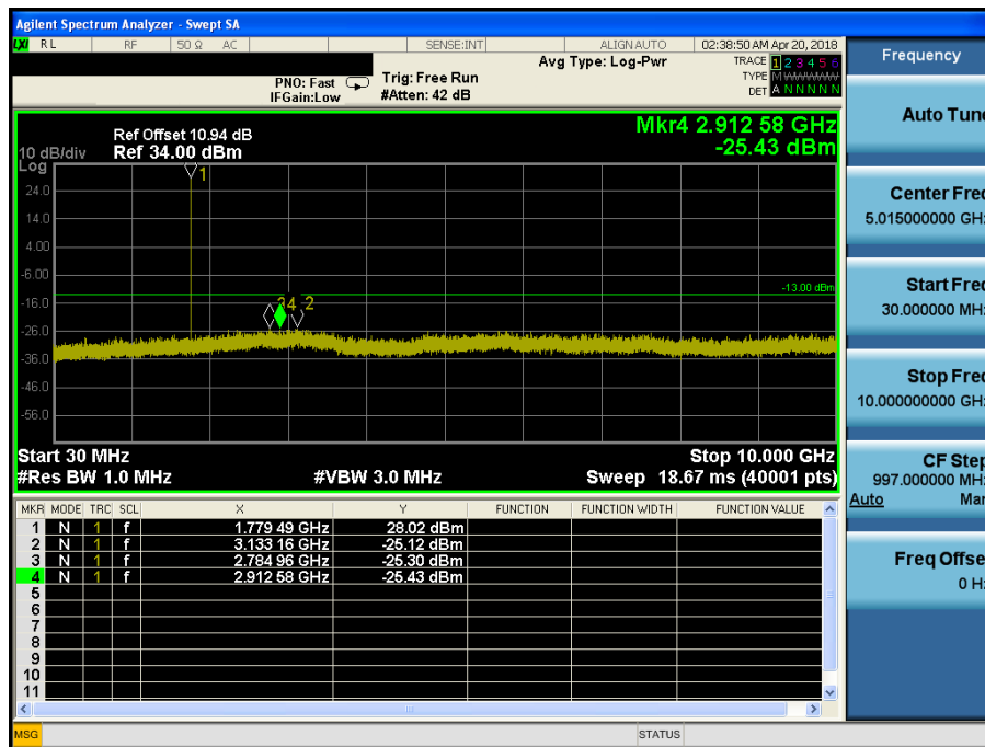
LTE Band 66 / 1.4MHz / 16QAM - RB Size/Offset (1/2) – High Channel
