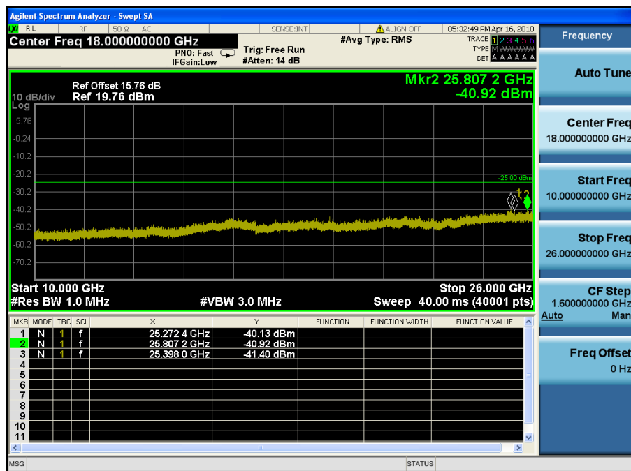
LTE Band 7 / 5MHz / 16QAM - RB Size/Offset (12/13) – Low Channel
