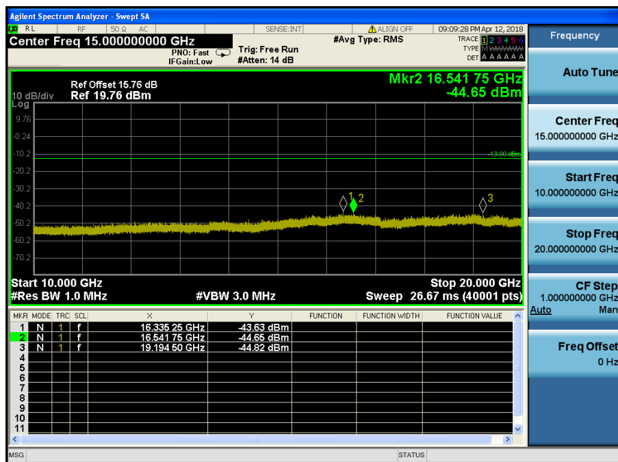
LTE Band 2 / 20MHz / QPSK - RB Size/Offset (1/50)–Mid Channel
