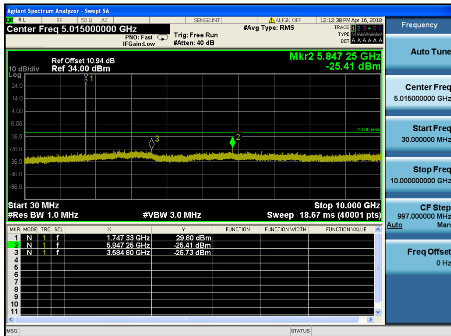
LTE Band 66 / 5MHz / 16QAM - RB Size/Offset (1/24) – Mid Channel
