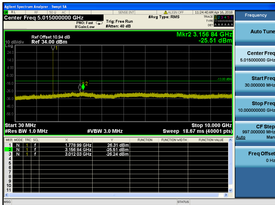
LTE Band 66 / 3MHz / 16QAM - RB Size/Offset (8/4) – High Channel
