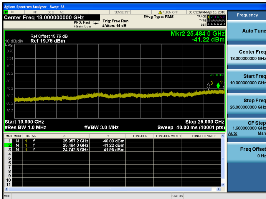
LTE Band 7 / 10MHz / 16QAM - RB Size/Offset (1/49) – Mid Channel
