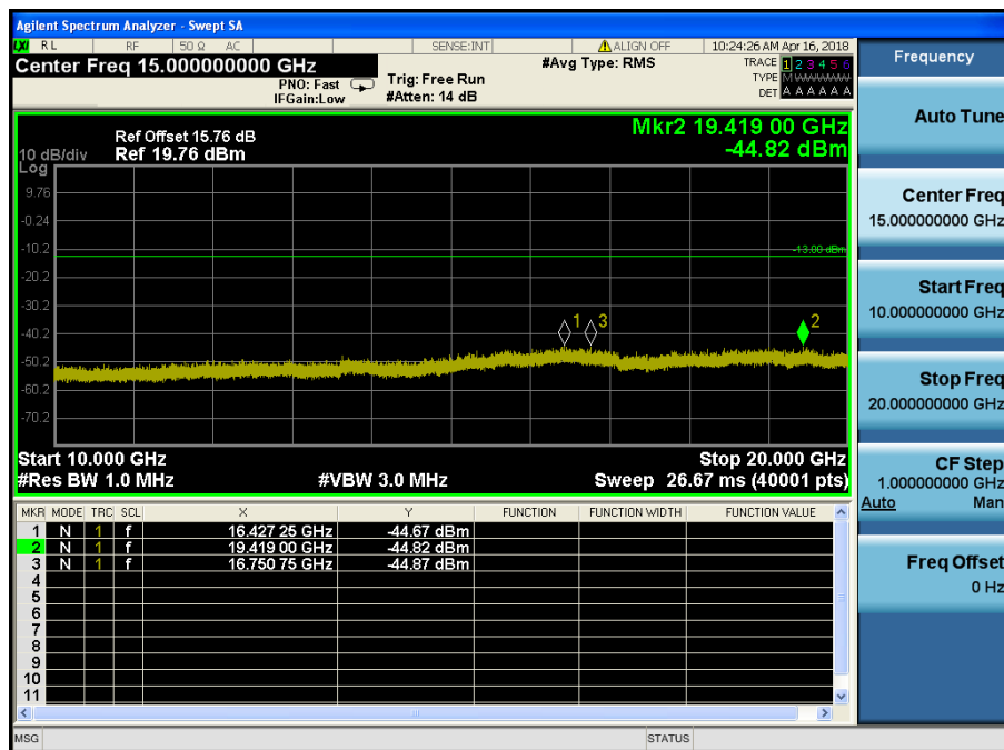
LTE Band 66 / 1.4MHz / 16QAM - RB Size/Offset (1/0) – Mid Channel
