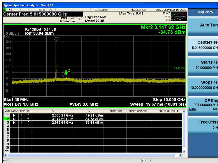
LTE Band 7 / 20MHz / QPSK - RB Size/Offset (50/0) – High Channel
