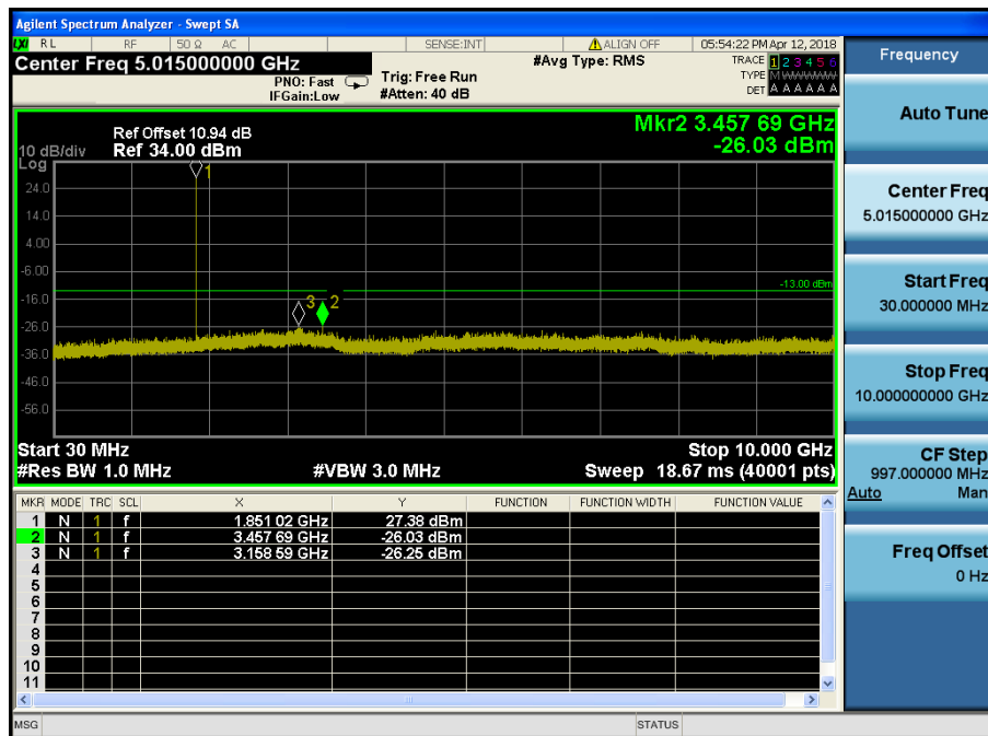
LTE Band 2 / 1.4MHz / QPSK - RB Size/Offset (3/2) – Low Channel
