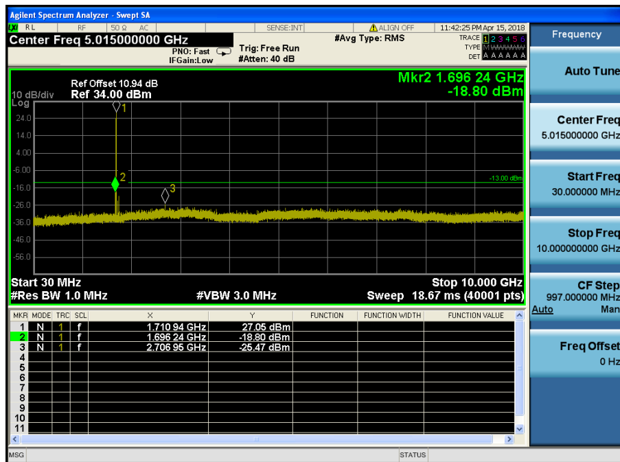
LTE Band 66 / 3MHz / QPSK - RB Size/Offset (8/0) – Low Channel
