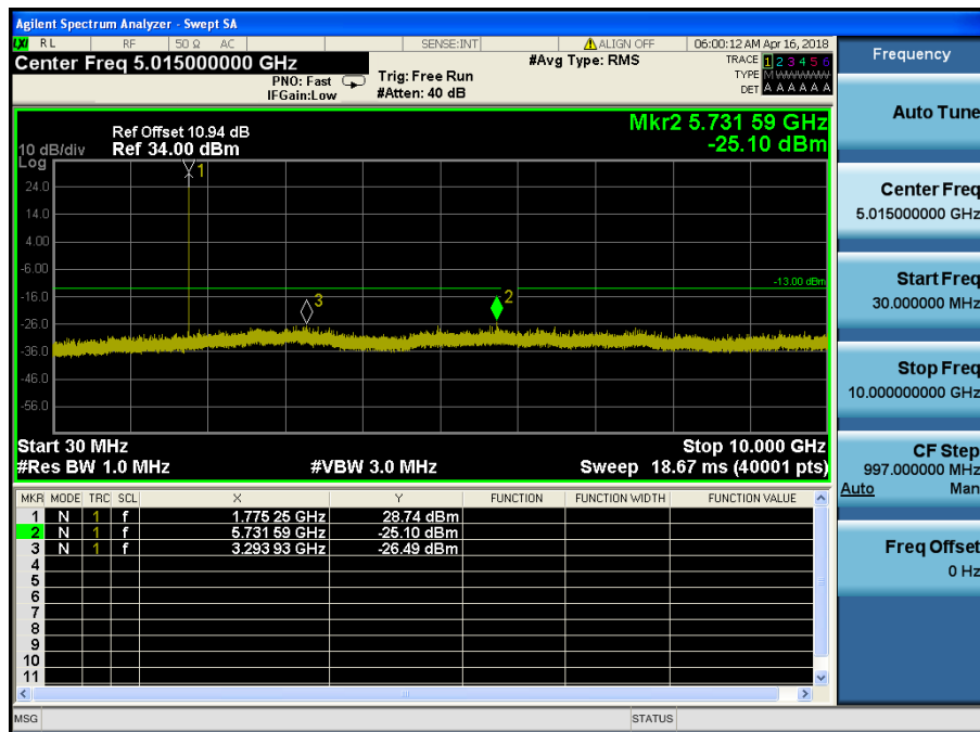
LTE Band 66 / 10MHz / QPSK - RB Size/Offset (1/25) – High Channel
