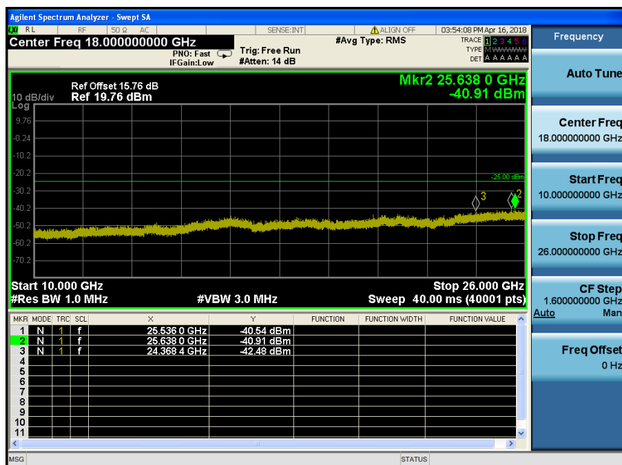
LTE Band 7 / 5MHz / QPSK - RB Size/Offset (12/13) – Mid Channel
