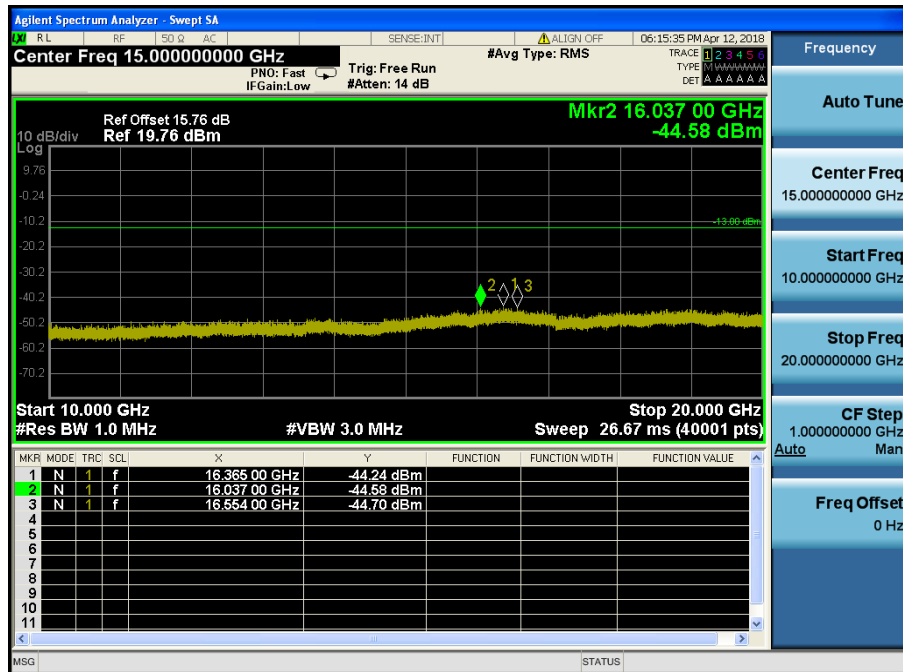
LTE Band 2 / 1.4MHz / QPSK - RB Size/Offset (3/2) – High Channel
