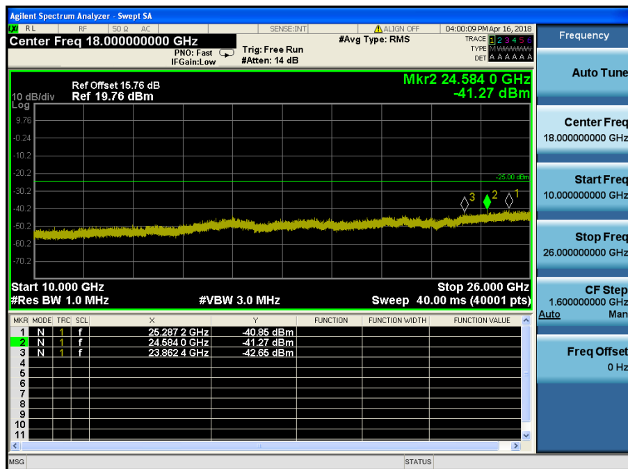
LTE Band 7 / 5MHz / QPSK - RB Size/Offset (12/0) – High Channel
