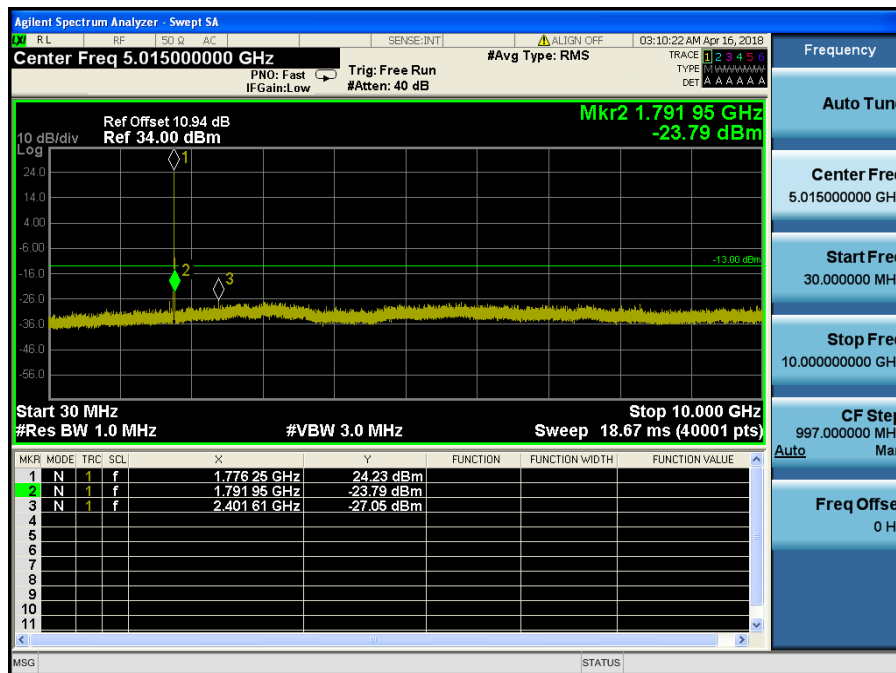
LTE Band 66 / 5MHz / QPSK - RB Size/Offset (25/0) – High Channel
