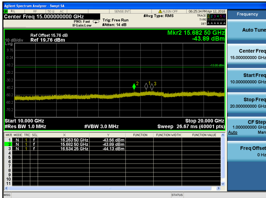
LTE Band 2 / 3MHz / QPSK - RB Size/Offset (1/7) – Low Channel
