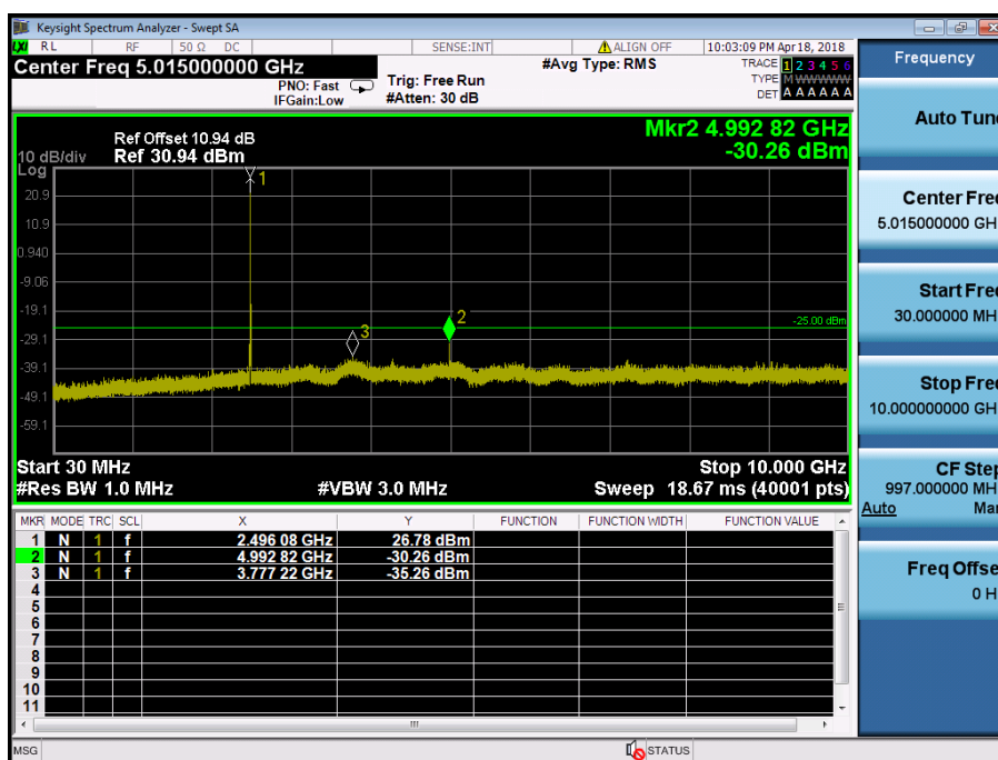
LTE Band 41 / 5MHz / 16QAM - RB Size/Offset (1/0) – Low Channel
