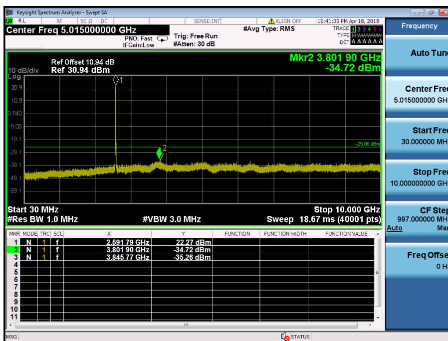
LTE Band 41 / 15MHz / 16QAM - RB Size/Offset (1/74) – Mid Channel
