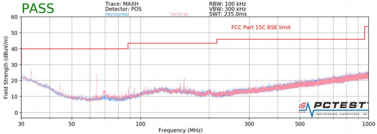
Plot 7-39. Radiated Spurious Plot below 1GHz
