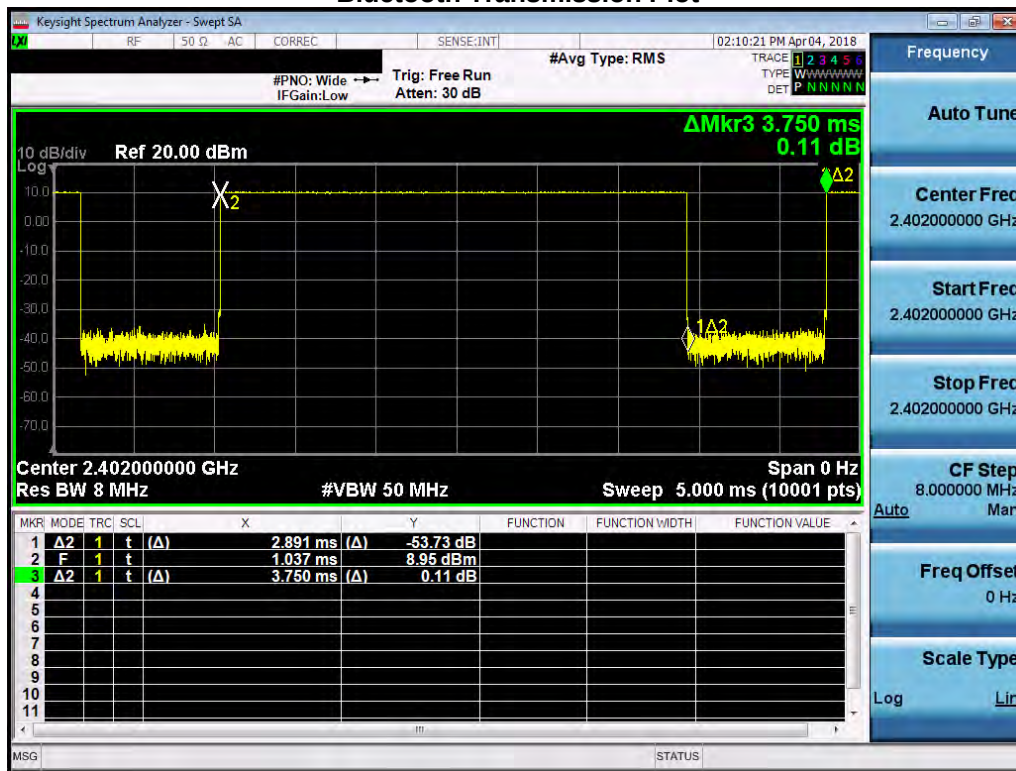
Bluetooth Transmission Plot
