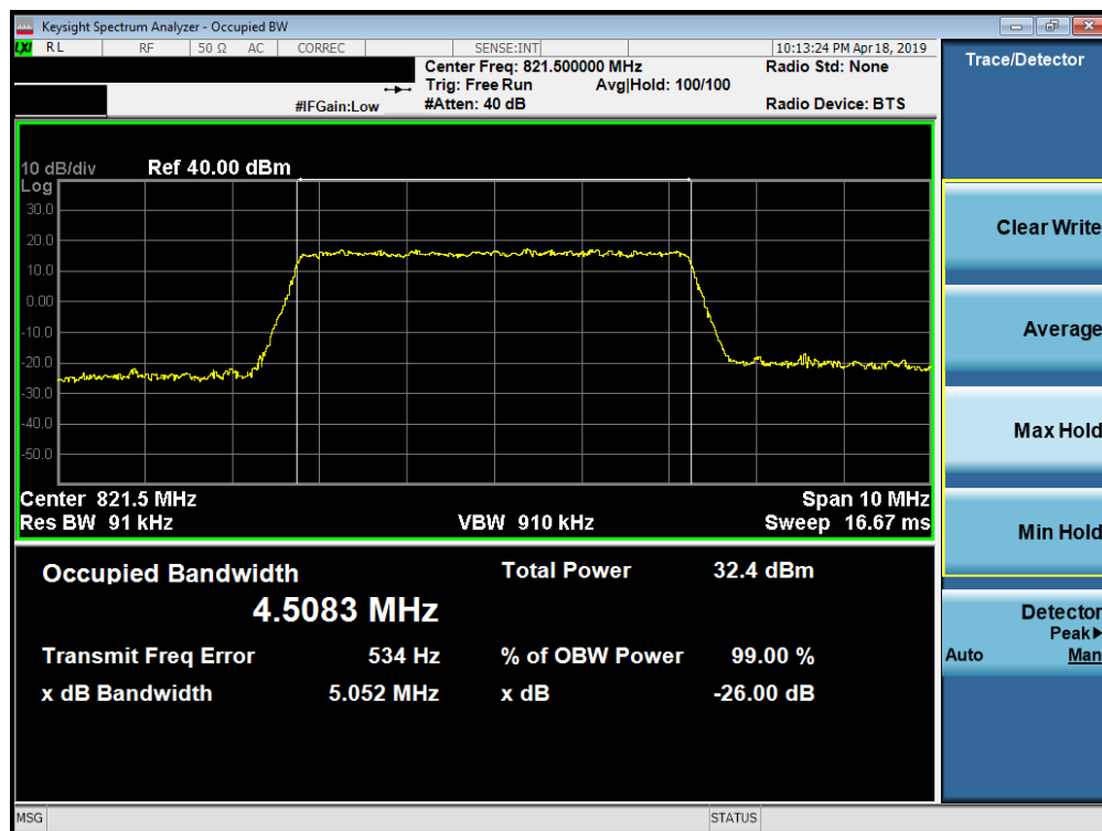
Plot 7-11. Occupied Bandwidth Plot (LTE Band 26, 5MHz 64-QAM – RB Size 25– High Channel)
