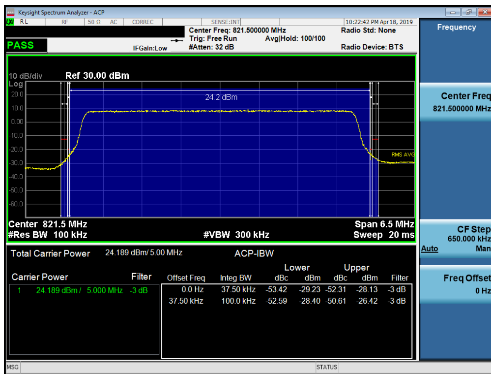
Plot 7-37. Channel Edge Plot (LTE Band 26, 5MHz QPSK – RB Size 25 – High Channel)
