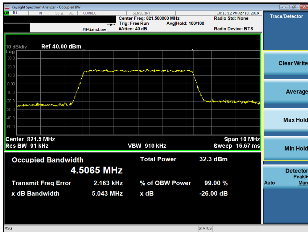
Plot 7-10. Occupied Bandwidth Plot (LTE Band 26, 5MHz 16-QAM – RB Size 25– High Channel)
