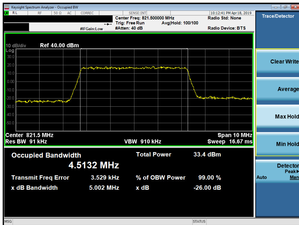
Plot 7-9. Occupied Bandwidth Plot (LTE Band 26, 5MHz QPSK – RB Size 25– High Channel)
