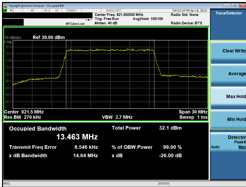
Plot 7-15. Occupied Bandwidth Plot (LTE Band 26, 15MHz QPSK – RB Size 75)
