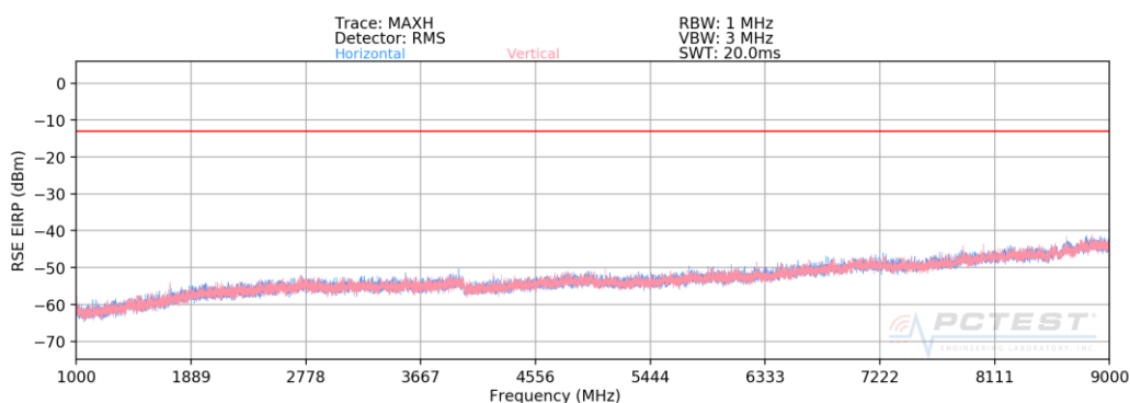
Plot 7-2. Radiated Spurious Plot above 1GHz (BC10 CDMA Mode)
