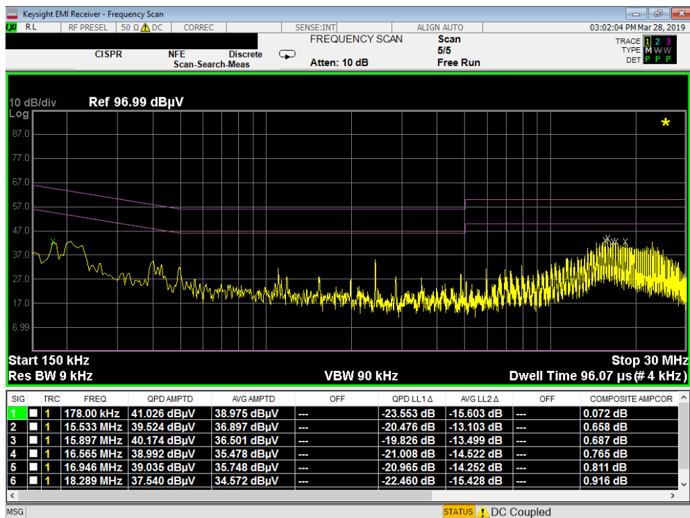
Plot 7-120. Line Conducted Plot with 802.11a UNII Band 2A (N)
