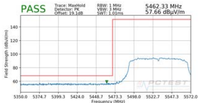
Plot 7-113. Radiated Lower Band Edge Plot (Peak – UNII Band 2C)
