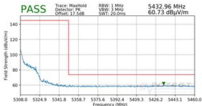
Plot 7-88. Radiated Upper Band Edge Plot (Peak - UNII Band 2A)
