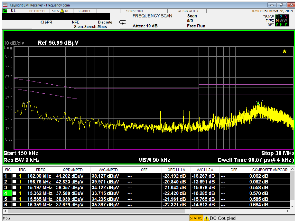
Plot 7-121. Line Conducted Plot with 802.11a UNII Band 2C (L1)
