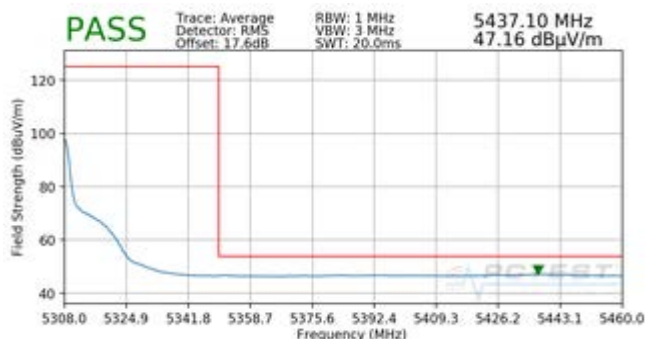
Plot 7-87. Radiated Upper Band Edge Plot (Average - UNII Band 2A)
