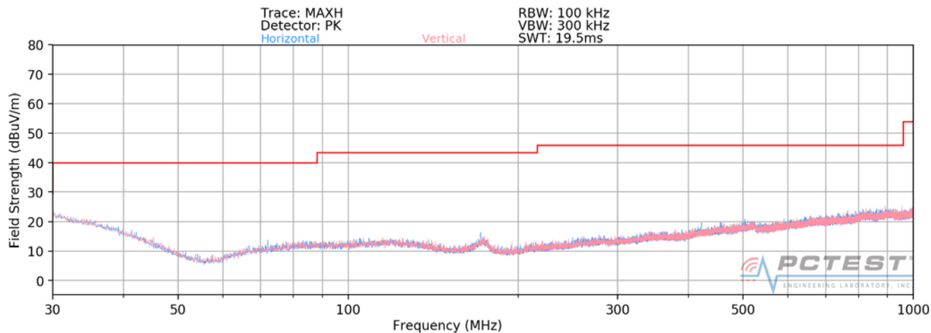
Plot 7-116. Radiated Spurious Plot below 1GHz (802.11a – U3 Ch. 157)
