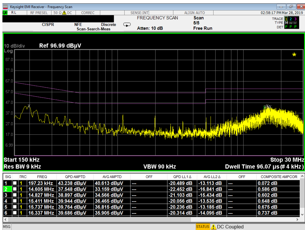
Plot 7-118. Line Conducted Plot with 802.11a UNII Band 1 (N)
