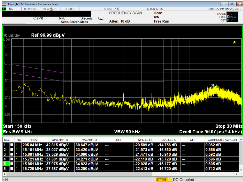
Plot 7-123. Line Conducted Plot with 802.11a UNII Band 3 (L1)
