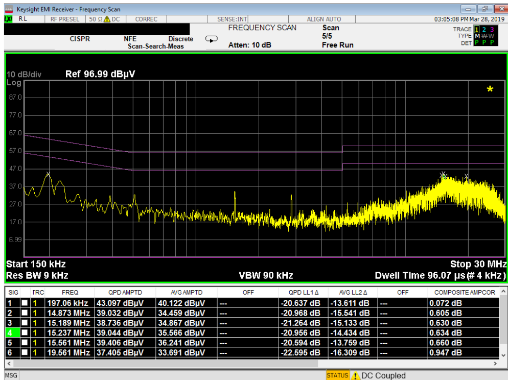
Plot 7-122. Line Conducted Plot with 802.11a UNII Band 2C (N)
