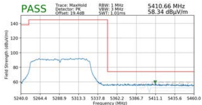
Plot 7-111. Radiated Upper Band Edge Plot (Peak - UNII Band 2A)
