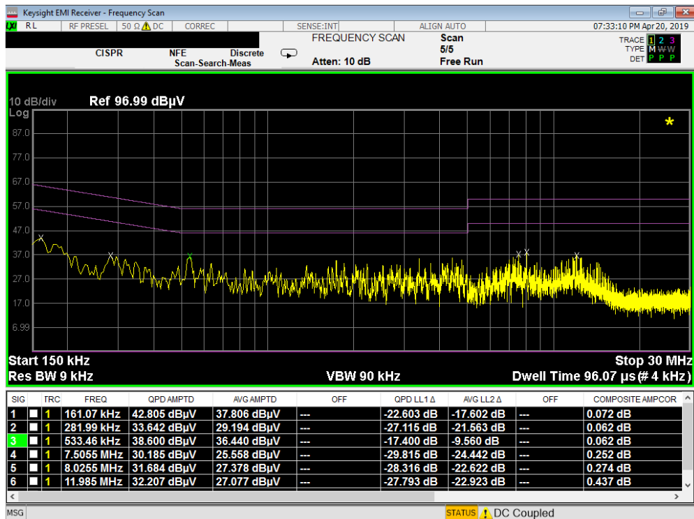
Plot 7-124. Line Conducted Plot with 802.11a UNII Band 3 (N)
