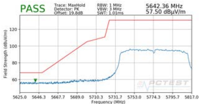
Plot 7-114. Radiated Lower Band Edge Plot (Peak – UNII Band 3)
