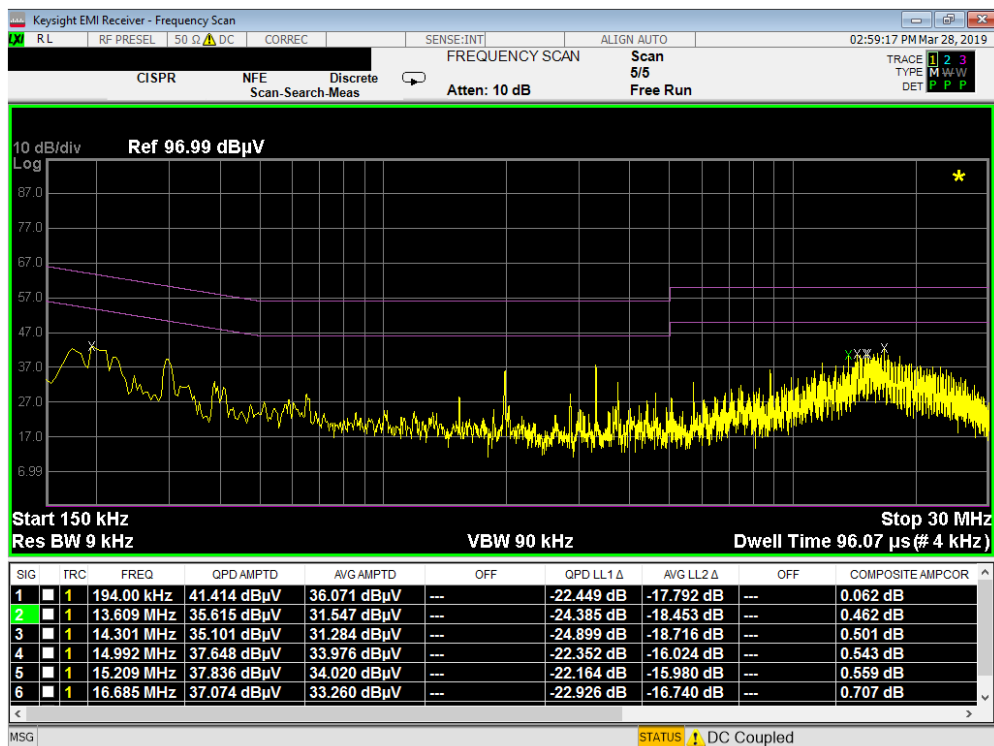
Plot 7-117. Line Conducted Plot with 802.11a UNII Band 1 (L1)
