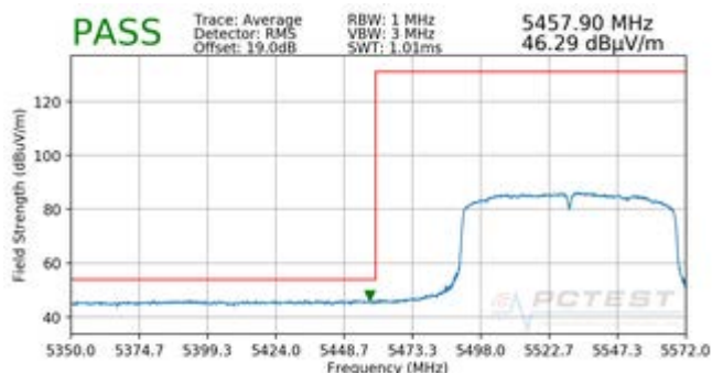
Plot 7-112. Radiated Lower Band Edge Plot (Average – UNII Band 2C)
