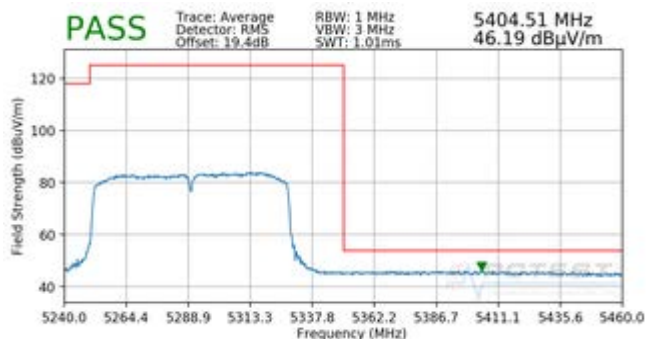
Plot 7-110. Radiated Upper Band Edge Plot (Average - UNII Band 2A)
