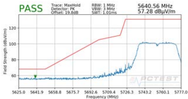
Plot 7-106. Radiated Lower Band Edge Plot (Peak – UNII Band 3)
