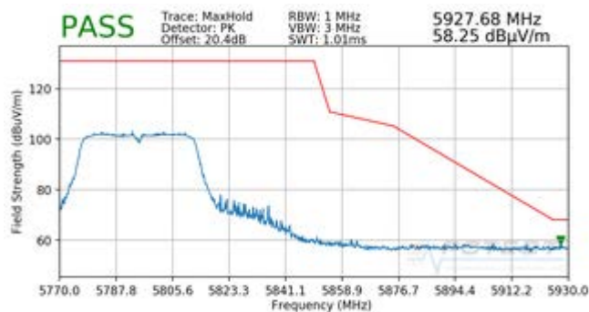
Plot 7-107. Radiated Upper Band Edge Plot (Peak – UNII Band 3)
