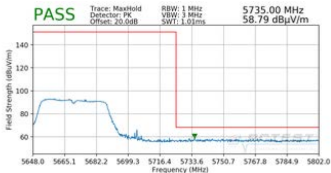
Plot 7-105. Radiated Upper Band Edge Plot (Peak – UNII Band 2C)
