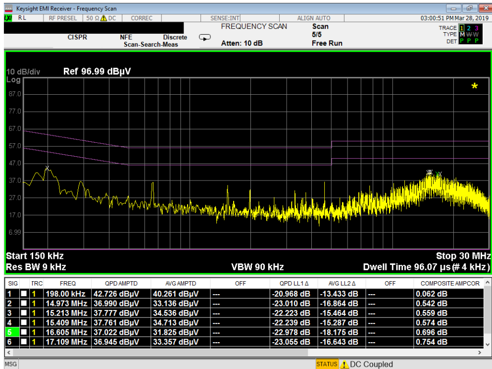
Plot 7-119. Line Conducted Plot with 802.11a UNII Band 2A (L1)
