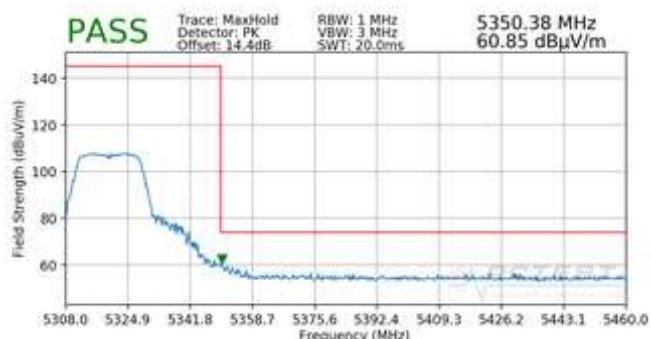
Plot 7-14. Radiated Upper Band Edge Plot (Peak – UNII Band 2A)
