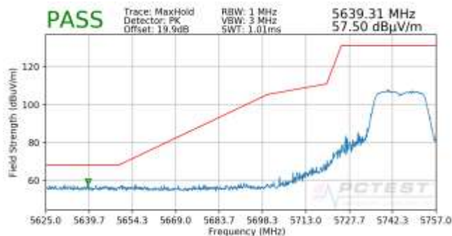
Plot 7-21. Radiated Upper Band Edge Plot (Peak – UNII Band 2C)
