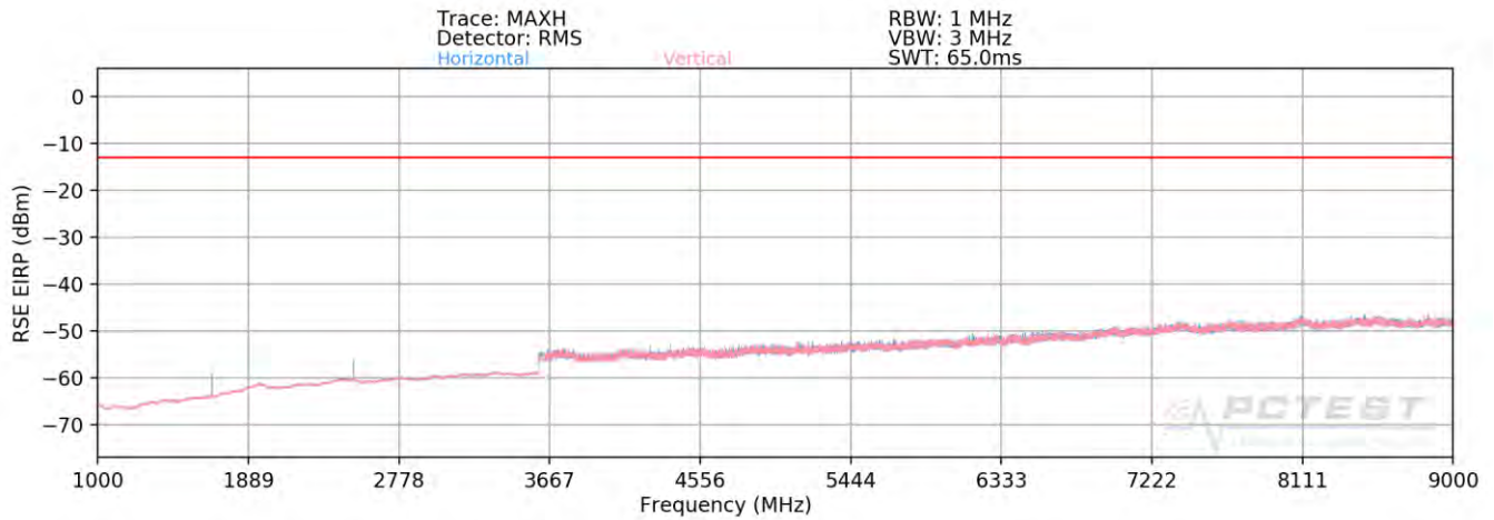
Plot 7-103. Radiated Spurious Emission Plot >1GHz (Cellular CDMA Mode)
