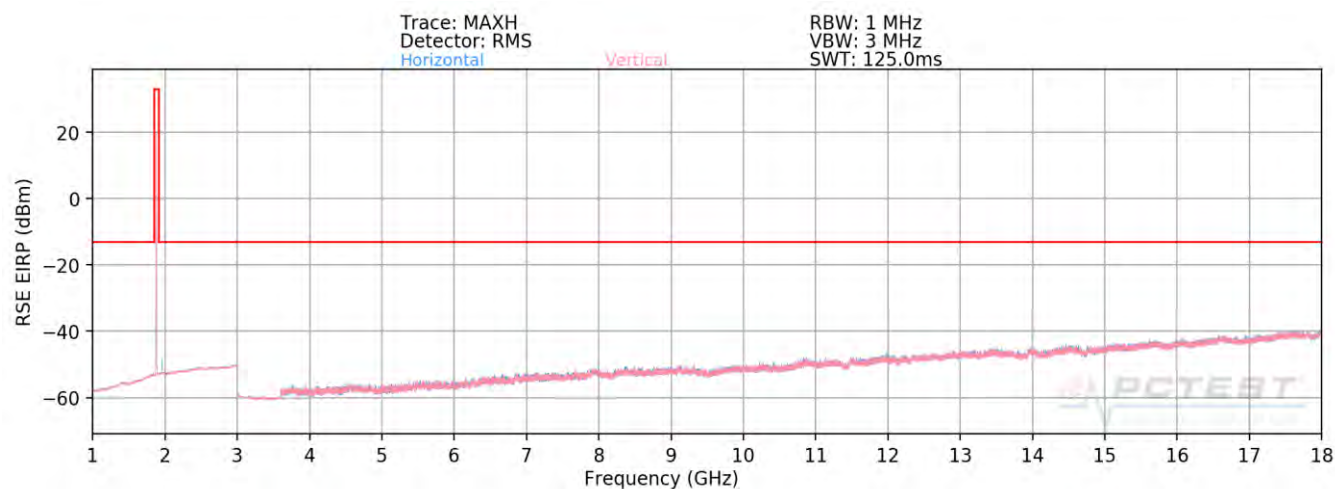
Plot 7-107. Radiated Spurious Emission Plot >1GHz (PCS CDMA Mode)
