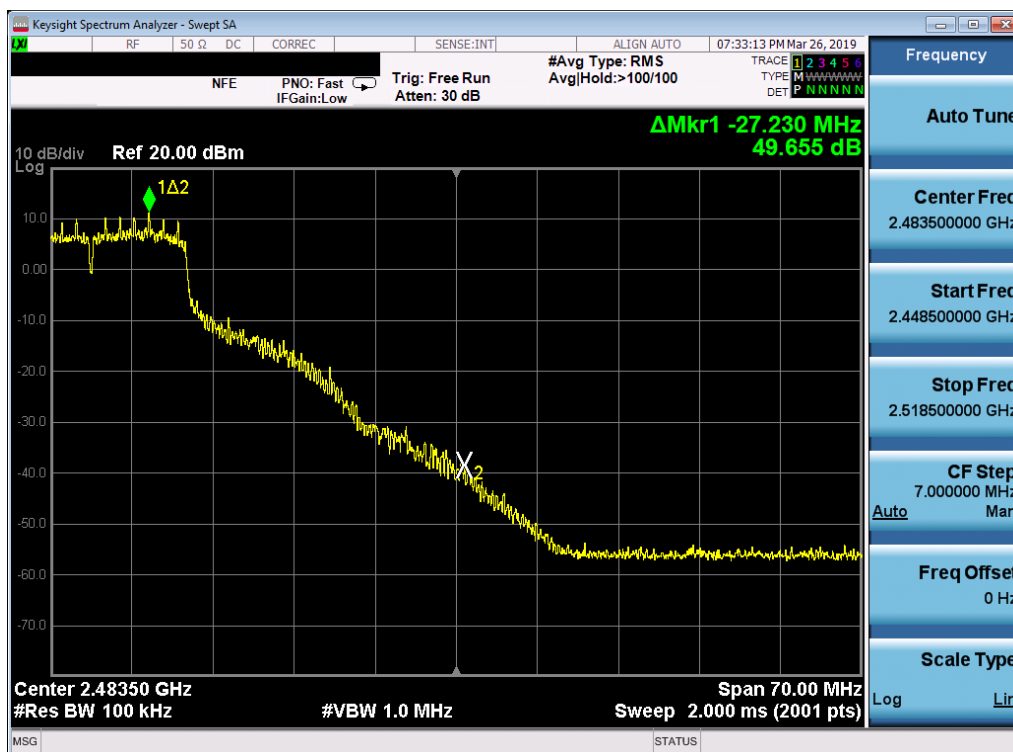
Plot 7-28. Band Edge Plot (802.11g – Ch. 9)
