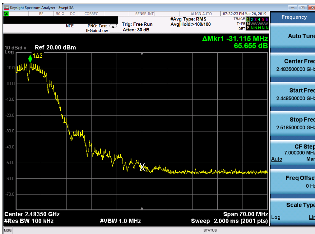
Plot 7-22. Band Edge Plot (802.11b – Ch. 9)
