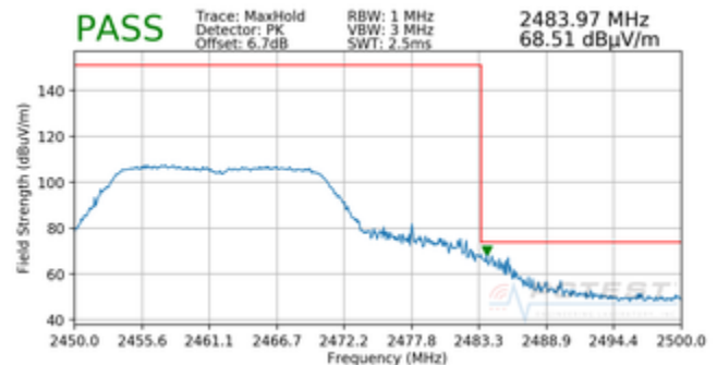
Plot 7-58. Radiated Restricted Upper Band Edge Measurement (Peak)
