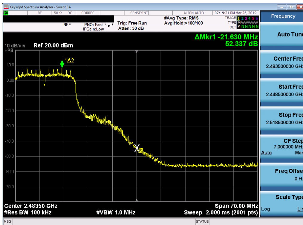
Plot 7-35. Band Edge Plot (802.11n (2.4GHz) – Ch. 10)
