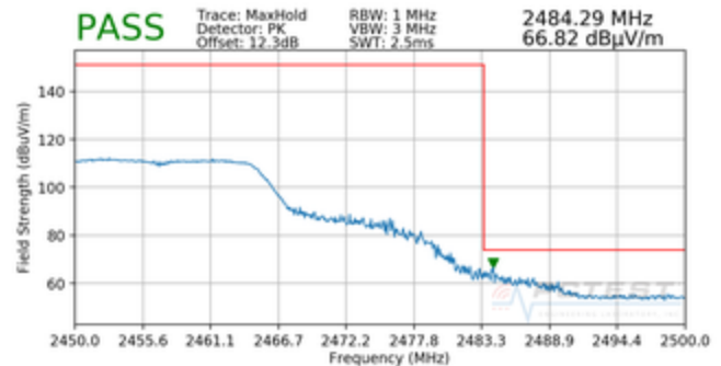
Plot 7-56. Radiated Restricted Upper Band Edge Measurement (Peak)
