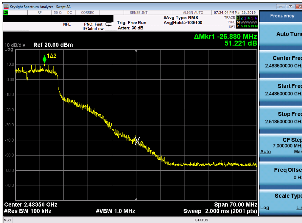
Plot 7-34. Band Edge Plot (802.11n (2.4GHz) – Ch. 9)
