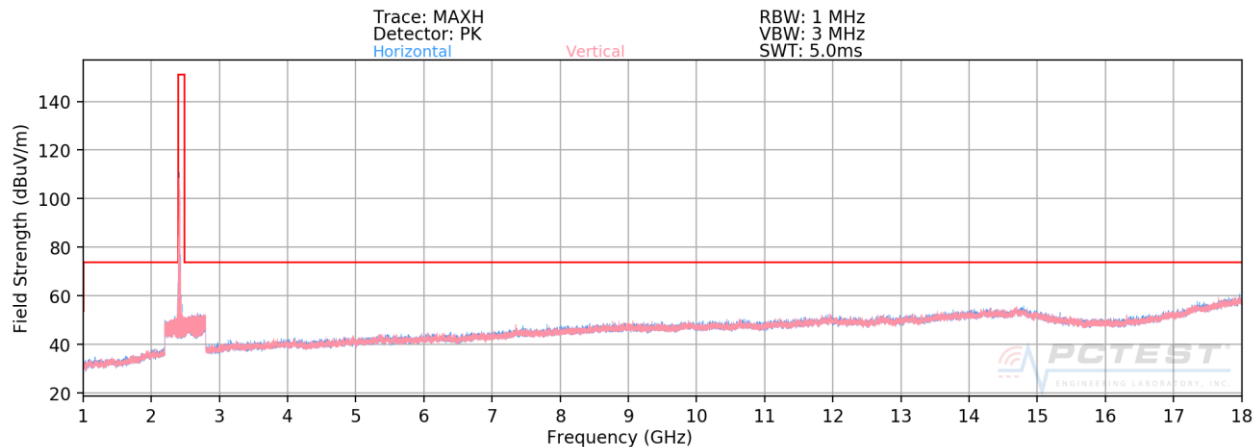
Plot 7-43. Radiated Spurious Plot above 1GHz (802.11b – Ch. 1)
