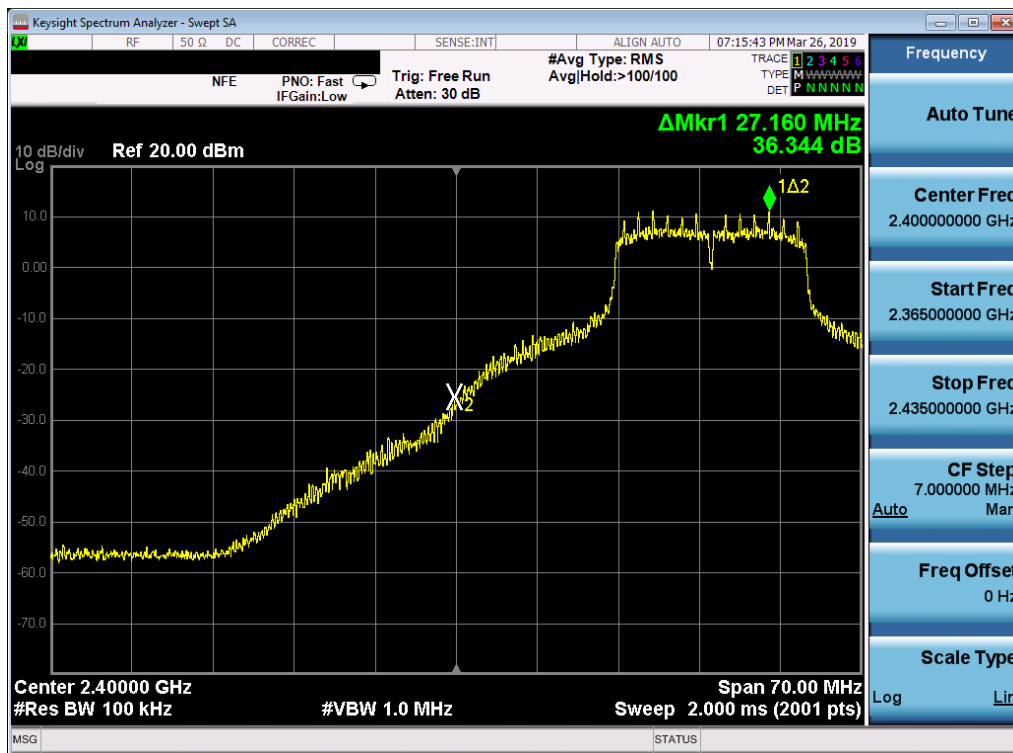
Plot 7-27. Band Edge Plot (802.11g– Ch. 3)
