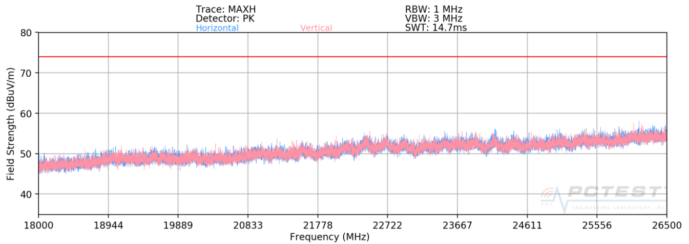
Plot 7-46. Radiated Spurious Plot above 18GHz ANT1
