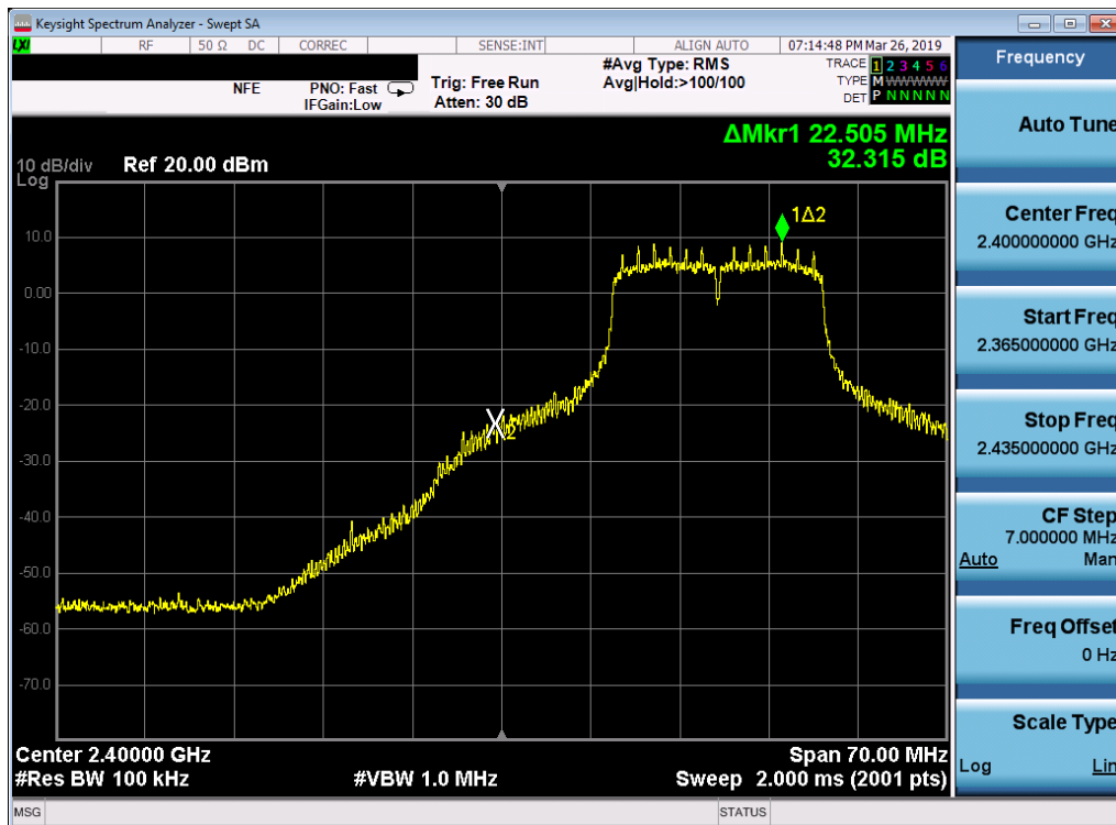
Plot 7-26. Band Edge Plot (802.11g– Ch. 2)
