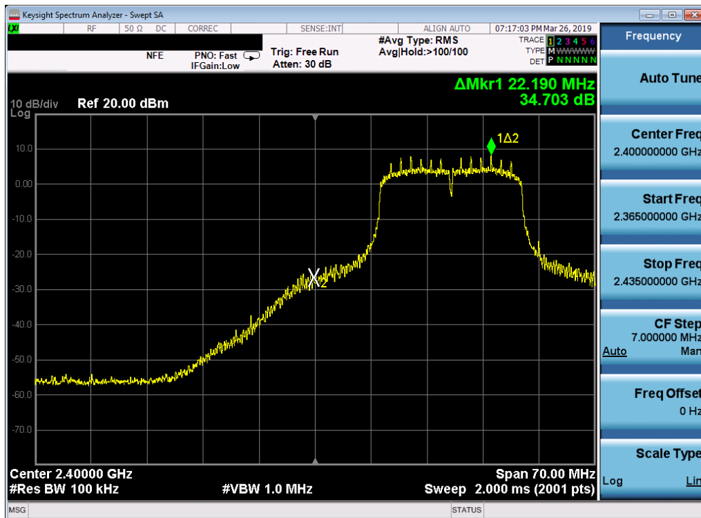
Plot 7-32. Band Edge Plot (802.11n (2.4GHz) – Ch. 2)
