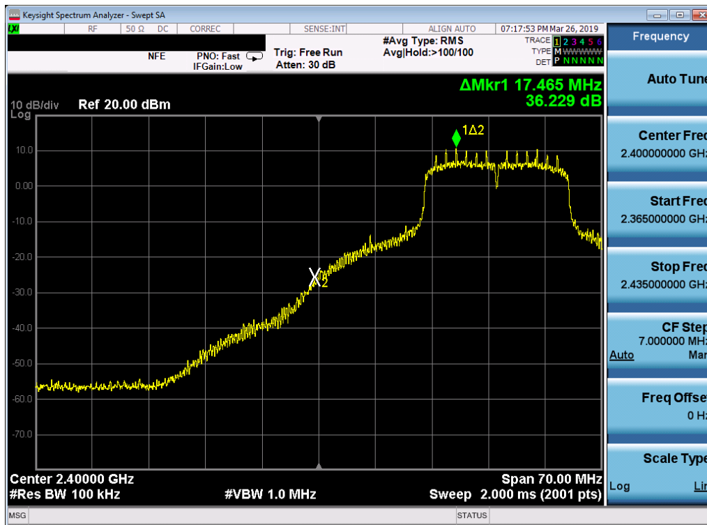
Plot 7-33. Band Edge Plot (802.11n (2.4GHz) – Ch. 3)
