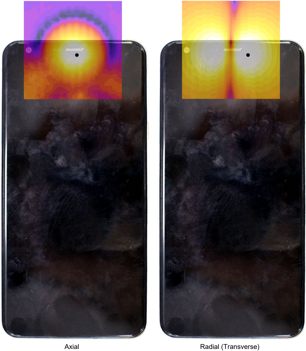
Figure 16-3 T-Coil Scan Overlay Magnetic Field Distributions
