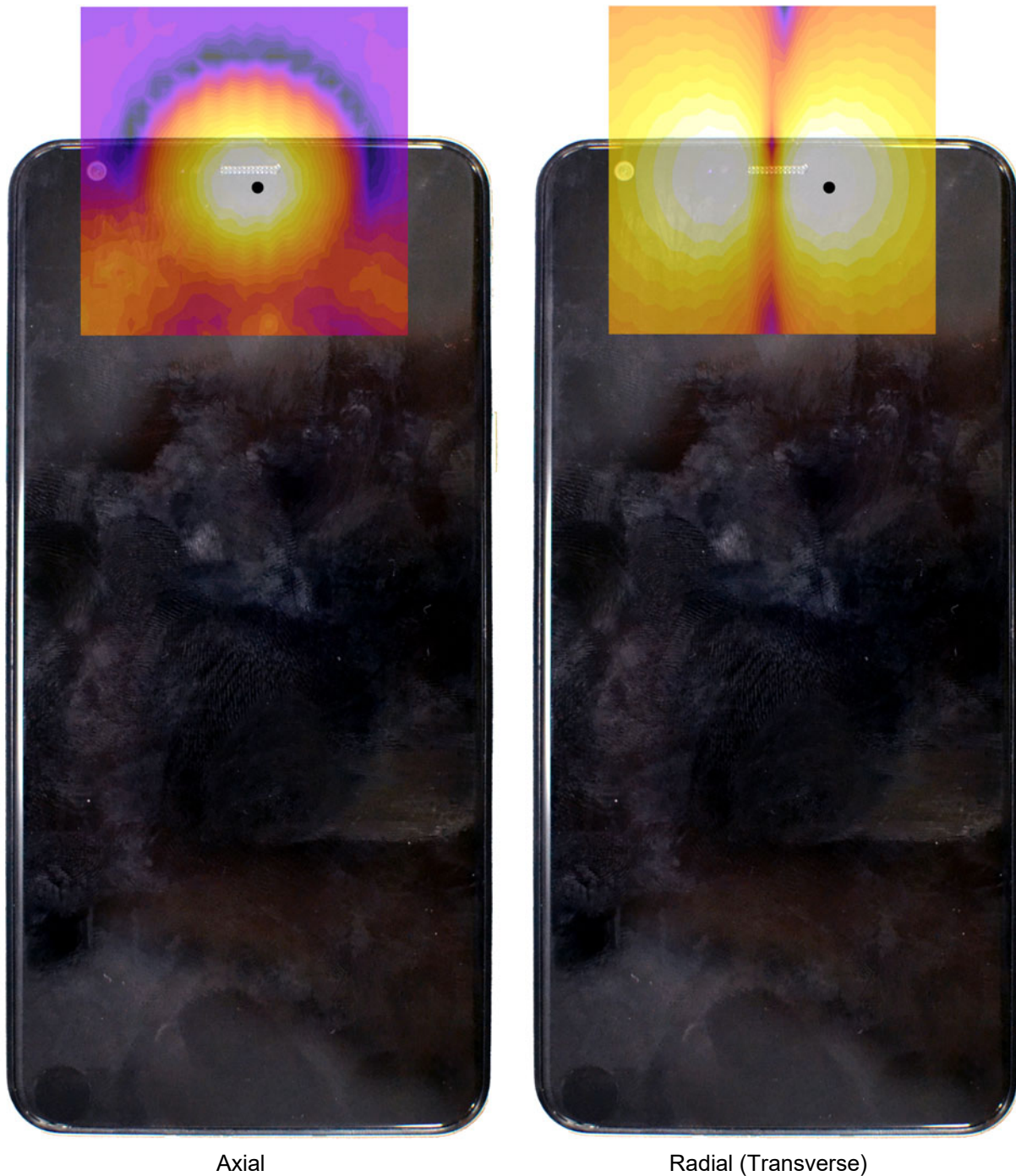
Figure 16-3 T-Coil Scan Overlay Magnetic Field Distributions
