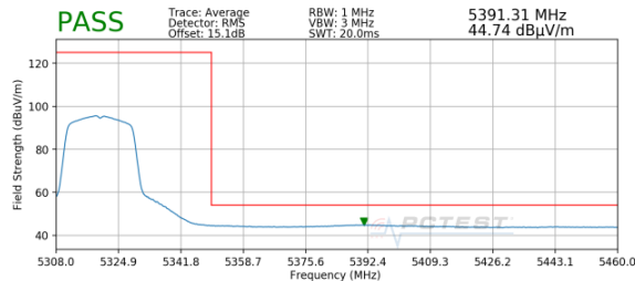
Plot 7-87. Radiated Upper Band Edge Plot (Average – UNII Band 2A)
