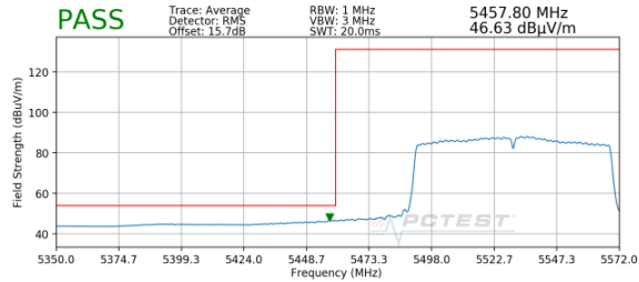
Plot 7-103. Radiated Lower Band Edge Plot (Average – UNII Band 2C)
