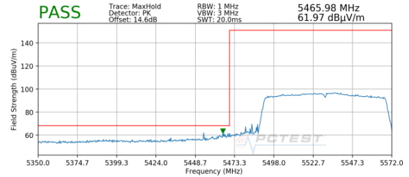
Plot 7-104. Radiated Lower Band Edge Plot (Peak – UNII Band 2C)
