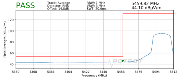
Plot 7-89. Radiated Lower Band Edge Plot (Average - UNII Band 2C)
