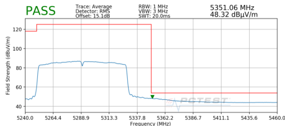
Plot 7-101. Radiated Upper Band Edge Plot (Average – UNII Band 2A)
