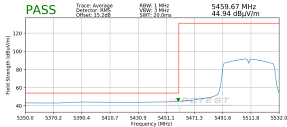
Plot 7-96. Radiated Lower Band Edge Plot (Average – UNII Band 2C)
