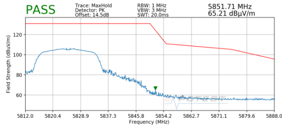
Plot 7-91. Radiated Upper Band Edge Plot (Peak - UNII Band 3)
