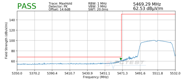
Plot 7-97. Radiated Lower Band Edge Plot (Peak – UNII Band 2C)
