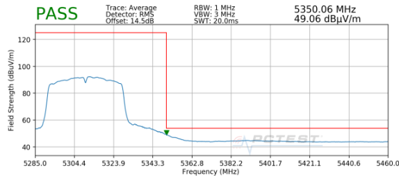
Plot 7-94. Radiated Upper Band Edge Plot (Average – UNII Band 2A)
