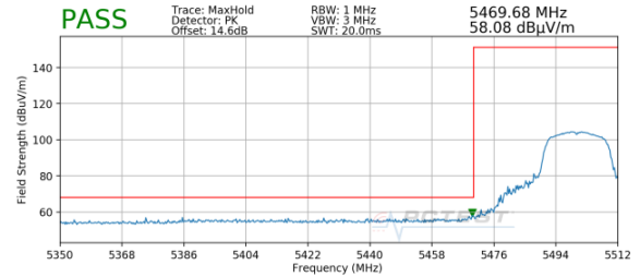
Plot 7-90. Radiated Lower Band Edge Plot (Peak - UNII Band 2C)
