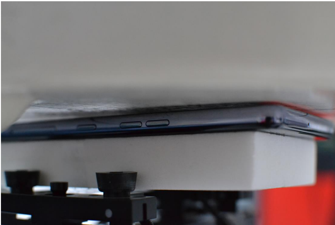
SAR Test Setup Photo 6 – Back Side at 1 mm
