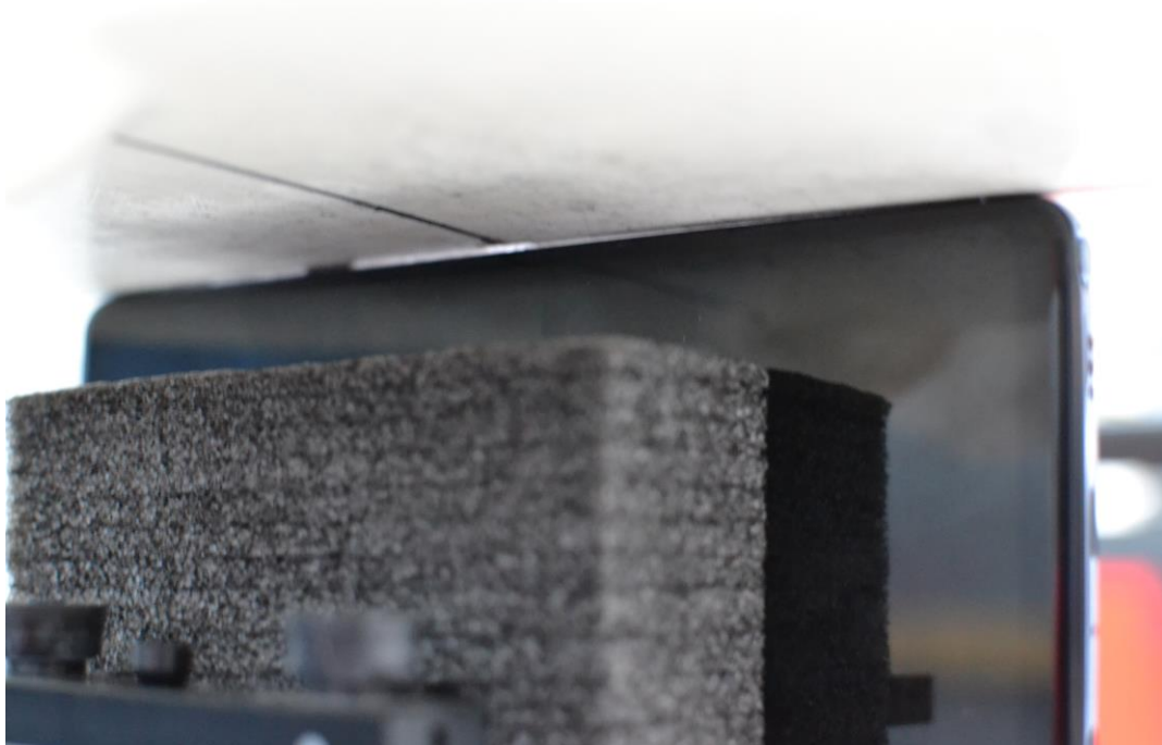
SAR Test Setup Photo 17 – Right Edge at 0 mm
