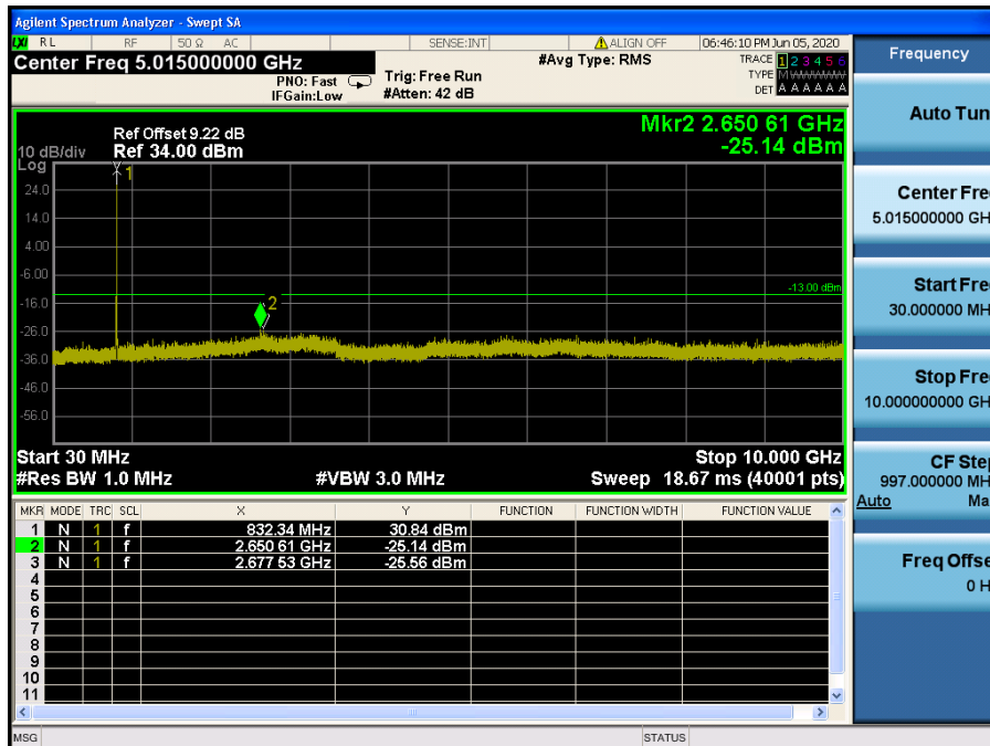
LTE Band 5 / 10 MHz / 64QAM - RB Size/Offset (1/0) – Mid Channel
