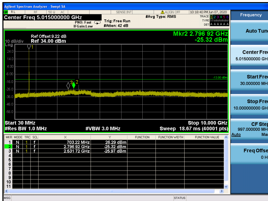
LTE Band 12, 17 / 10 MHz / QPSK - RB Size/Offset (25/12) – Low Channel
