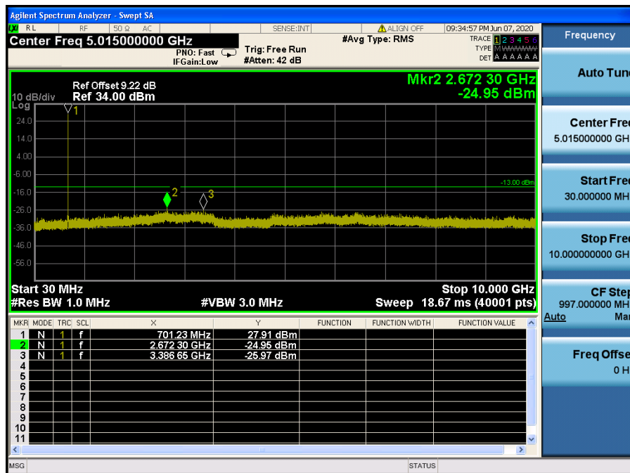
LTE Band 12, 17 / 5 MHz / QPSK - RB Size/Offset (12/6) – Low Channel
