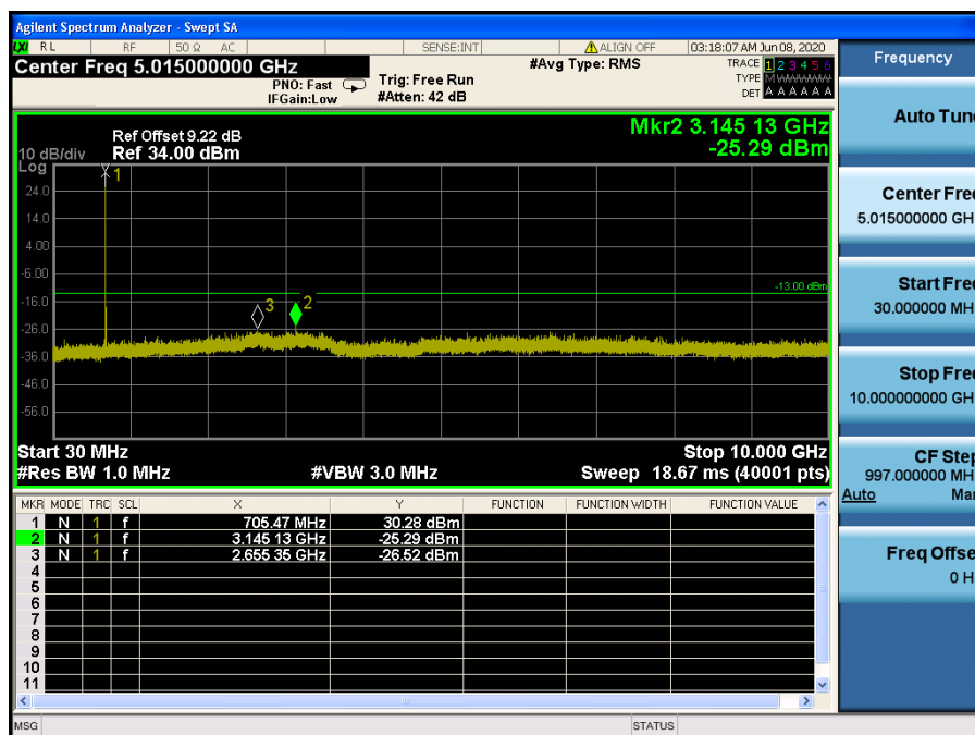
LTE Band 12, 17 / 5 MHz / 64QAM - RB Size/Offset (1/0) – Mid Channel
