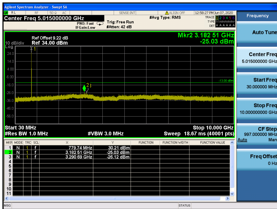
LTE Band 13 / 5 MHz / QPSK - RB Size/Offset (1/12) – Low Channel
