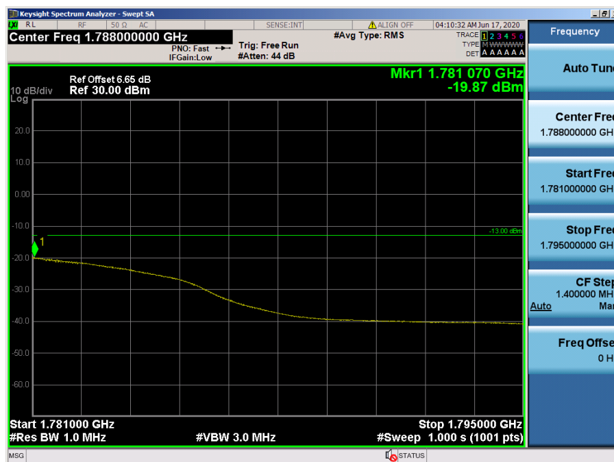
LTE Band 66, 4 / 15 MHz / QPSK - RB Size/Offset (36/39)
