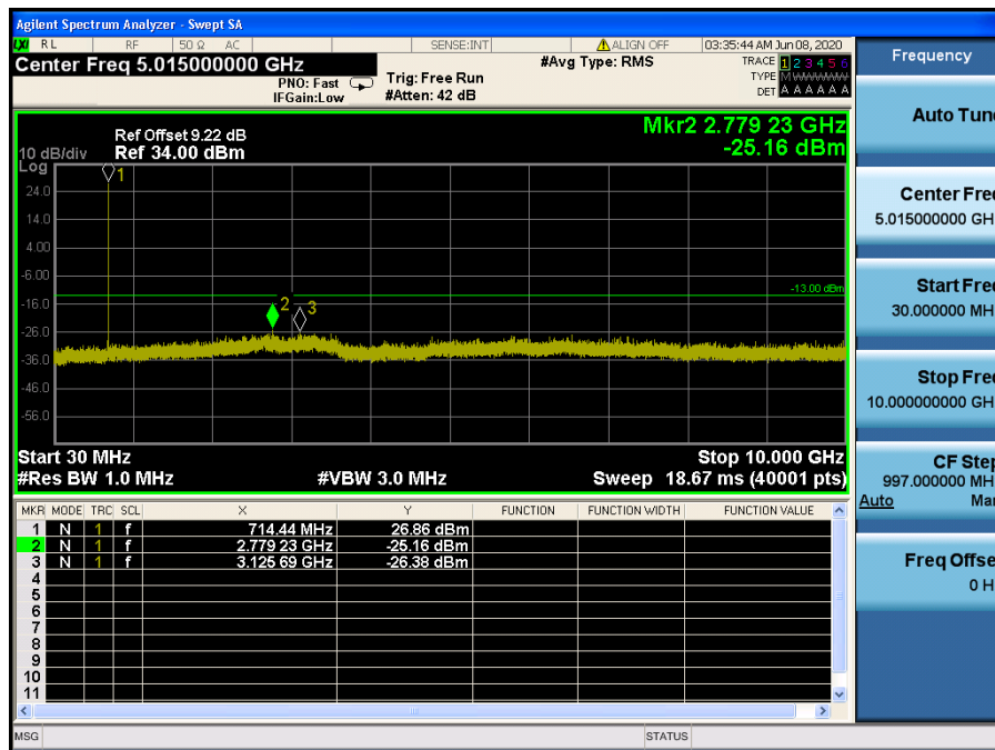
LTE Band 12, 17 / 5 MHz / 64QAM - RB Size/Offset (12/6) – High Channel
