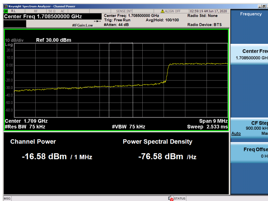
LTE Band 66, 4 / 10 MHz / QPSK - RB Size/Offset (50/0)
