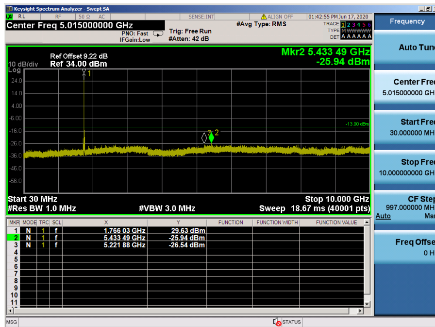
LTE Band 66, 4 / 15 MHz / 64QAM - RB Size/Offset (1/0) – High Channel
