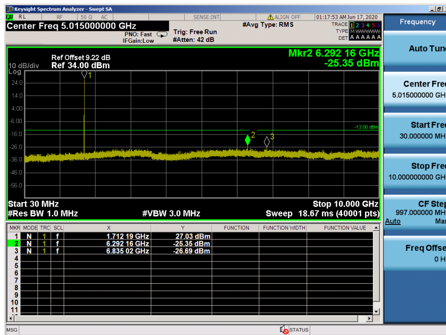
LTE Band 66, 4 / 3MHz / QPSK - RB Size/Offset (8/7) – Low Channel
