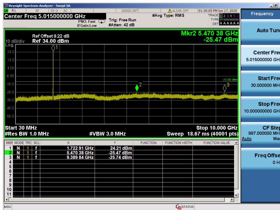
LTE Band 66, 4 / 15 MHz / 64QAM - RB Size/Offset (36/39) – Low Channel
