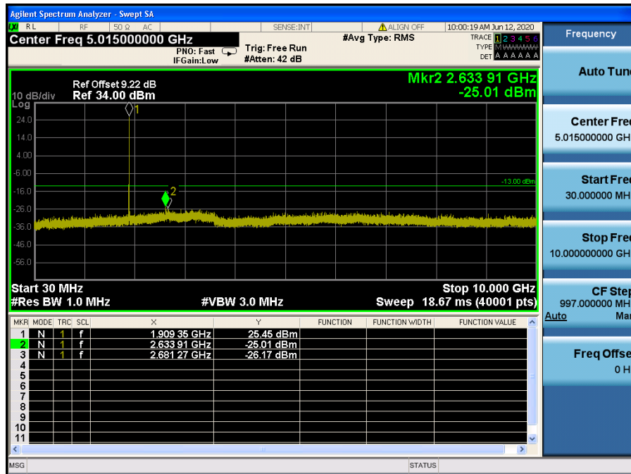
LTE Band 2 / 3MHz / 64QAM - RB Size/Offset (15/0) – High Channel
