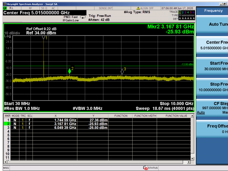
LTE Band 66, 4 / 5 MHz / 16QAM - RB Size/Offset (12/0) – Mid Channel
