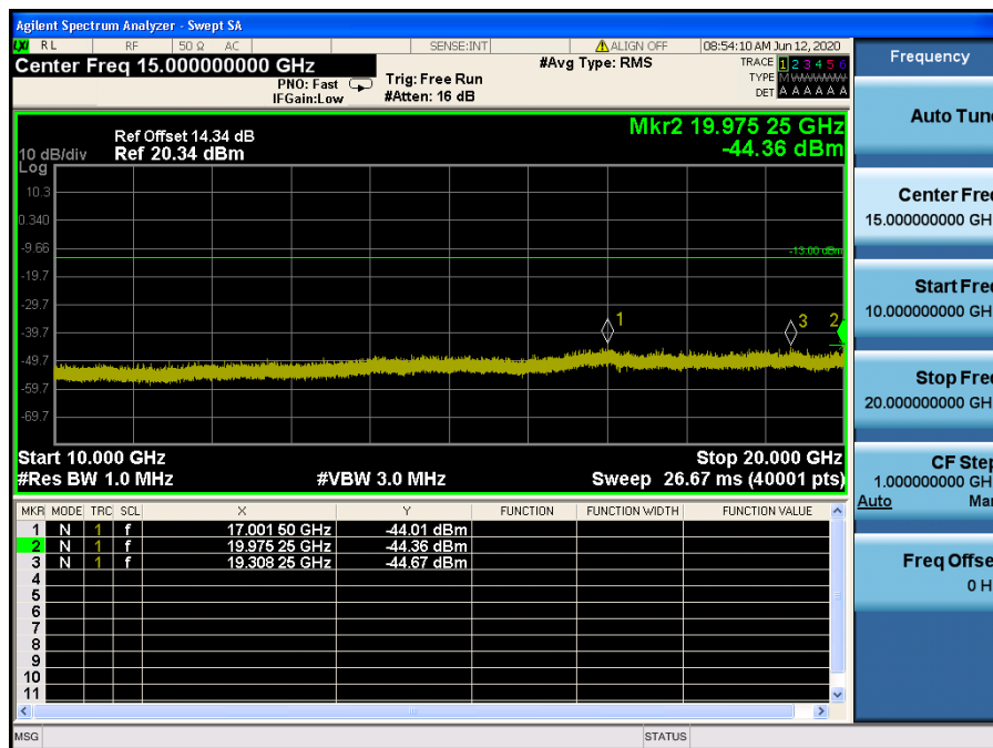
LTE Band 2 / 1.4 MHz / 64QAM - RB Size/Offset (1/5) – High Channel
