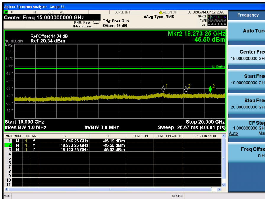
LTE Band 2 / 1.4 MHz / 64QAM - RB Size/Offset (6/0) – Low Channel
