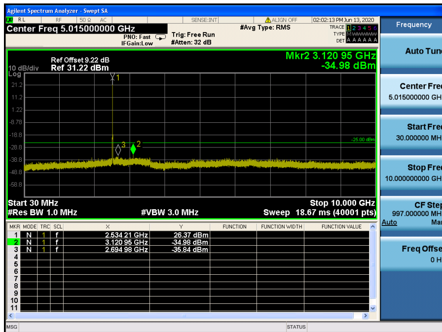
LTE Band 7 / 5 MHz / 16QAM - RB Size/Offset (12/0) – Mid Channel
