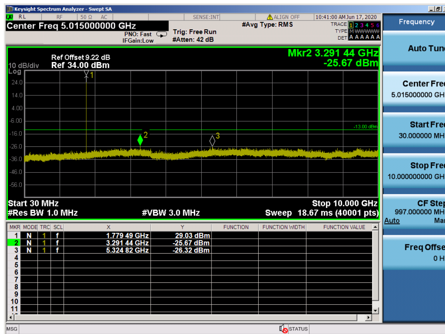
LTE Band 66, 4 / 1.4 MHz / 64QAM - RB Size/Offset (3/3) – High Channel
