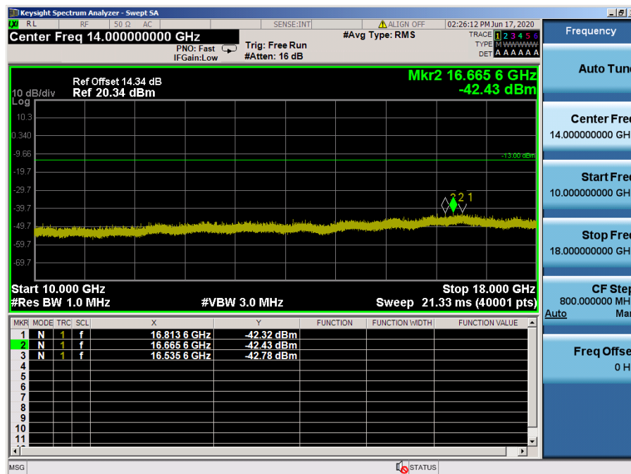
LTE Band 66, 4 / 20 MHz / 64QAM - RB Size/Offset (50/25) – Mid Channel
