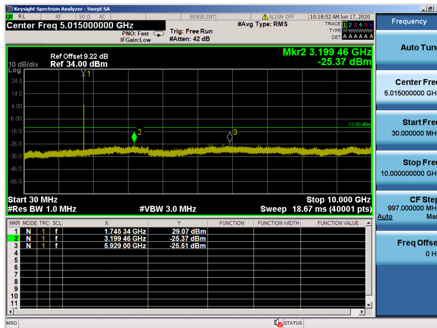
LTE Band 66, 4 / 1.4 MHz / 64QAM - RB Size/Offset (1/2) – Mid Channel
