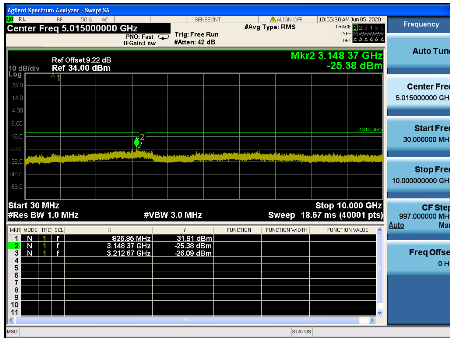
LTE Band 5 / 3MHz / QPSK - RB Size/Offset (1/14) – Low Channel
