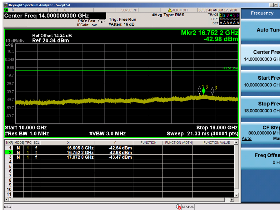
LTE Band 66, 4 / 5 MHz / 16QAM - RB Size/Offset (12/0) – Low Channel
