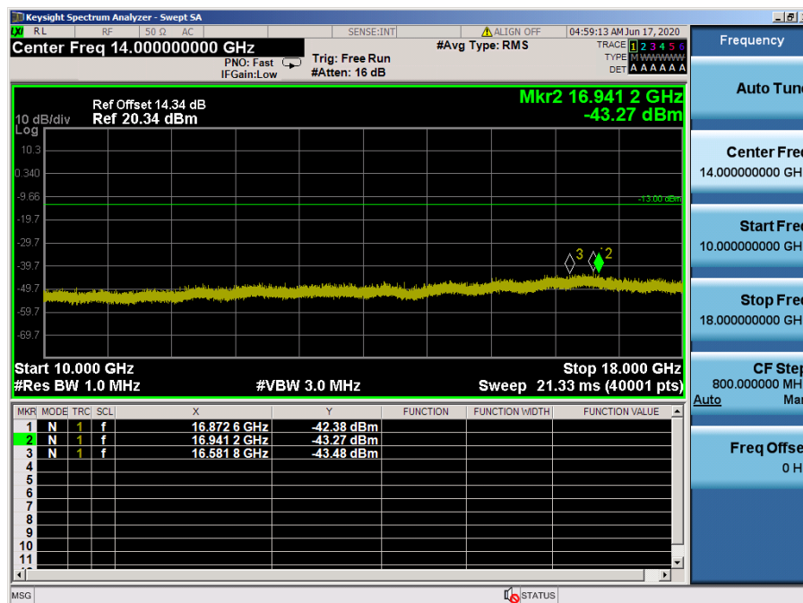
LTE Band 66, 4 / 20 MHz / QPSK - RB Size/Offset (50/50) – High Channel
