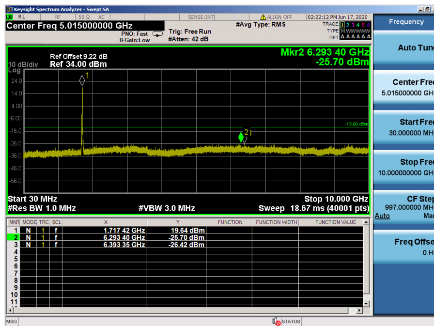
LTE Band 66, 4 / 20 MHz / 64QAM - RB Size/Offset (100/0) – Low Channel
