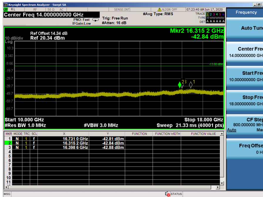
LTE Band 66, 4 / 5 MHz / 16QAM - RB Size/Offset (12/6) – High Channel
