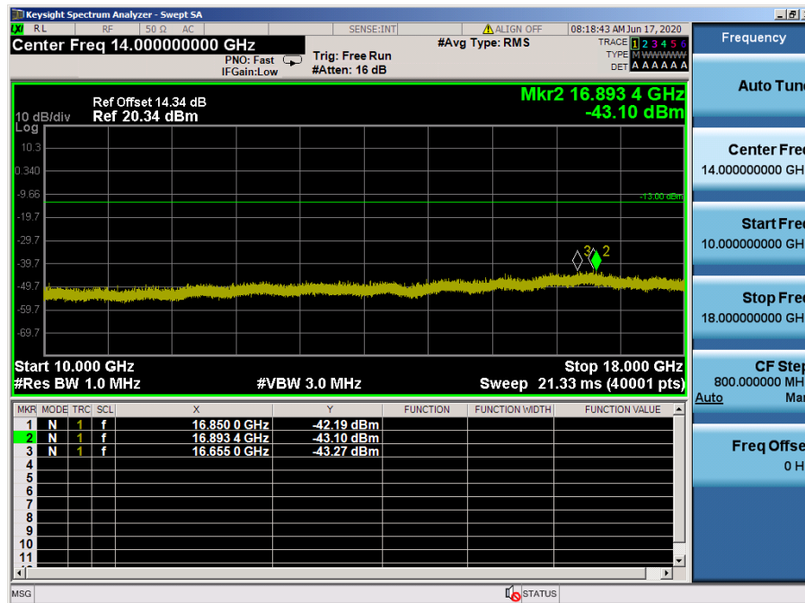
LTE Band 66, 4 / 10 MHz / 16QAM - RB Size/Offset (50/0) – High Channel
