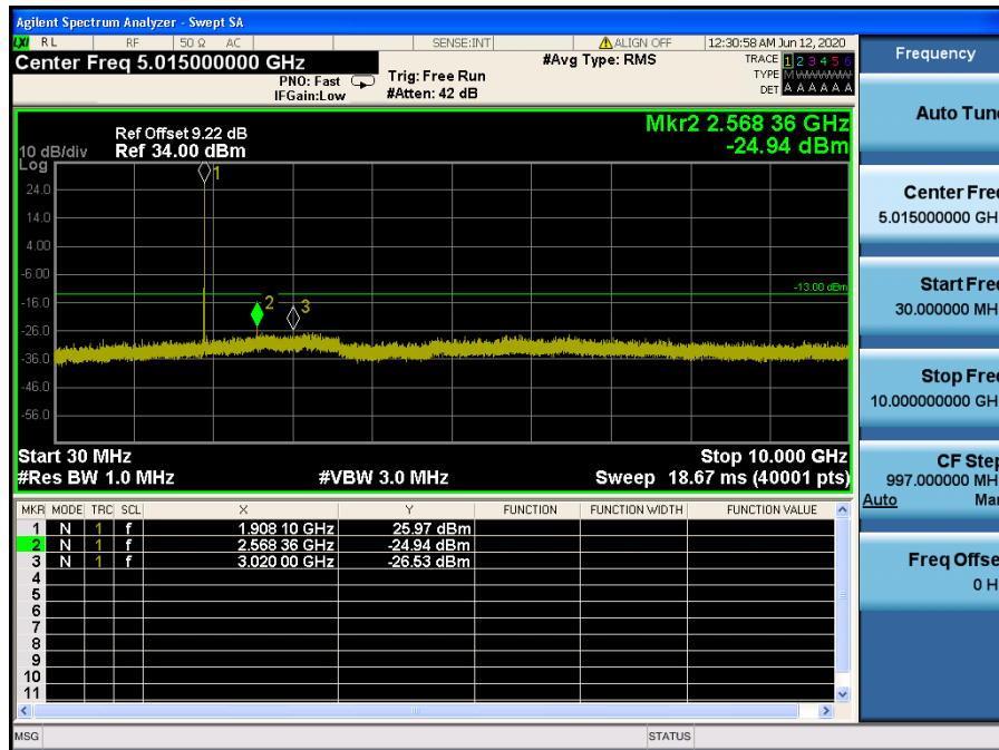
LTE Band 2 / 5 MHz / QPSK - RB Size/Offset (12/13) – High Channel
