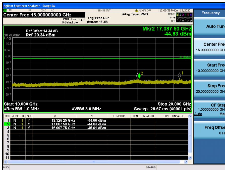
LTE Band 2 / 15 MHz / 64QAM - RB Size/Offset (36/0) – Mid Channel
