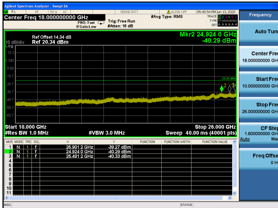
LTE Band 7 / 15 MHz / 64QAM - RB Size/Offset (1/0) – Low Channel
