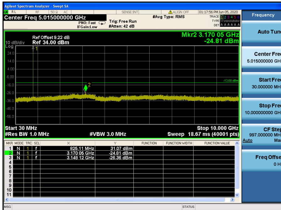
LTE Band 5 / 1.4 MHz / 16QAM - RB Size/Offset (3/2) – Low Channel
