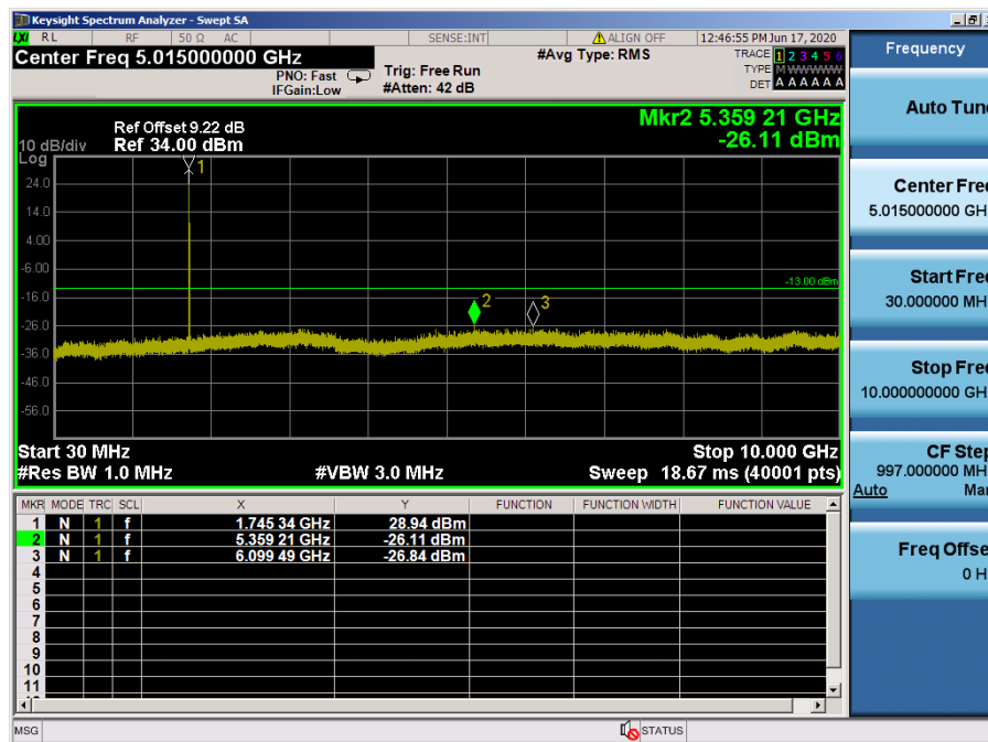
LTE Band 66, 4 / 10 MHz / 64QAM - RB Size/Offset (1/25) – Mid Channel
