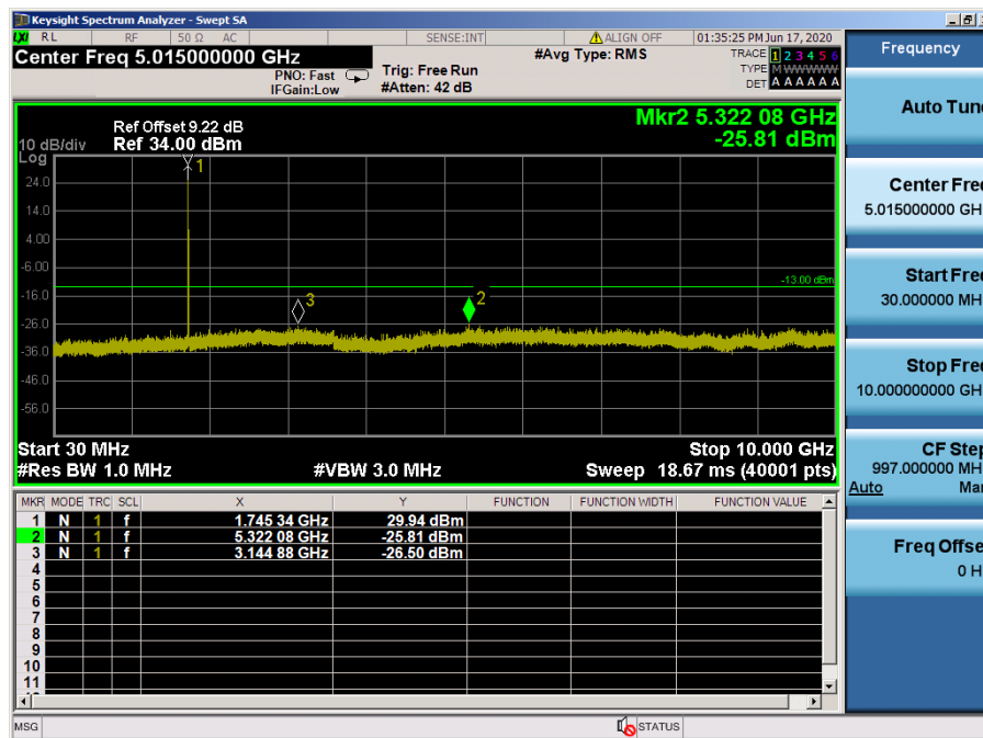
LTE Band 66, 4 / 15 MHz / 64QAM - RB Size/Offset (1/36) – Mid Channel
