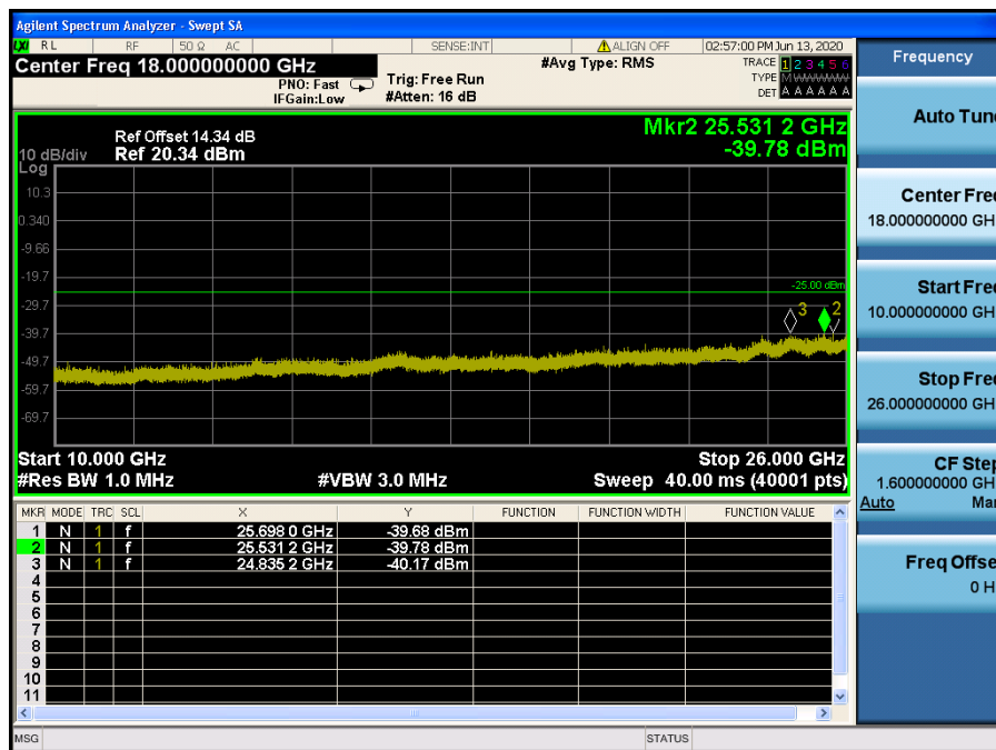
LTE Band 7 / 10 MHz / 16QAM - RB Size/Offset (25/25) – High Channel
