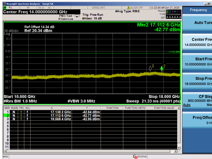
LTE Band 66, 4 / 3MHz / 64QAM - RB Size/Offset (1/14) – High Channel
