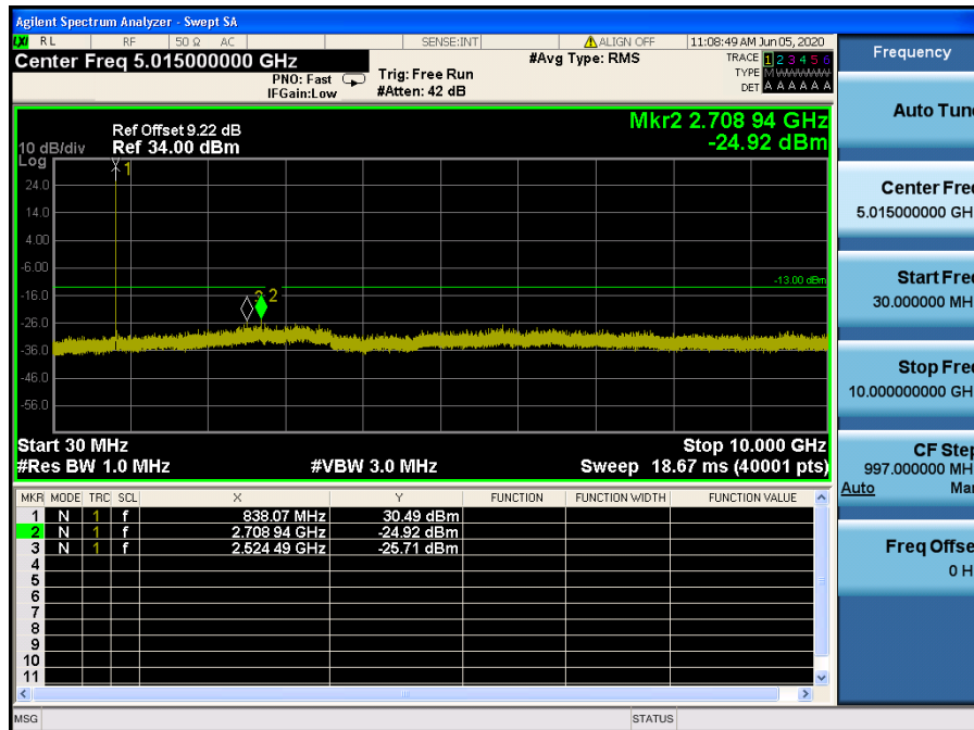
LTE Band 5 / 3MHz / QPSK - RB Size/Offset (1/0) – Mid Channel
