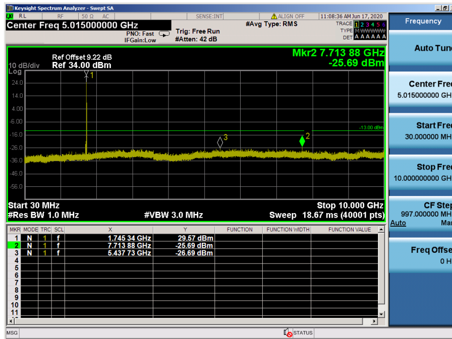
LTE Band 66, 4 / 3MHz / 64QAM - RB Size/Offset (1/7) – Mid Channel
