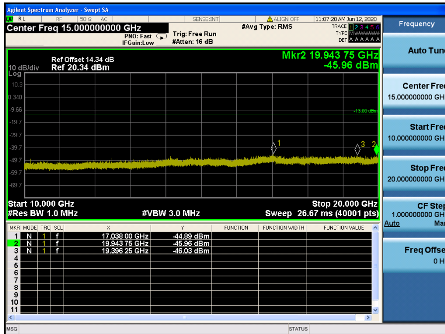
LTE Band 2 / 10 MHz / 64QAM - RB Size/Offset (25/12) – Low Channel
