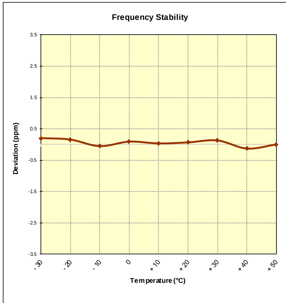
Figure 7-14. Frequency Stability Graph (PCS CDMA Mode – Ch. 600)
