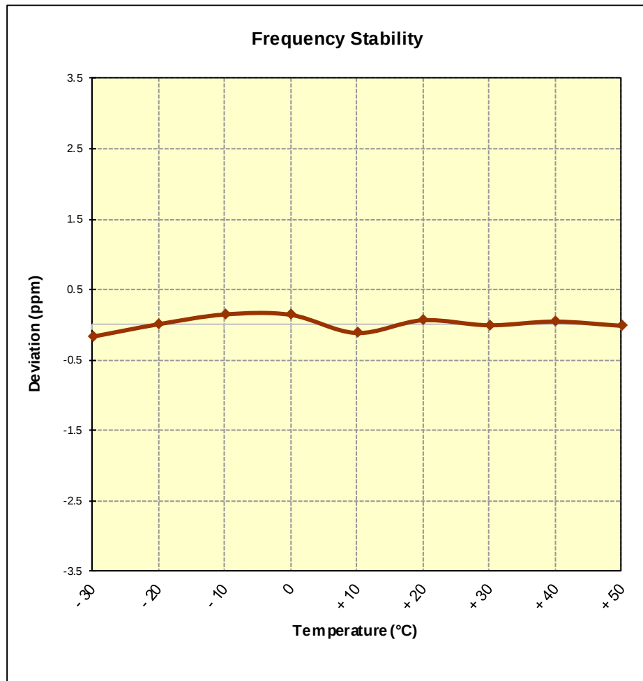
Figure 7-13. Frequency Stability Graph (PCS GPRS Mode – Ch. 661)
