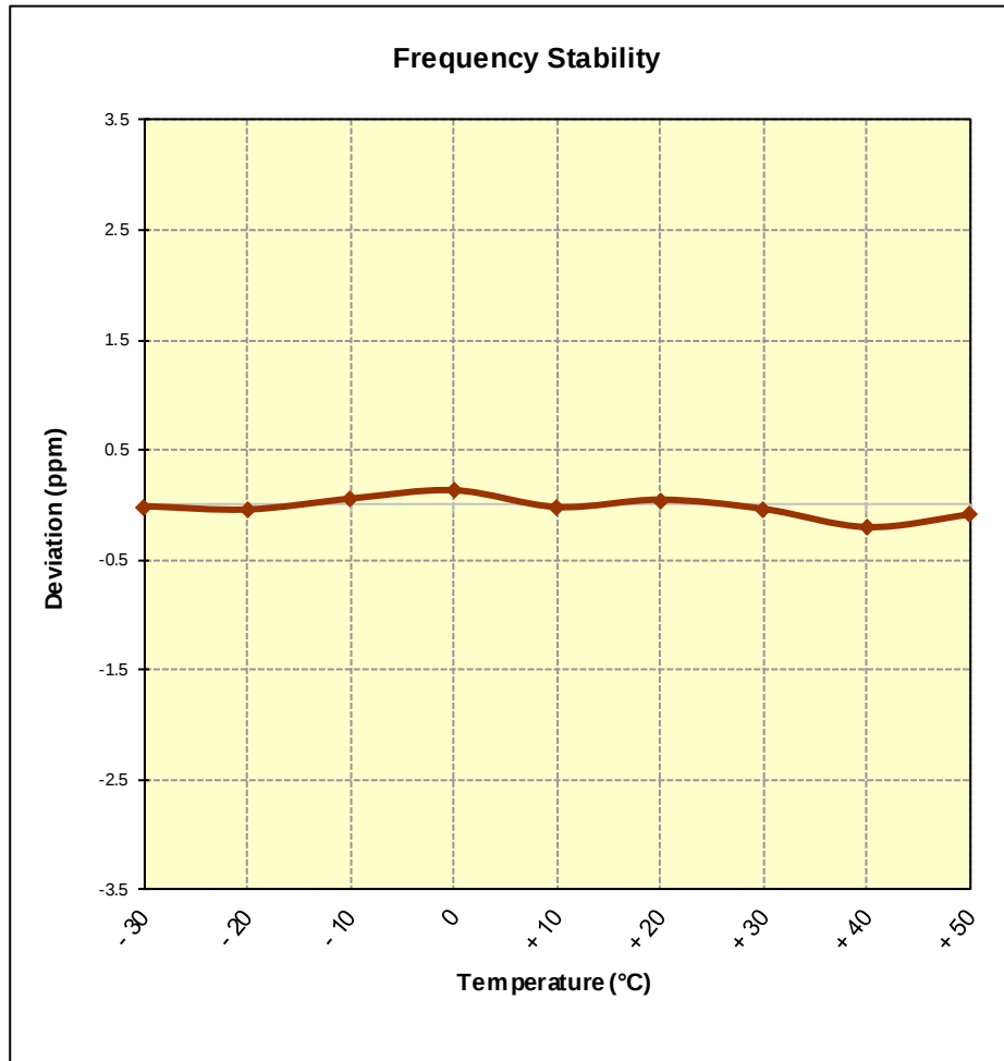
Figure 7-15. Frequency Stability Graph (PCS WCDMA Mode – Ch. 9400)
