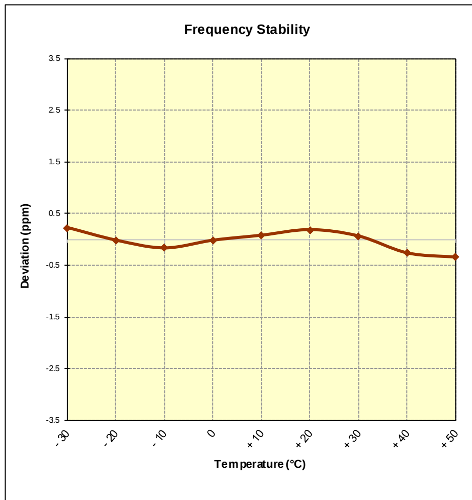
Figure 7-11. Frequency Stability Graph (Cellular WCDMA Mode – Ch. 4183)
