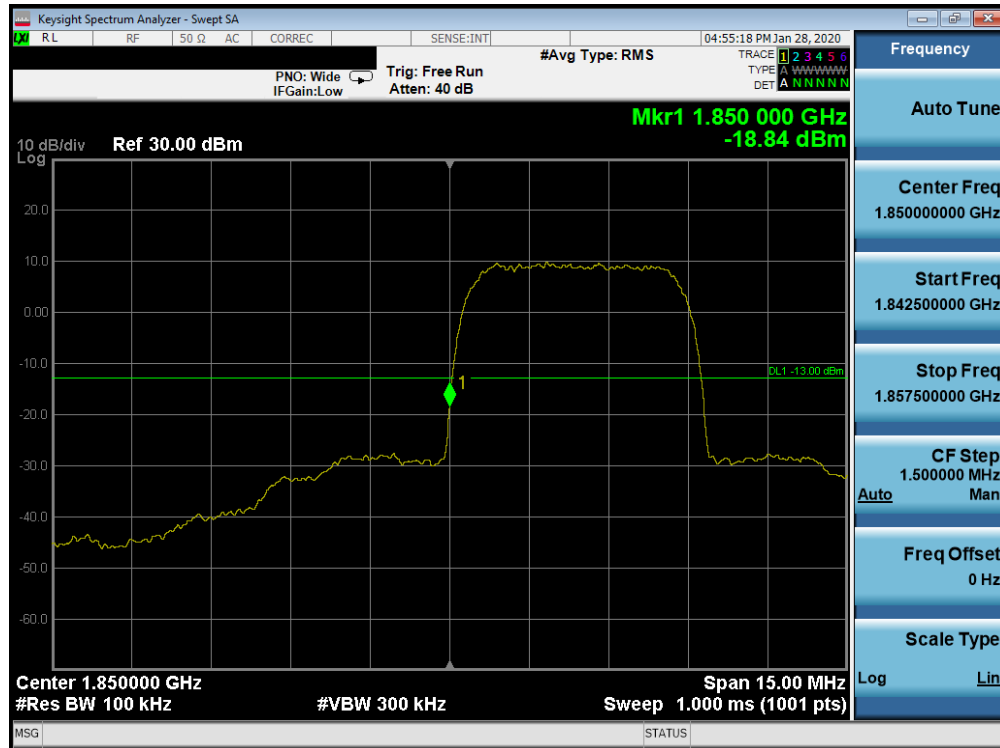
Plot 7-90. Band Edge Plot (PCS WCDMA Mode - Low Channel)
