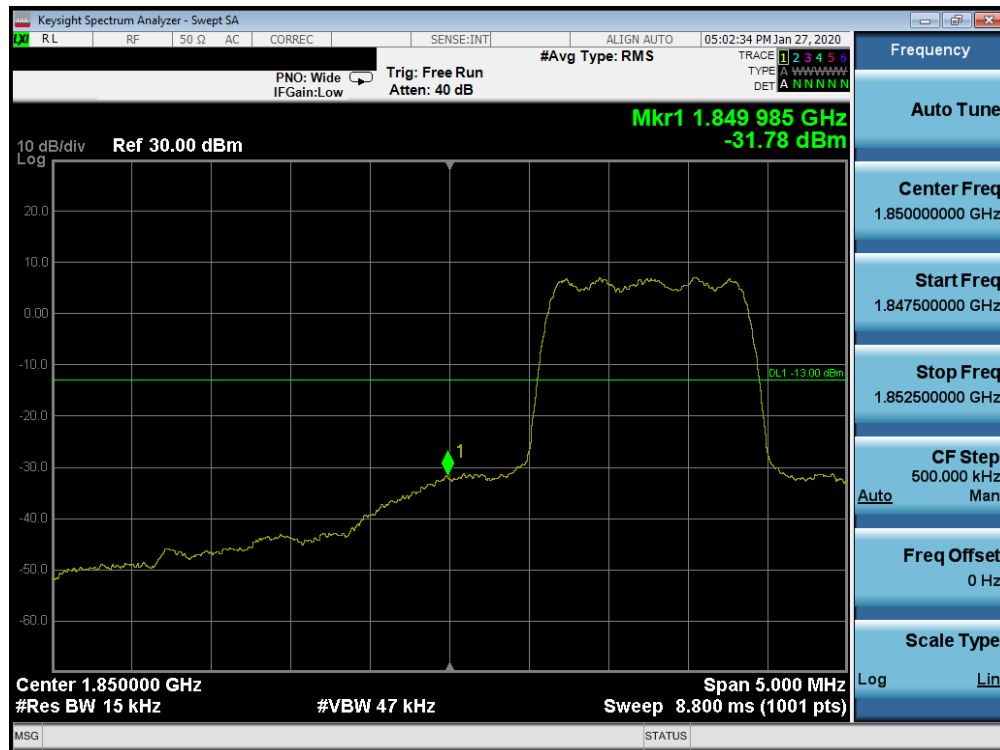
Plot 7-80. Band Edge Plot (PCS CDMA Mode - Low Channel)
