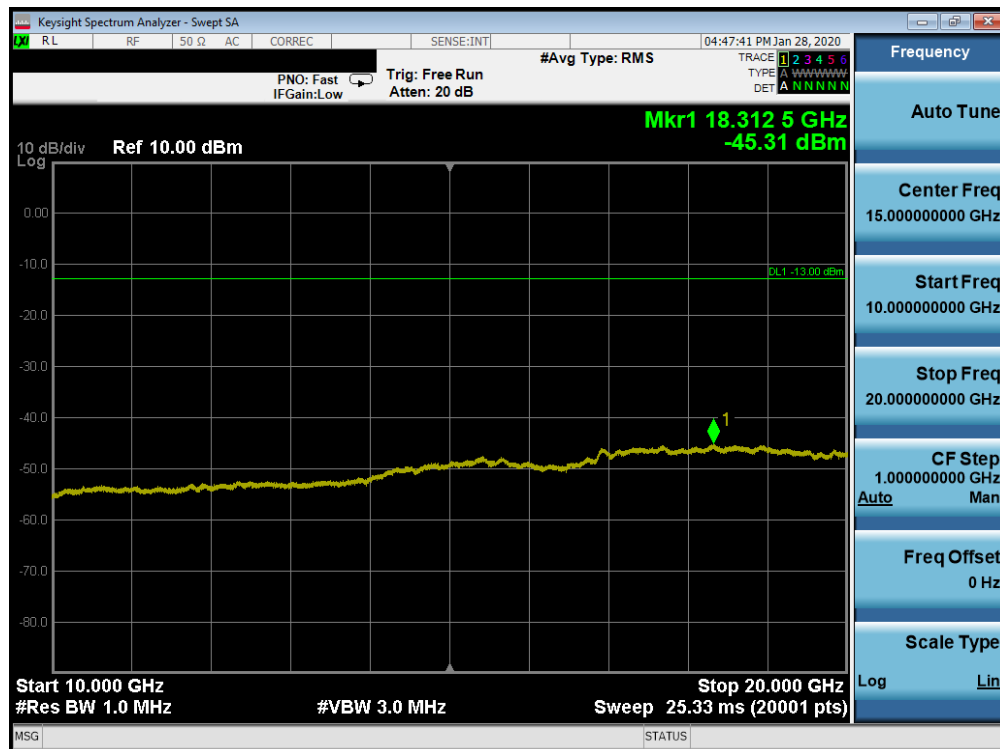
Plot 7-57. Conducted Spurious Plot (AWS WCDMA Mode - Mid Channel)
