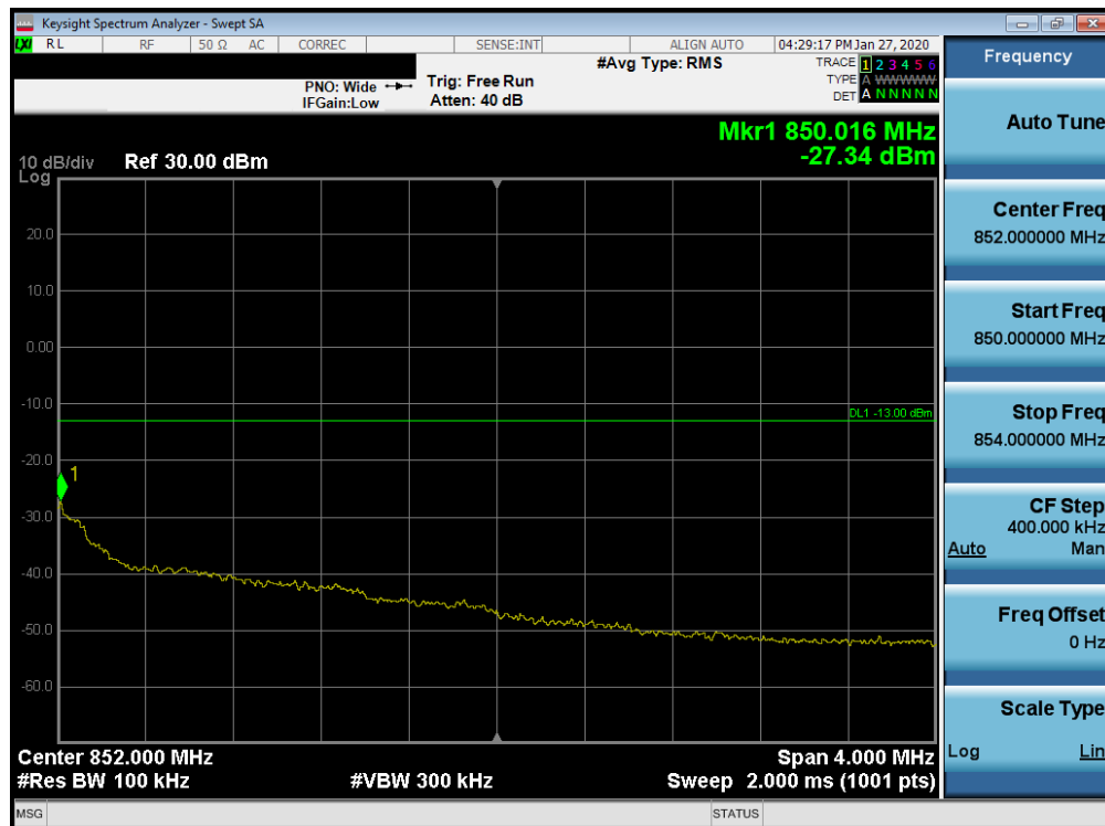
Plot 7-79. 4MHz Span Plot (Cellular CDMA Mode - High Channel)
