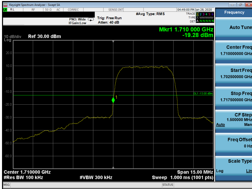
Plot 7-86. Band Edge Plot (AWS WCDMA Mode - Low Channel)
