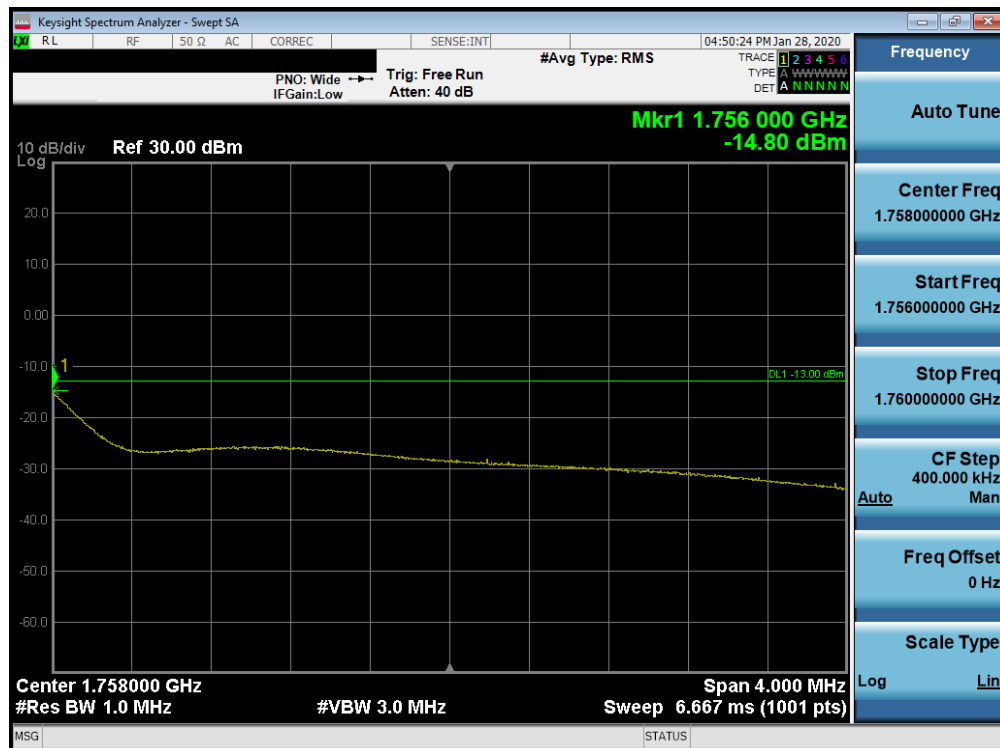
Plot 7-89. 4MHz Span Plot (AWS WCDMA Mode - High Channel)
