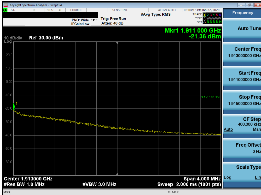
Plot 7-83. 4MHz Span Plot (PCS CDMA Mode - High Channel)
