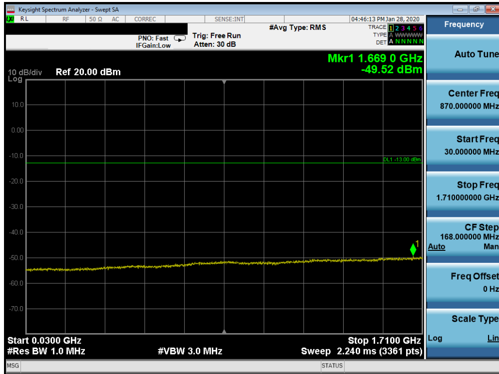
Plot 7-55. Conducted Spurious Plot (AWS WCDMA Mode - Mid Channel)
