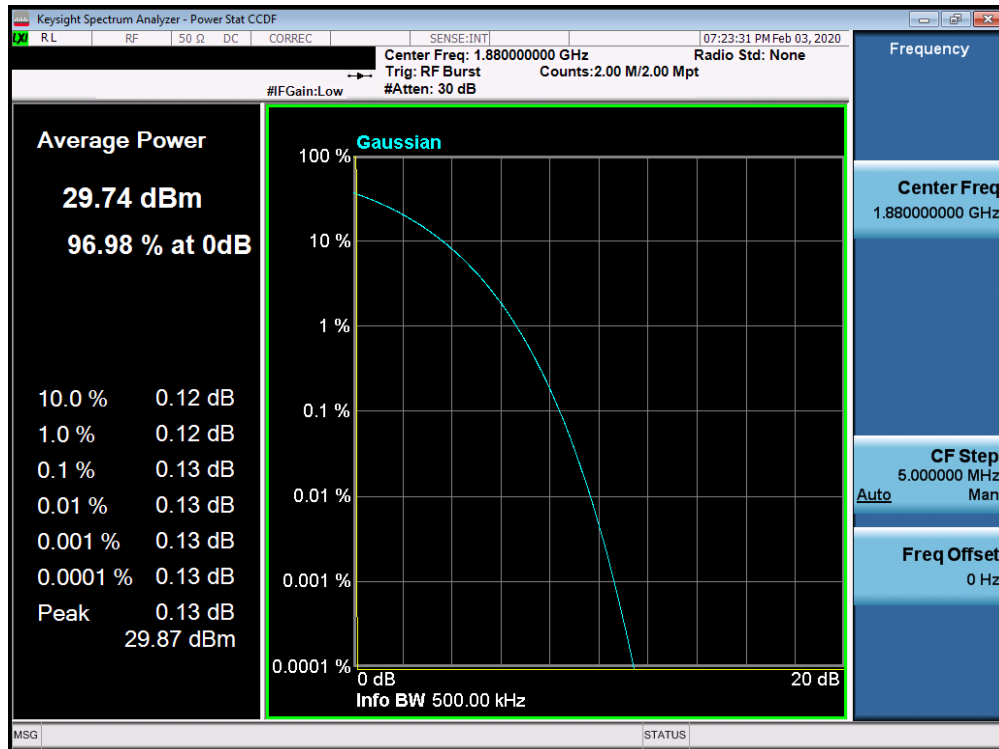
Plot 7-94. Peak-Average Ratio Plot (PCS GPRS Mode)
