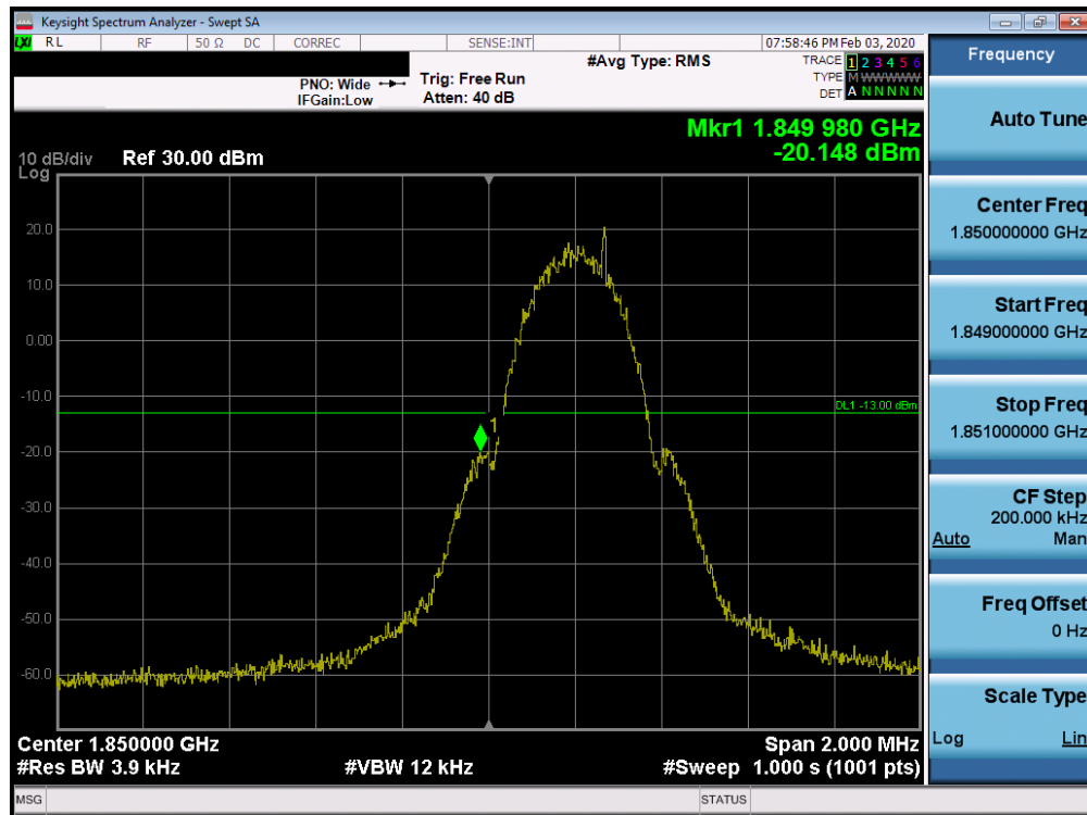
Plot 7-72. Band Edge Plot (PCS GSM Mode - Low Channel)
