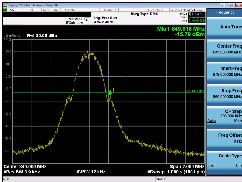
Plot 7-71. Band Edge Plot (Cellular GSM Mode - High Channel)
