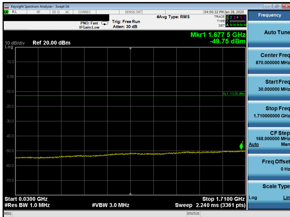
Plot 7-58. Conducted Spurious Plot (AWS WCDMA Mode - High Channel)
