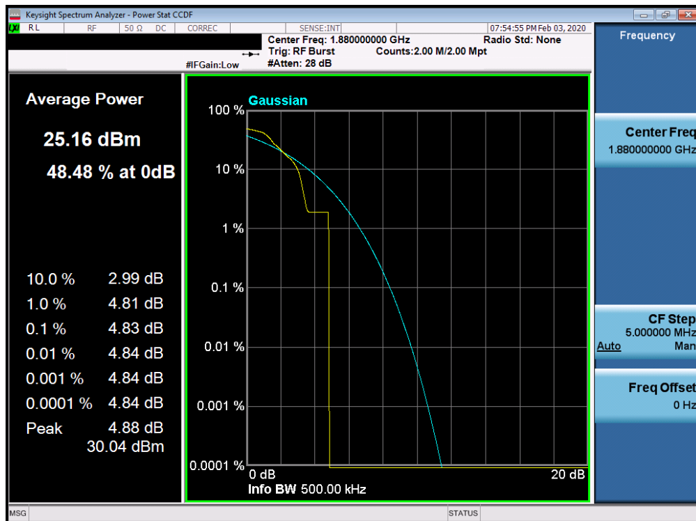
Plot 7-95. Peak-Average Ratio Plot (EDGE1900 Mode)
