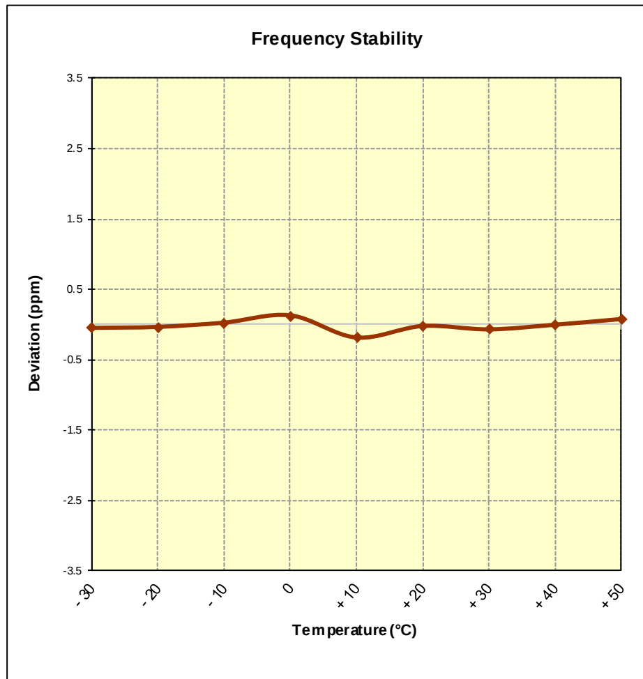
Figure 7-12. Frequency Stability Graph (AWS WCDMA Mode – Ch. 1413)
