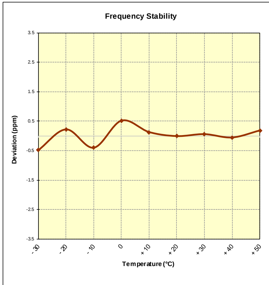
Figure 7-10. Frequency Stability Graph (Cellular CDMA Mode – Ch. 384)
