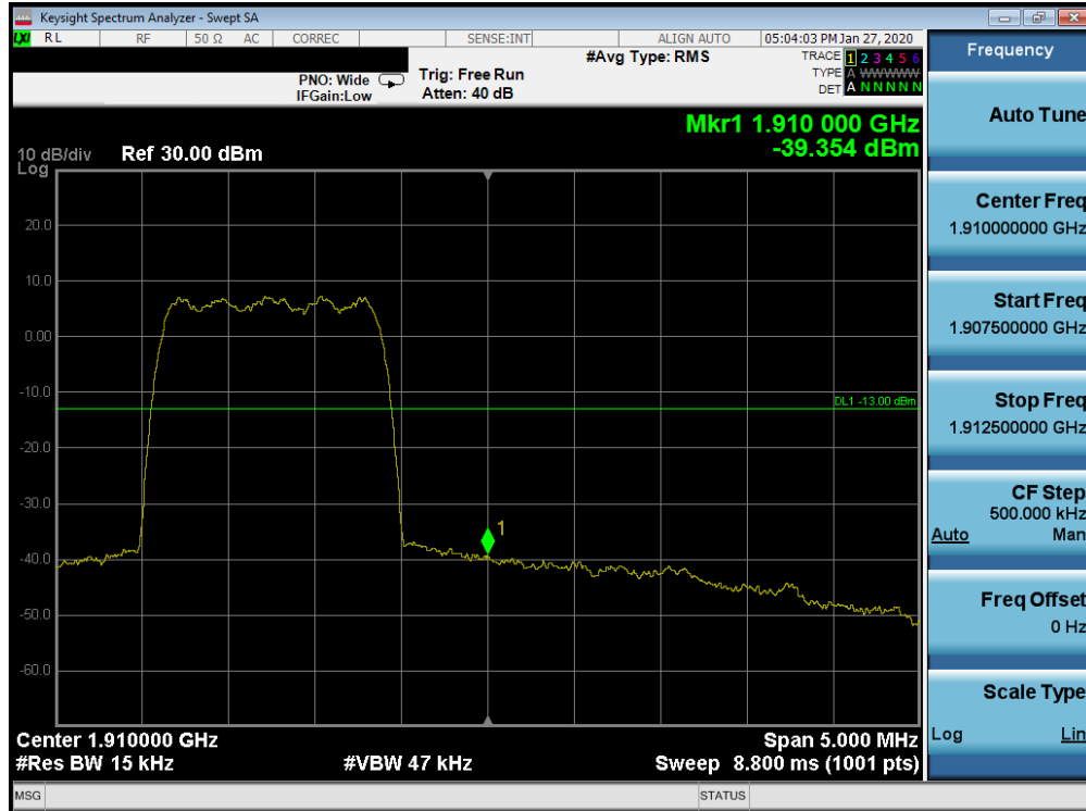
Plot 7-82. Band Edge Plot (PCS CDMA Mode - High Channel)
