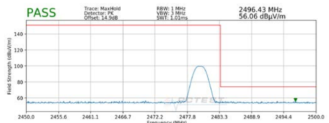
Plot 7-2. Radiated Restricted Upper Band Edge Measurement (Peak)
