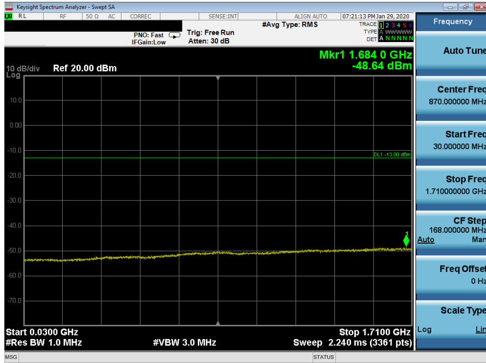
Plot 7-124. Conducted Spurious Plot (Band 66/4 - 15.0MHz QPSK - RB Size 1, RB Offset 0 - Mid Channel)
