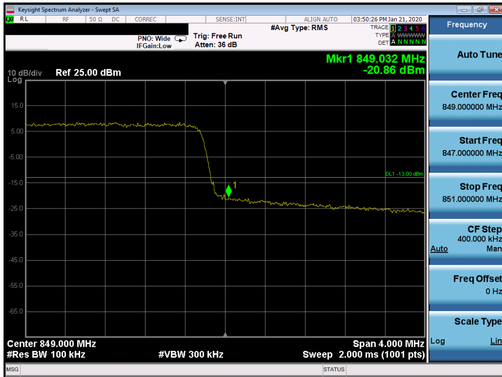
Plot 7-180. Upper Band Edge Plot (Band 26/5 - 5.0MHz QPSK - Full RB Configuration)
