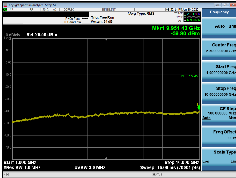
Plot 7-26. Conducted Spurious Plot (LTE Band 26 – 10MHz QPSK Size 1, RB Offset 0- Mid Channel)
