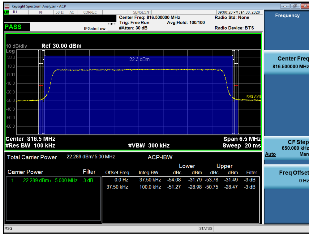
Plot 7-33. Channel Edge Plot (LTE Band 26 – 5MHz QPSK – Low Channel)
