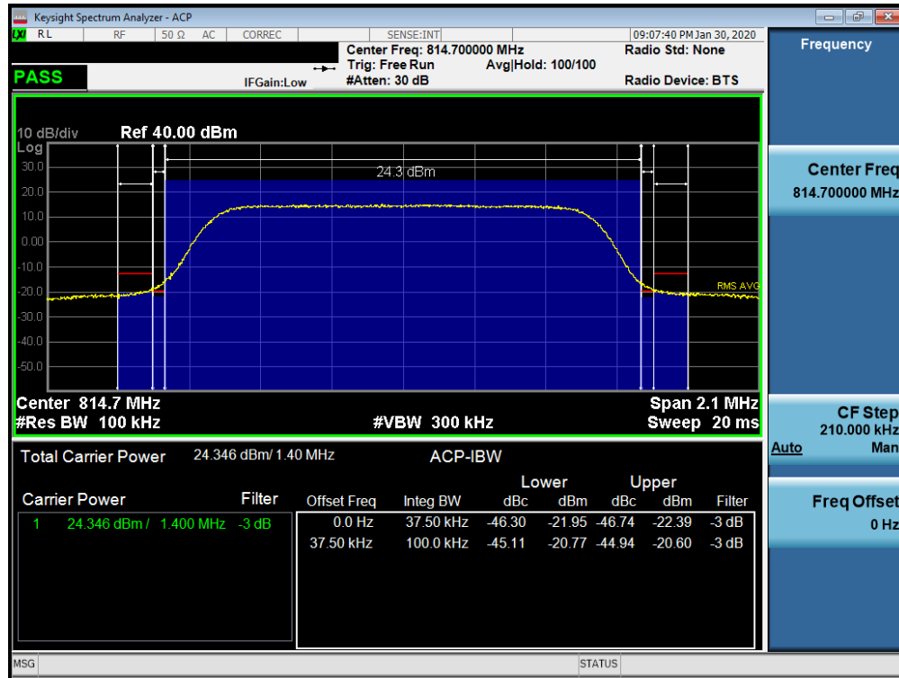
Plot 7-29. Channel Edge Plot (LTE Band 26 – 1.4MHz QPSK – Low Channel)
