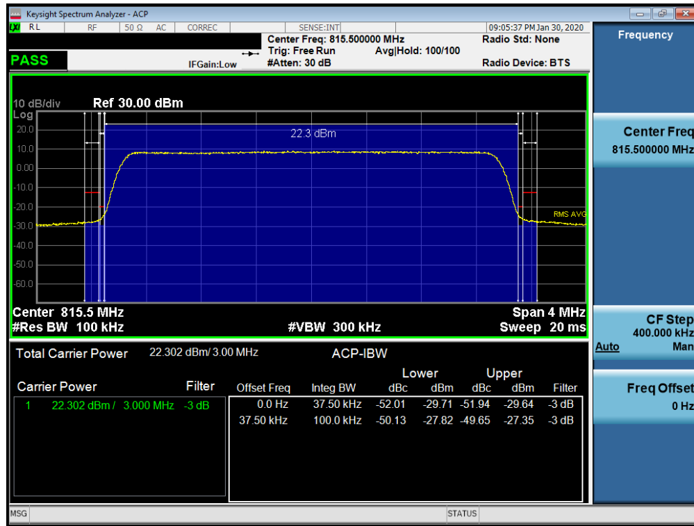
Plot 7-31. Channel Edge Plot (LTE Band 26 – 3.0MHz QPSK – Low Channel)
