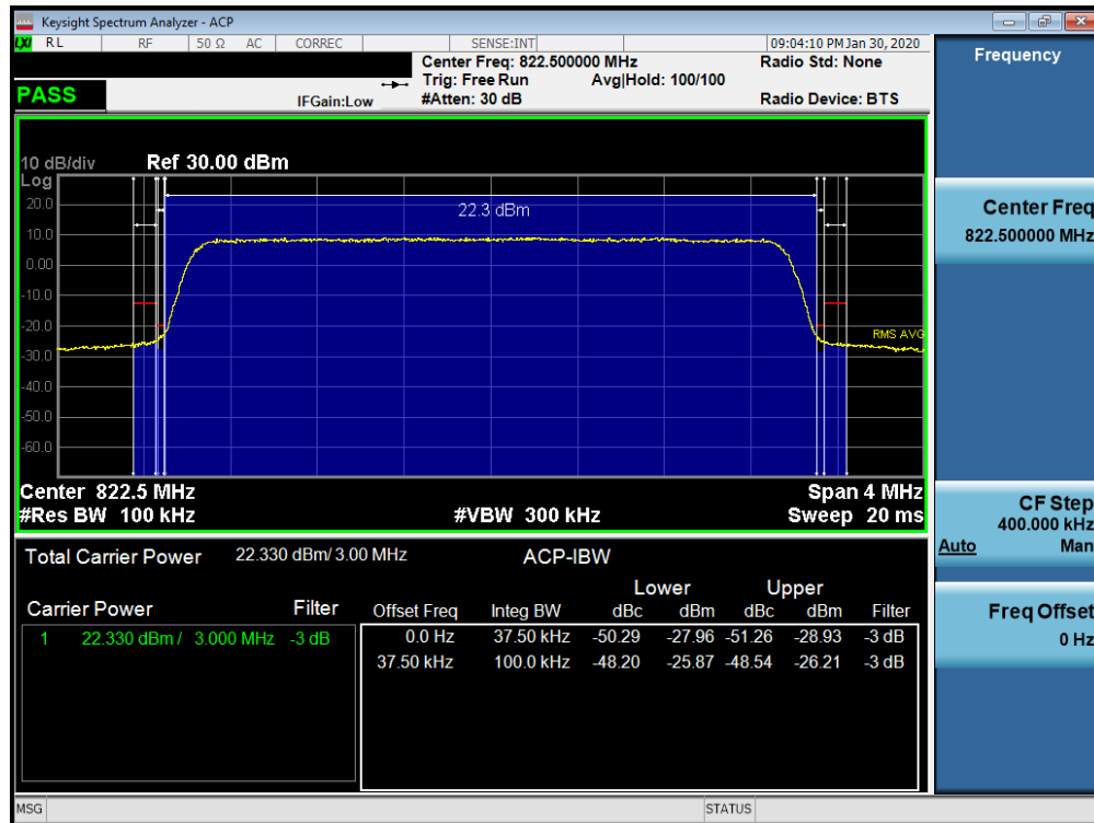
Plot 7-32. Channel Edge Plot (LTE Band 26 – 3.0MHz QPSK – High Channel)
