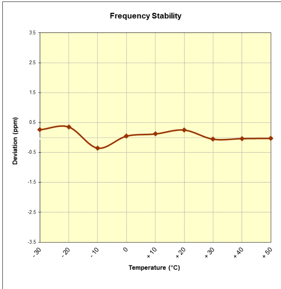
Figure 7-7. CDMA BC10 Frequency Stability Chart
