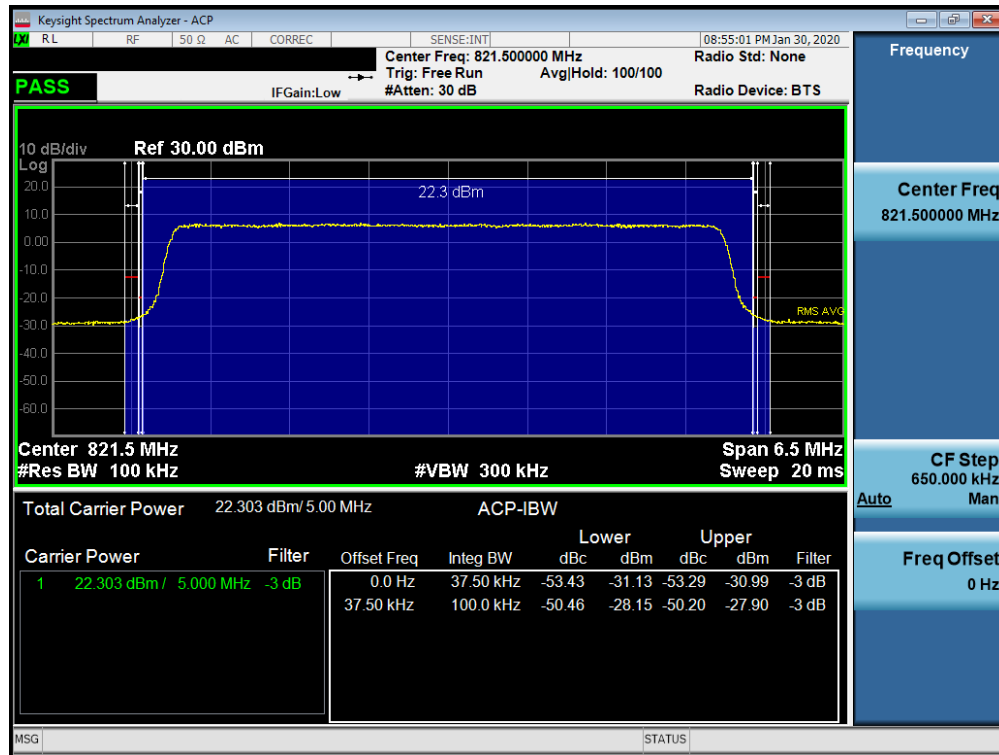
Plot 7-34. Channel Edge Plot (LTE Band 26 – 5MHz QPSK – High Channel)
