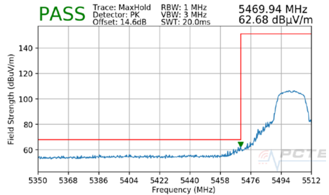
Plot 7-90. Radiated Lower Band Edge Plot (Peak – UNII Band 2C)
