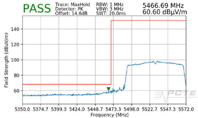
Plot 7-104. Radiated Lower Band Edge Plot (Peak - UNII Band 2C)
