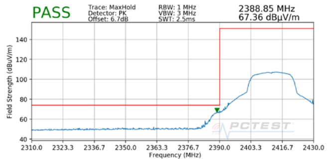
Plot 7-42. Radiated Restricted Lower Band Edge Measurement (Peak)
