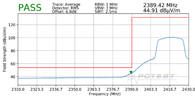
Plot 7-43. Radiated Restricted Lower Band Edge Measurement (Average)
