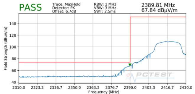
Plot 7-44. Radiated Restricted Lower Band Edge Measurement (Peak)
