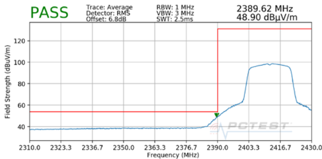
Plot 7-41. Radiated Restricted Lower Band Edge Measurement (Average)
