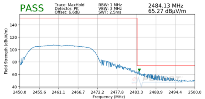
Plot 7-48. Radiated Restricted Upper Band Edge Measurement (Peak)
