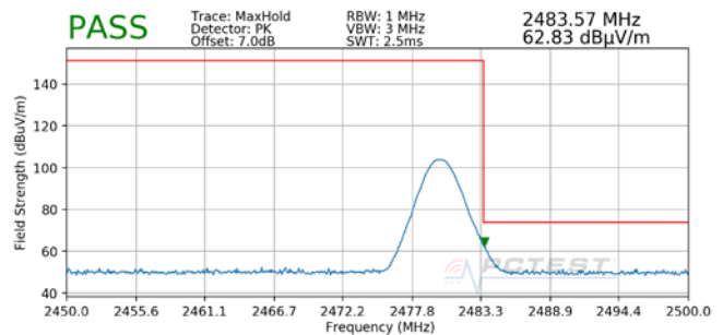
Plot 7-47. Radiated Restricted Upper Band Edge Measurement (Peak)
