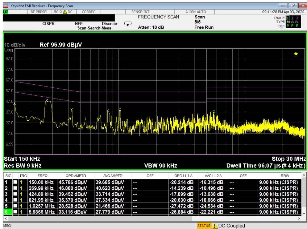
Plot 7-48. Line-Conducted Test Plot (L1)
