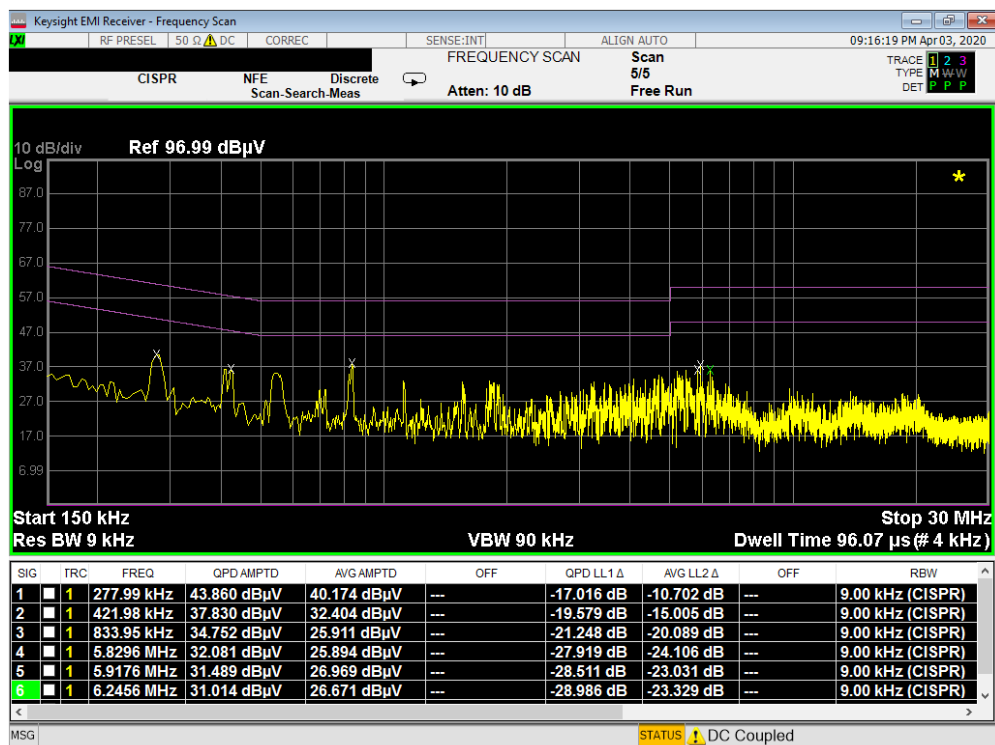
Plot 7-49. Line-Conducted Test Plot (N)
