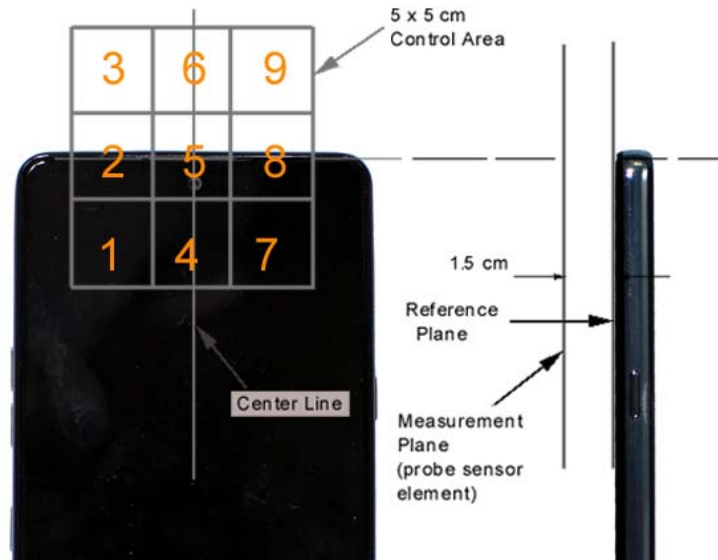
Figure 18-3 5x5 Scan grid above WD (Acoustic Scan Area pictured)
