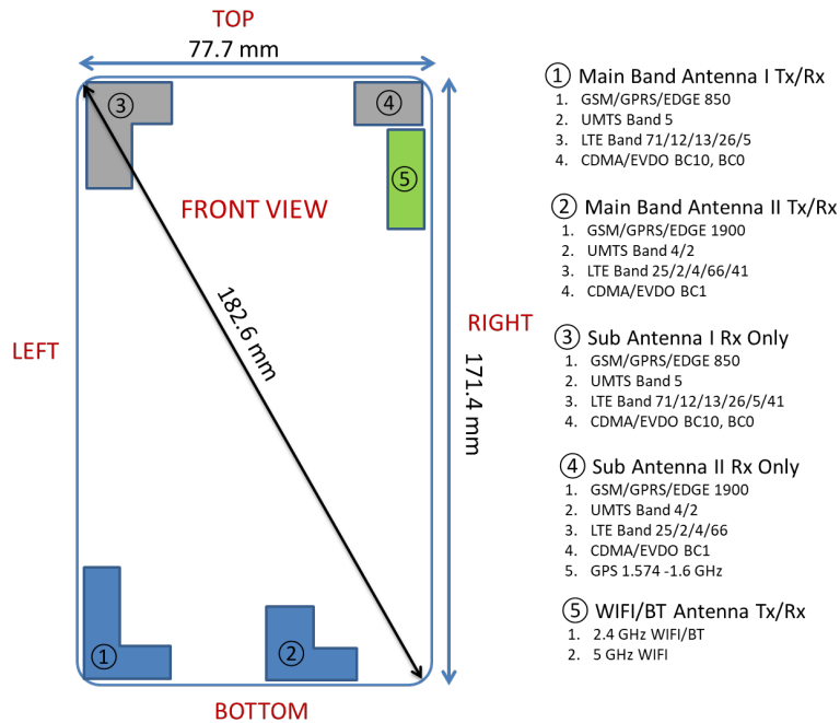
Figure E-1 DUT Antenna Locations
