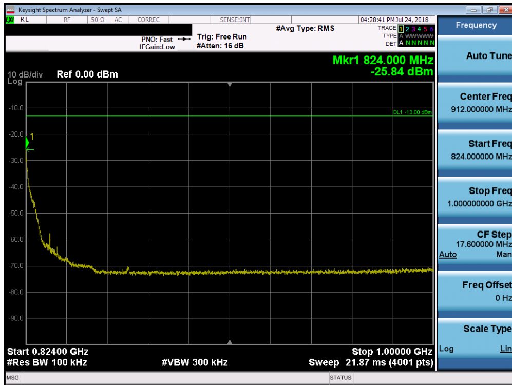
Plot 7-22. Conducted Spurious Plot (Ch. 684)
