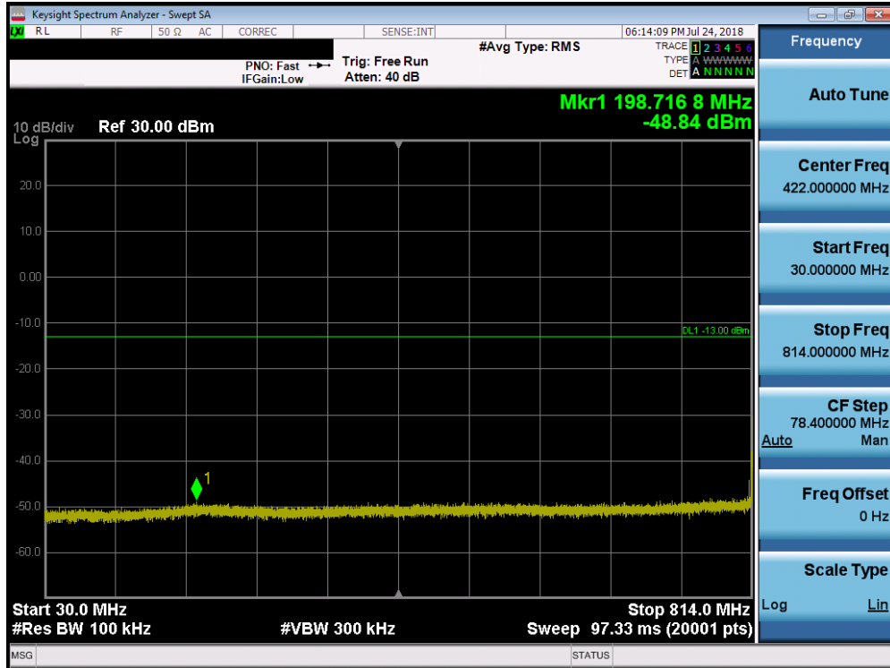
Plot 7-24. Conducted Spurious Plot (LTE Band 26, 10.0MHz QPSK – RB Size 1, RB Offset 0 – Mid Channel)
