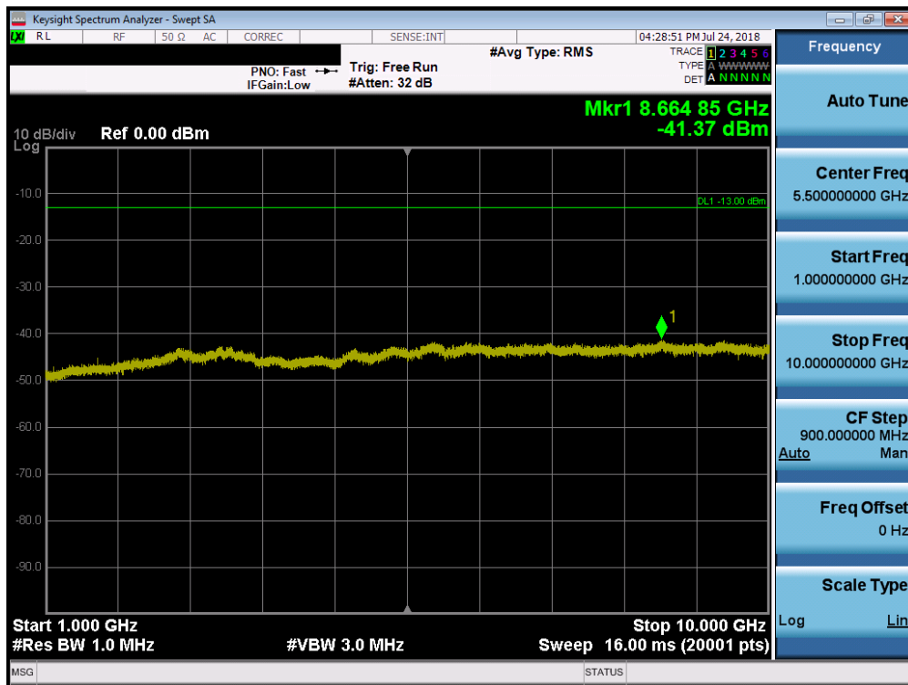
Plot 7-23. Conducted Spurious Plot (Ch. 684)
