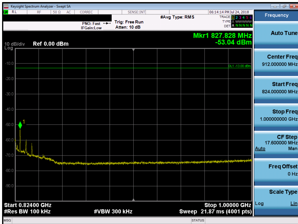
Plot 7-25. Conducted Spurious Plot (LTE Band 26, 10.0MHz QPSK – RB Size 1, RB Offset 0 – Mid Channel)
