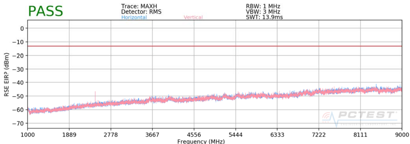
Plot 7-39. Radiated Spurious Plot Above 1GHz (LTE Band 26)
