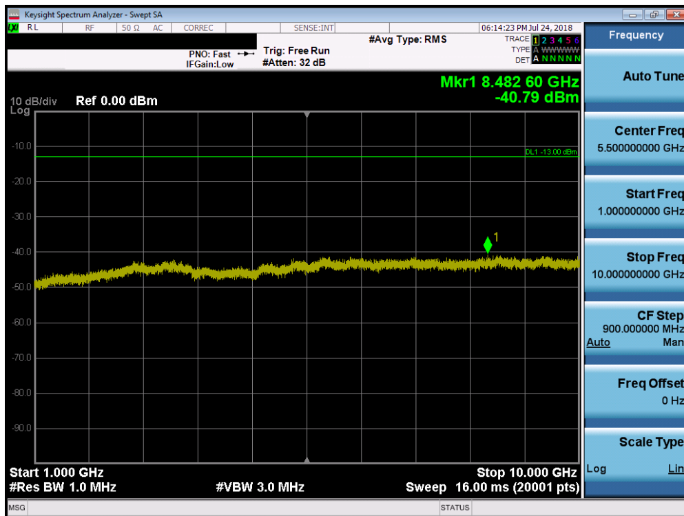
Plot 7-26. Conducted Spurious Plot (LTE Band 26, 10.0MHz QPSK – RB Size 1, RB Offset 0 – Mid Channel)
