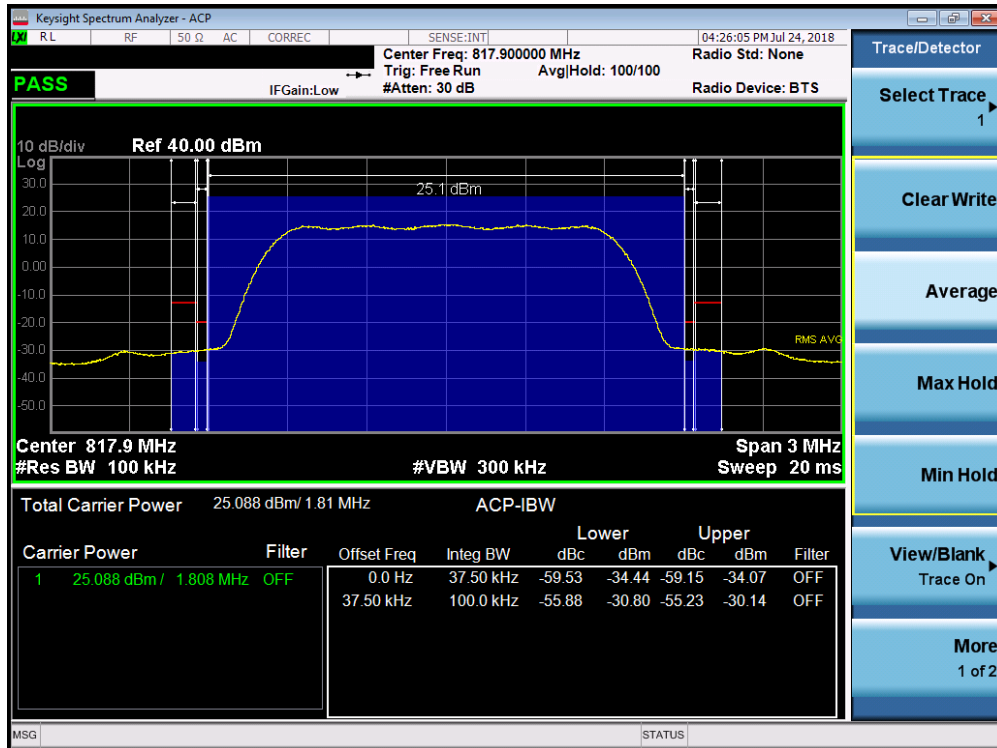
Plot 7-27. Channel Edge Plot (Ch. 476)
