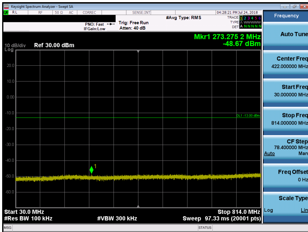
Plot 7-21. Conducted Spurious Plot (Ch. 684)
