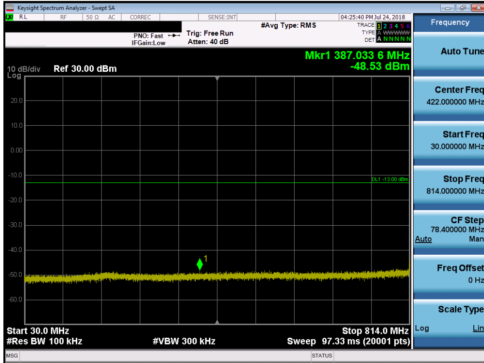
Plot 7-18. Conducted Spurious Plot (Ch. 476)
