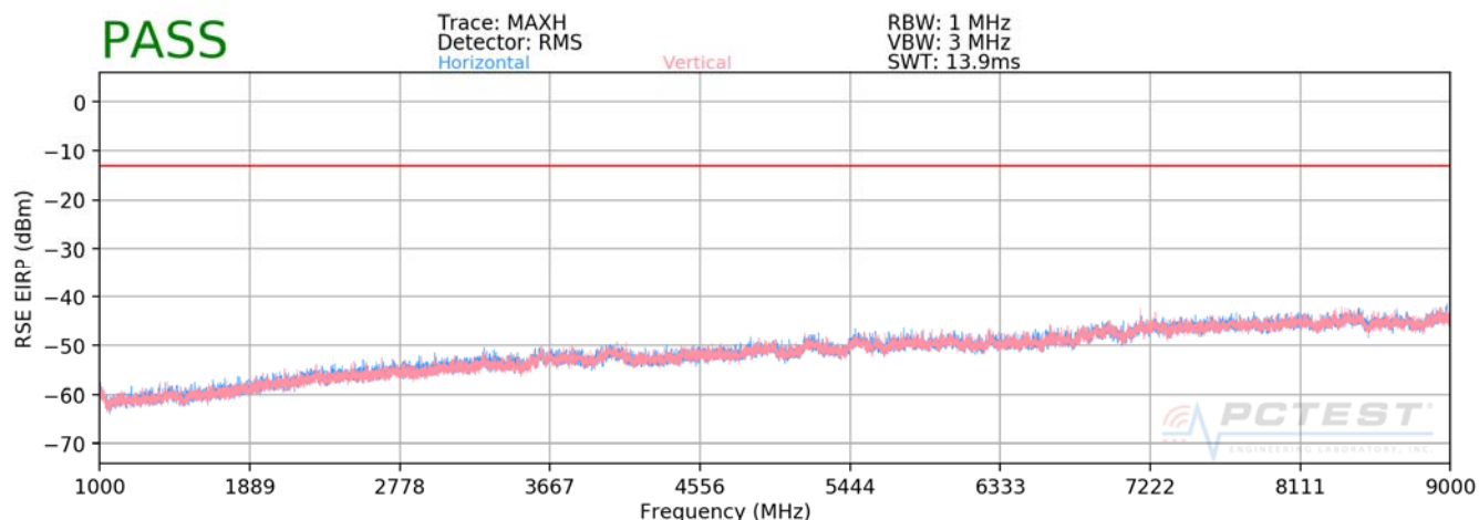
Plot 7-38. Radiated Spurious Plot Above 1GHz (CDMA BC10)
