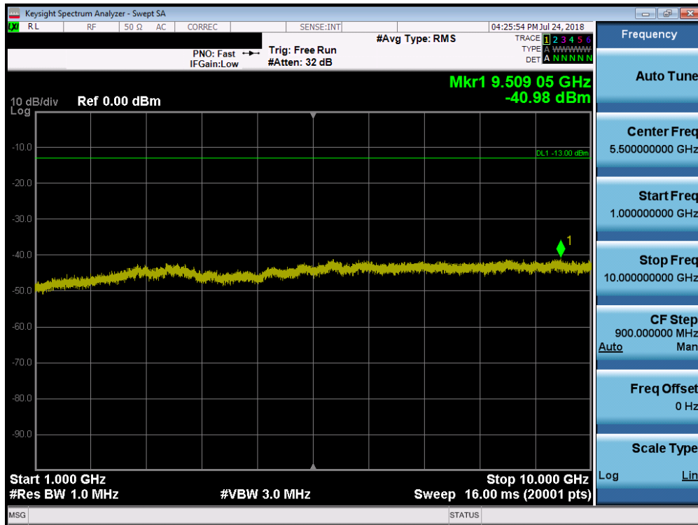
Plot 7-20. Conducted Spurious Plot (Ch. 476)
