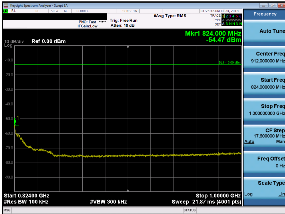
Plot 7-19. Conducted Spurious Plot (Ch. 476)
