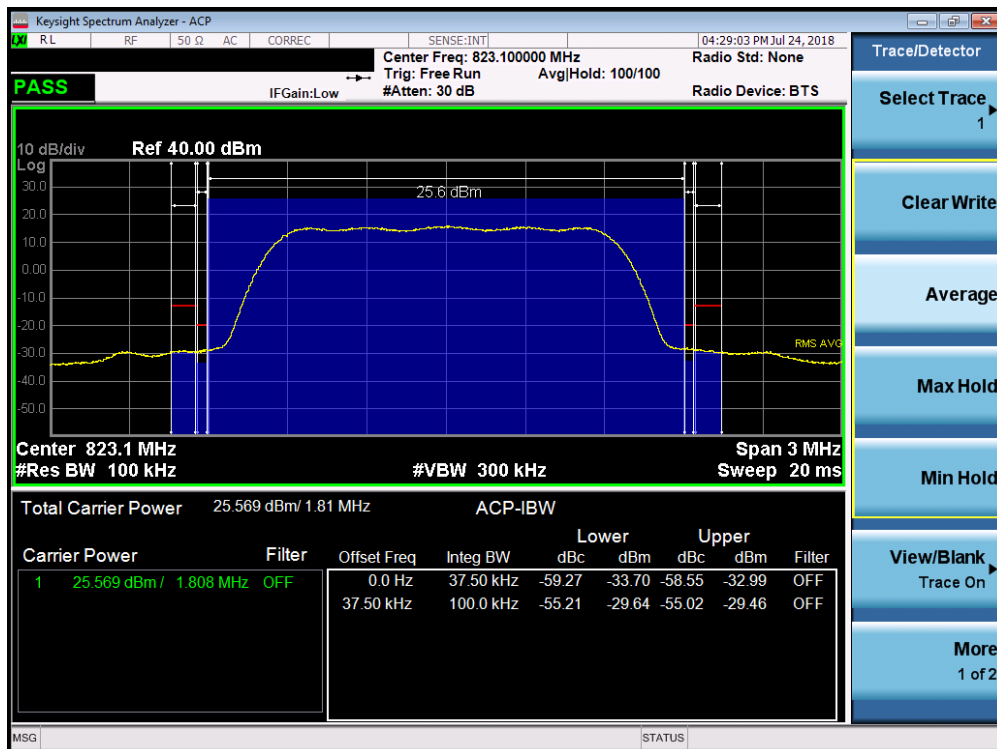
Plot 7-28. Channel Edge Plot (Ch. 684)
