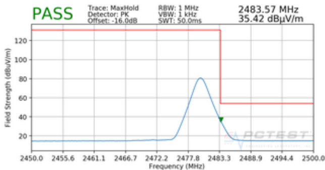
Plot 7-5. Radiated Restricted Upper Band Edge Measurement (Average)
