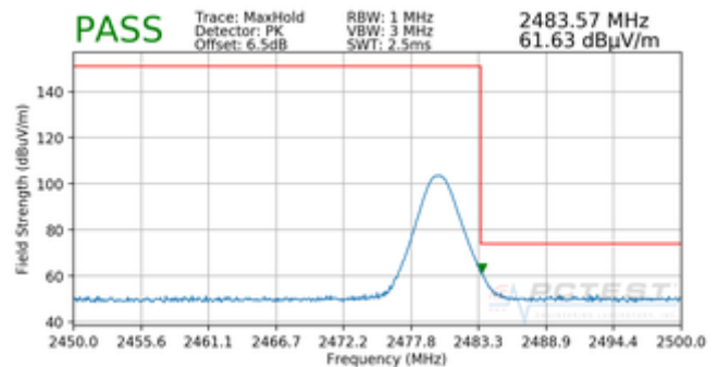
Plot 7-6. Radiated Restricted Upper Band Edge Measurement (Peak)
