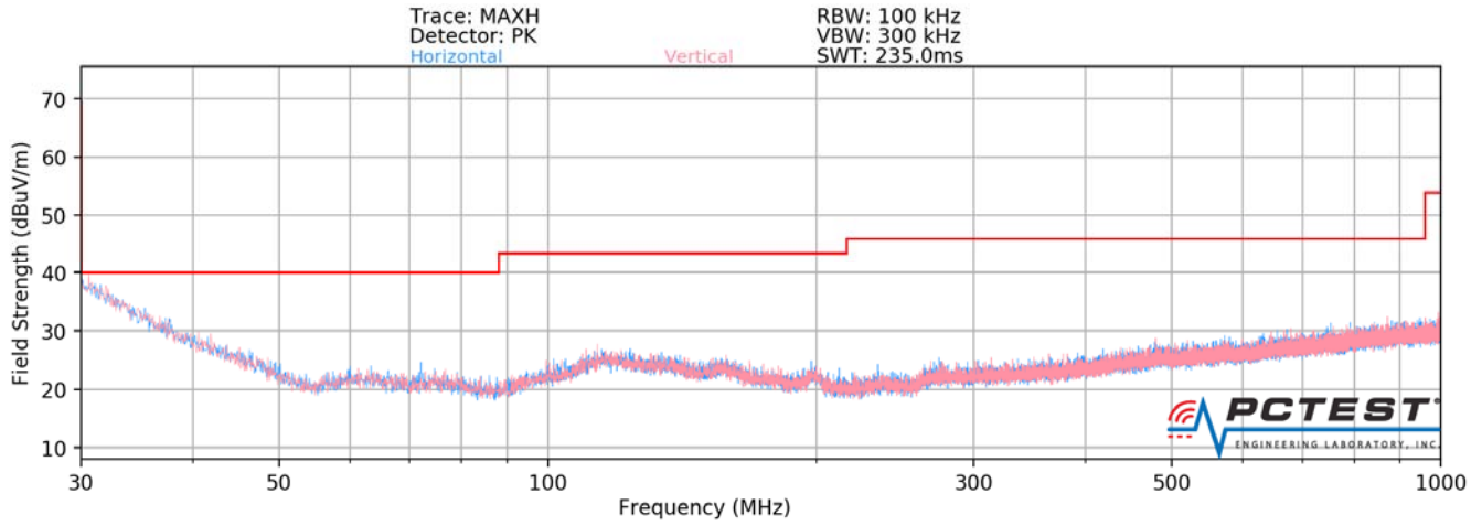
Plot 7-7. Radiated Spurious Plot below 1GHz
