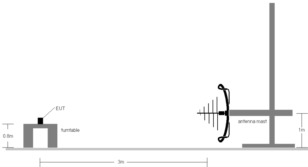
Figure 7-3. Radiated Test Setup > 30MHz
