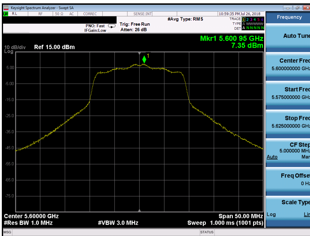
Plot 7-140. Power Spectral Density Plot SISO ANT2 (20MHz BW 802.11n (UNII Band 2C) – Ch. 120)
