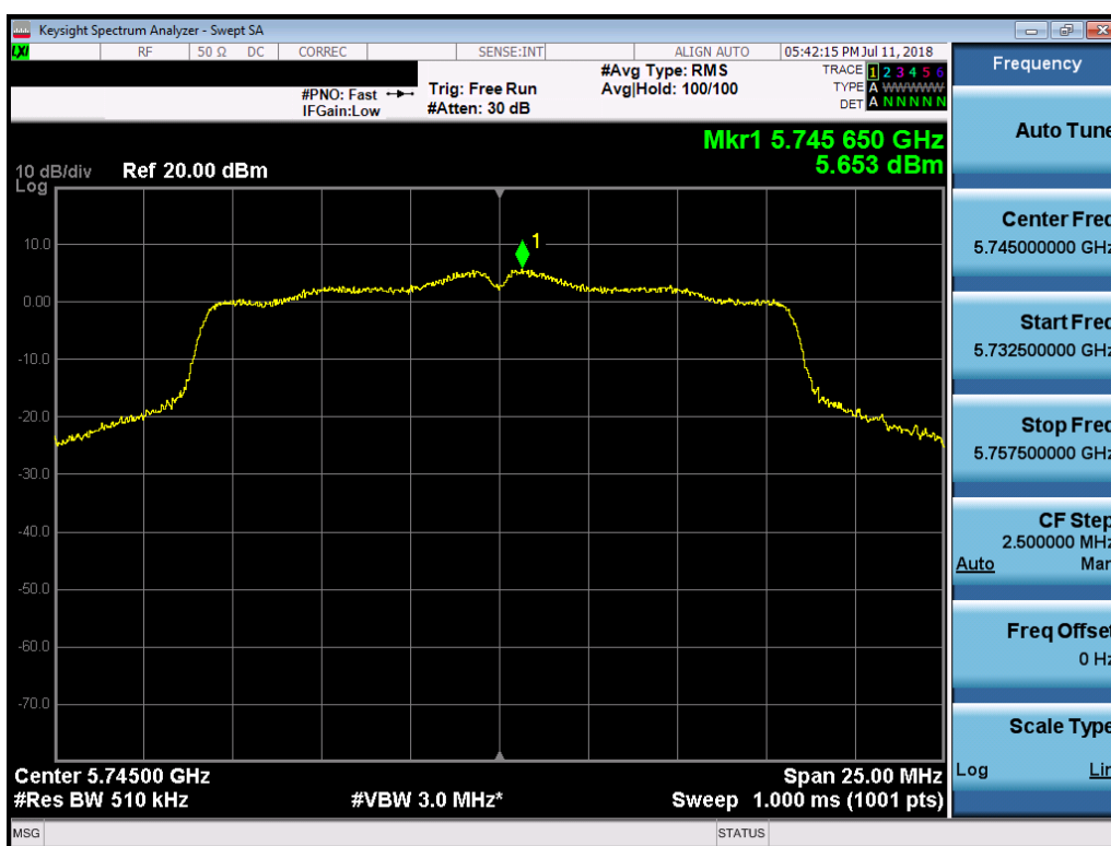
Plot 7-109. Power Spectral Density Plot SISO ANT1 (802.11a (UNII Band 3) – Ch. 149)
