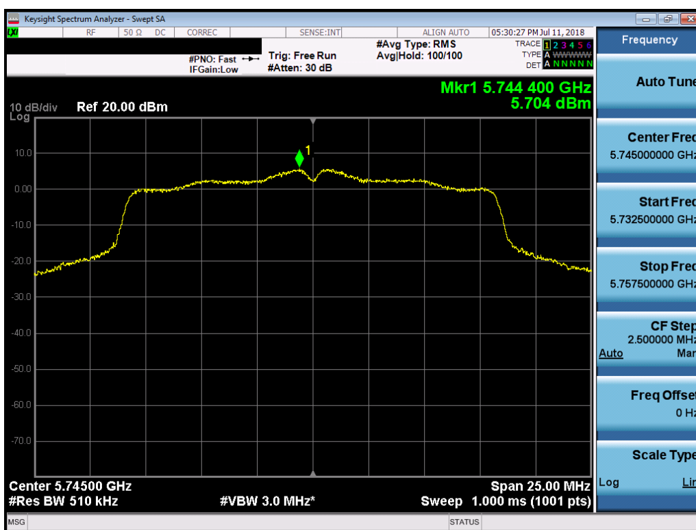
Plot 7-148. Power Spectral Density Plot SISO ANT2 (802.11a) (UNII Band 3) – Ch. 149)
