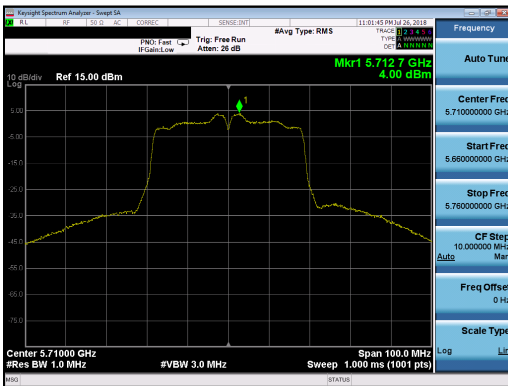
Plot 7-144. Power Spectral Density Plot SISO ANT2 (40MHz BW 802.11n (UNII Band 2C) – Ch. 142)
