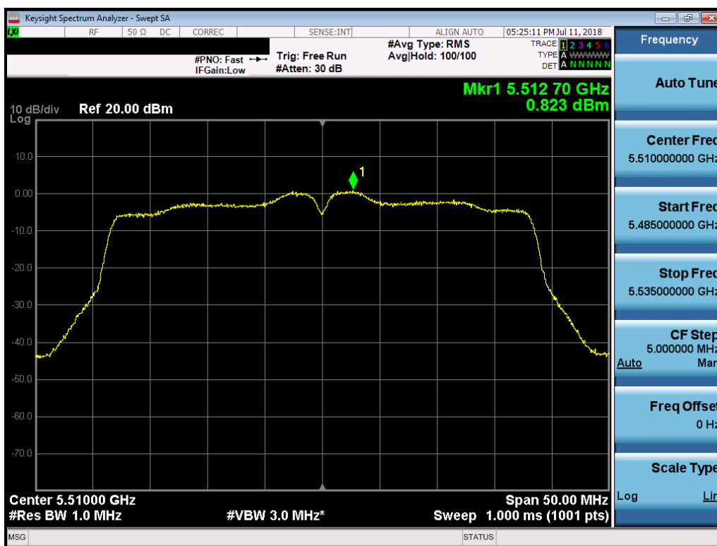
Plot 7-142. Power Spectral Density Plot SISO ANT2 (40MHz BW 802.11n (UNII Band 2C) – Ch. 102)
