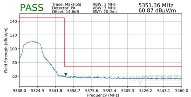
Plot 7-41. Radiated Upper Band Edge Plot SISO ANT2 (Peak – UNII Band 2A)
