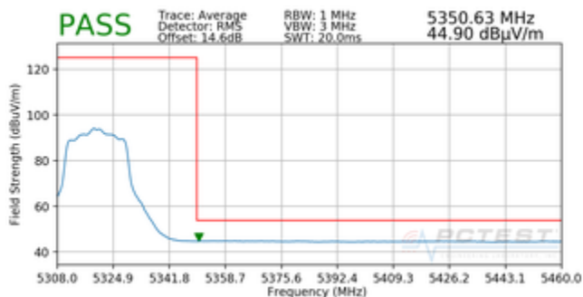
Plot 7-19. Radiated Upper Band Edge Plot SISO ANT1 (Average – UNII Band 2A)
