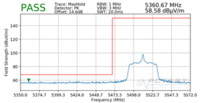
Plot 7-36. Radiated Lower Band Edge Plot SISO ANT1 (Peak – UNII Band 2C)
