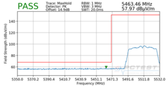
Plot 7-29. Radiated Lower Band Edge Plot SISO ANT1 (Peak – UNII Band 2C)
