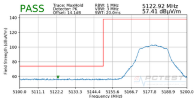
Plot 7-18. Radiated Lower Band Edge Plot SISO ANT1 (Peak – UNII Band 1)
