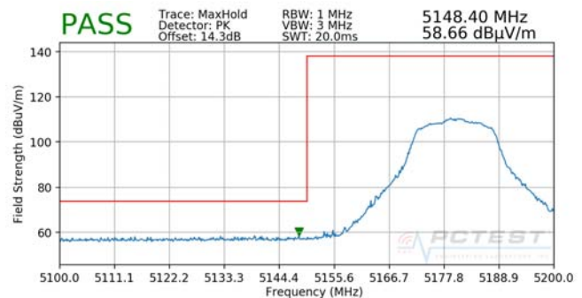
Plot 7-39. Radiated Lower Band Edge Plot SISO ANT2 (Peak – UNII Band 1)
